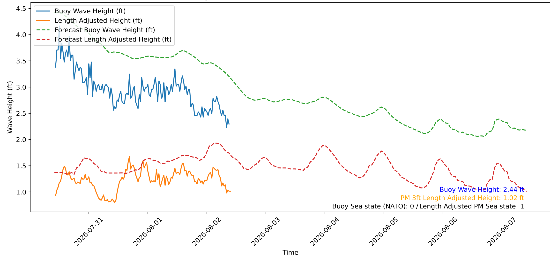
Wave Heights over Time for Red Beach at 2026-08-02 10:10:46
