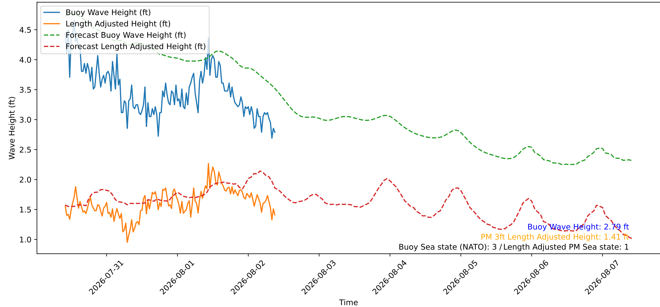
Wave Heights over Time for Oceanside Harbor at 2026-08-02 10:10:26
