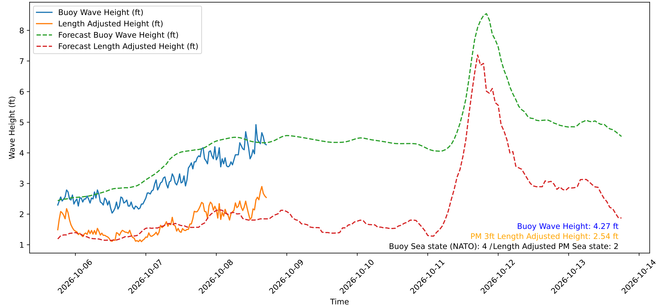
Wave Heights over Time for Oceanside Harbor at 2026-10-08 18:00:29
