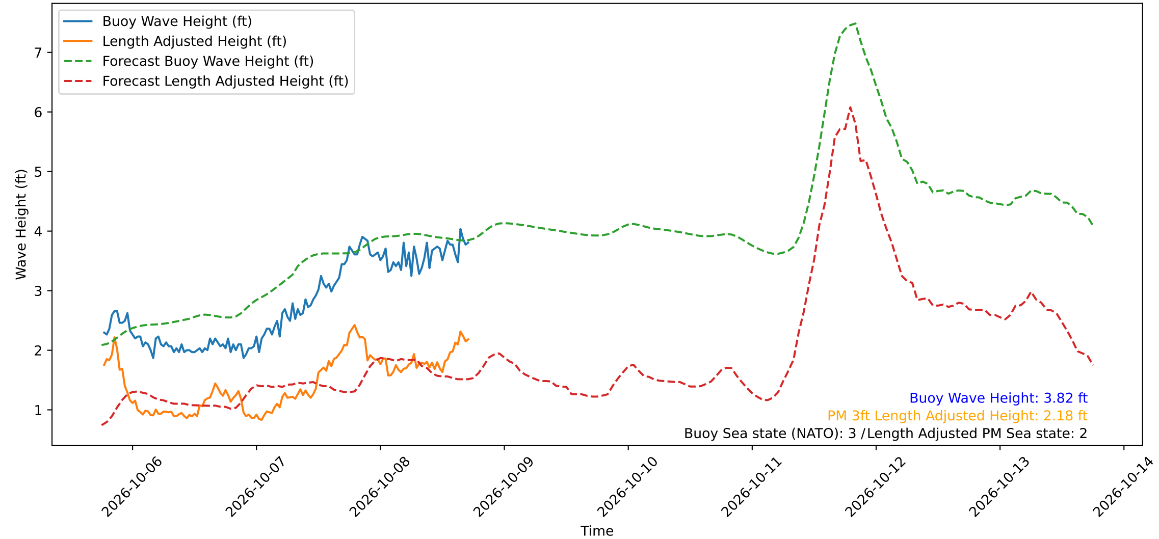
Wave Heights over Time for Red Beach at 2026-10-08 18:00:49
