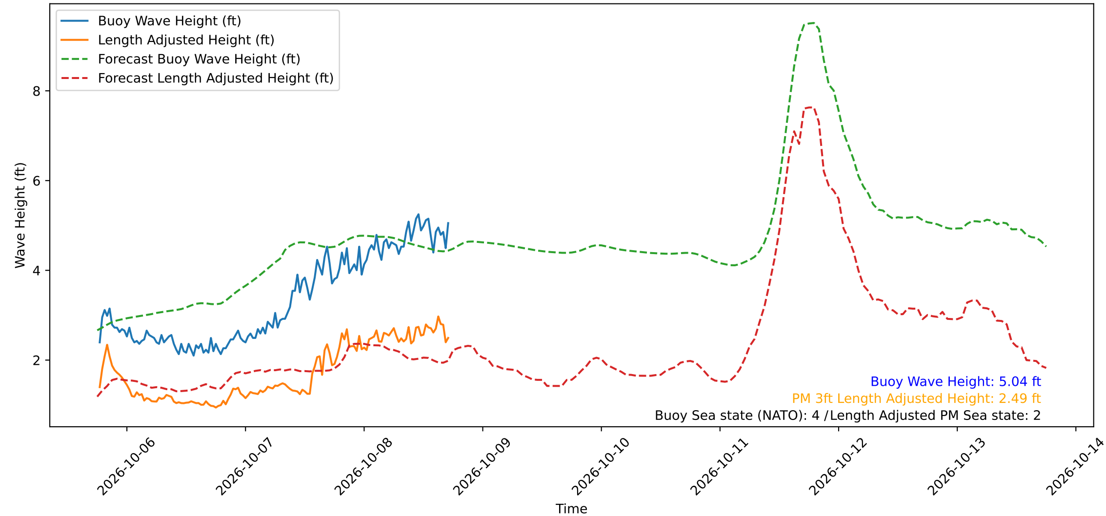
Wave Heights over Time for Green Beach at 2026-10-08 18:01:12
