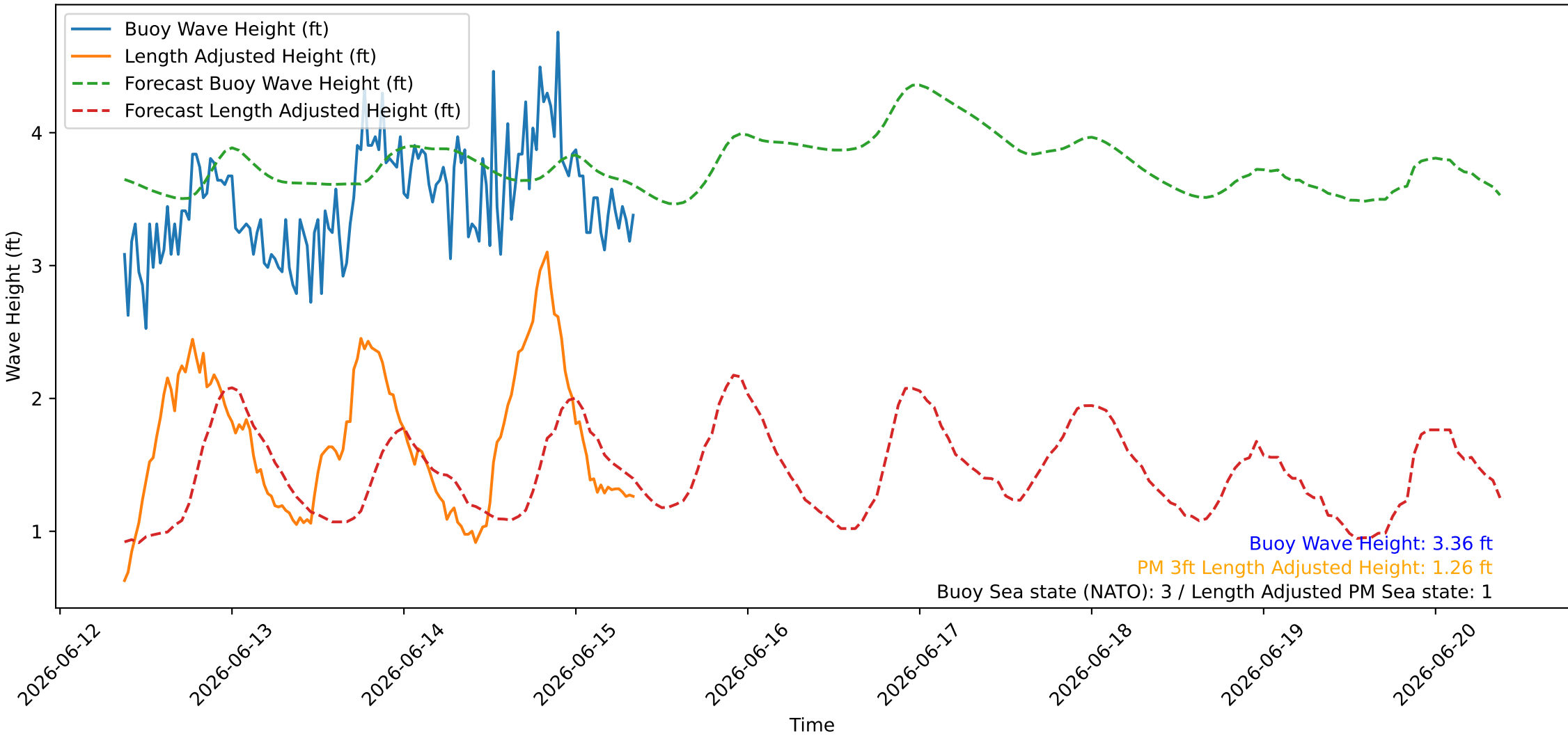
Wave Heights over Time for Red Beach at 2026-06-15 08:40:46
