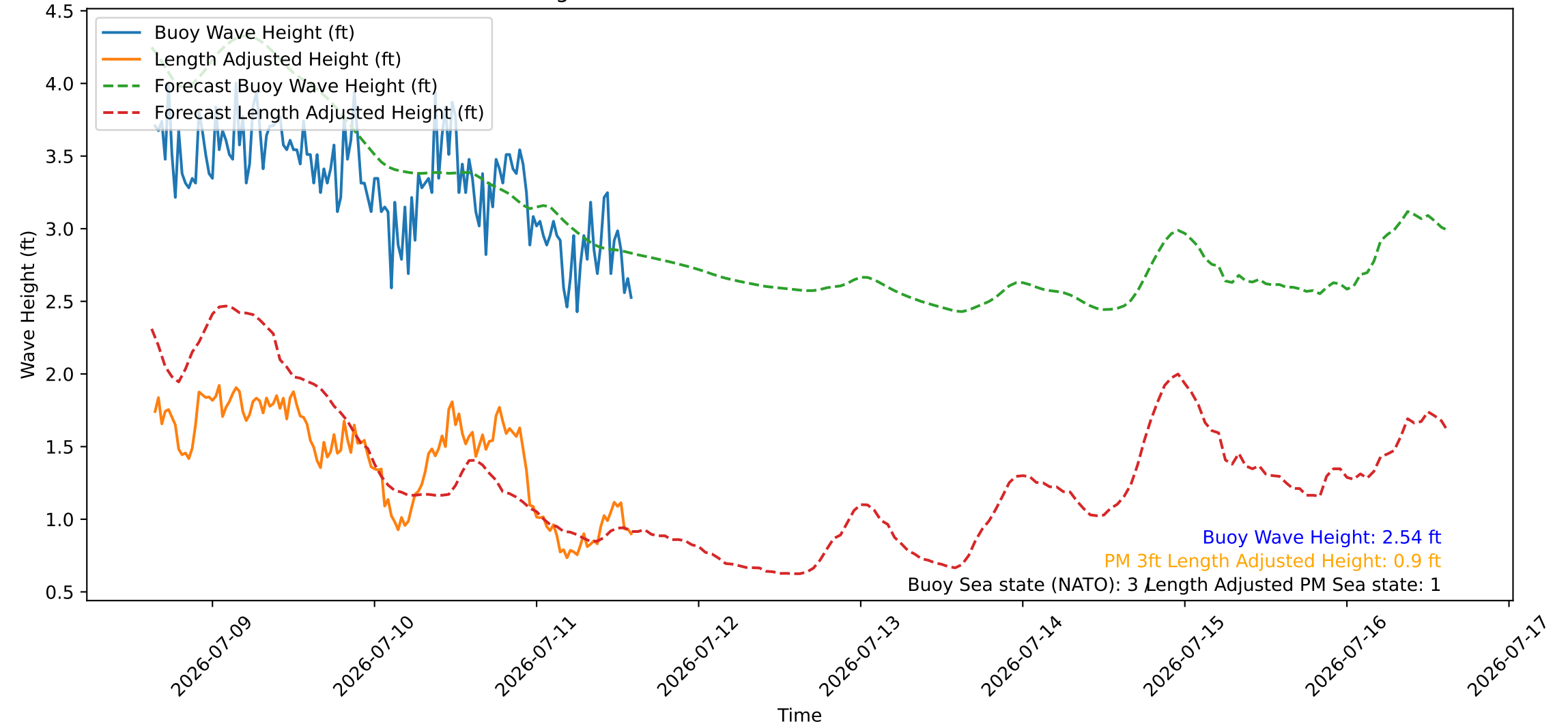
Wave Heights over Time for Red Beach at 2026-07-11 15:10:46
