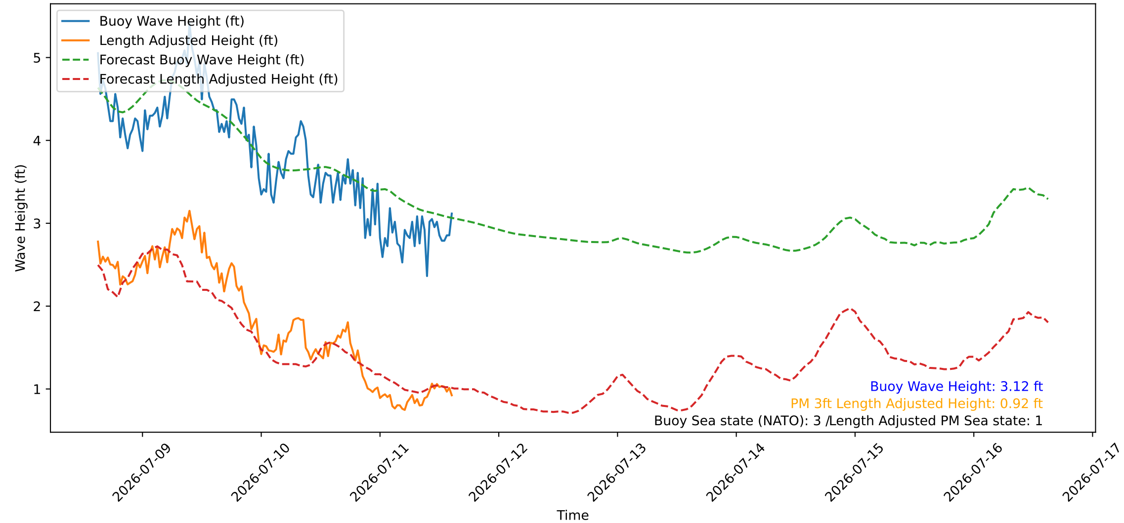
Wave Heights over Time for Oceanside Harbor at 2026-07-11 15:10:26
