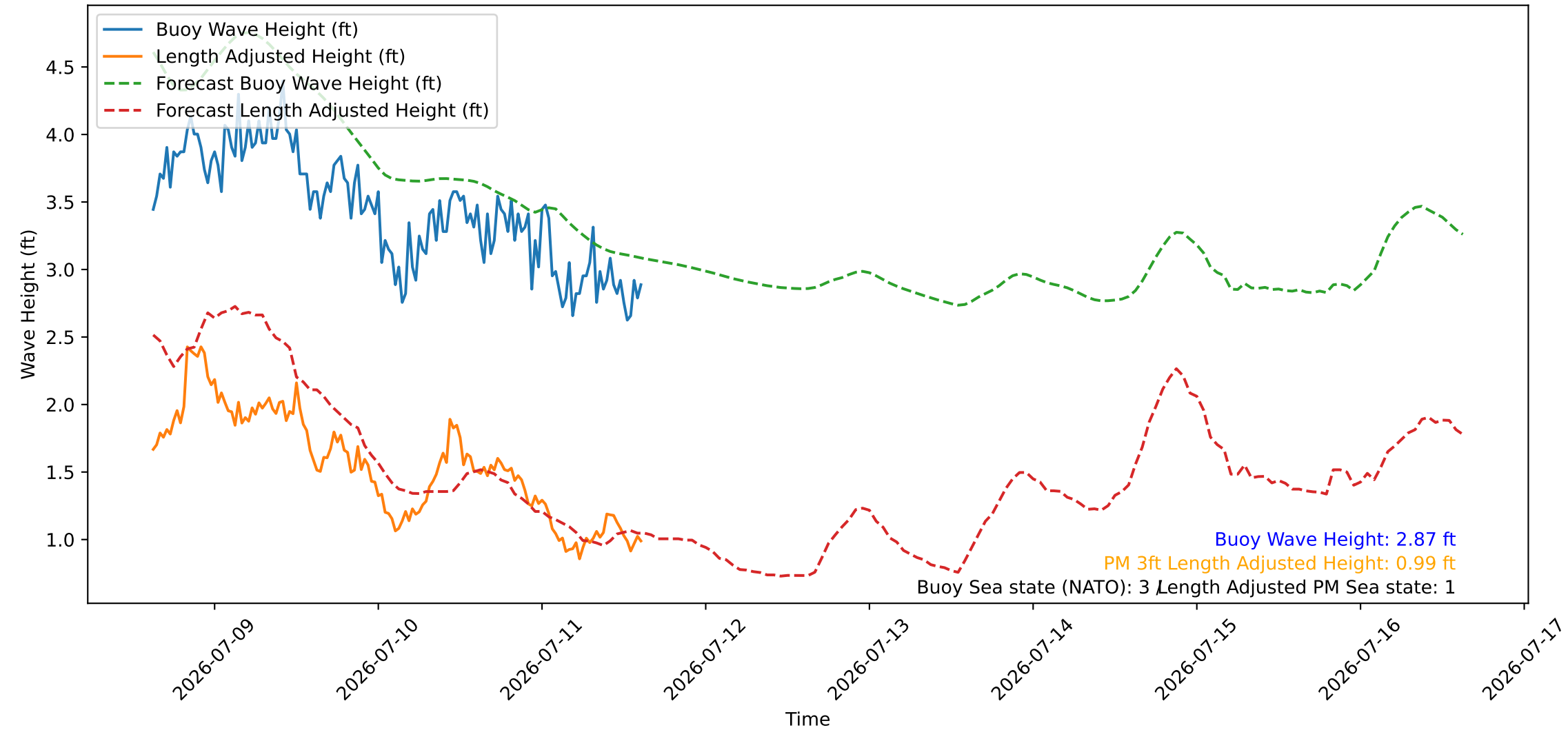
Wave Heights over Time for Green Beach at 2026-07-11 15:11:08
