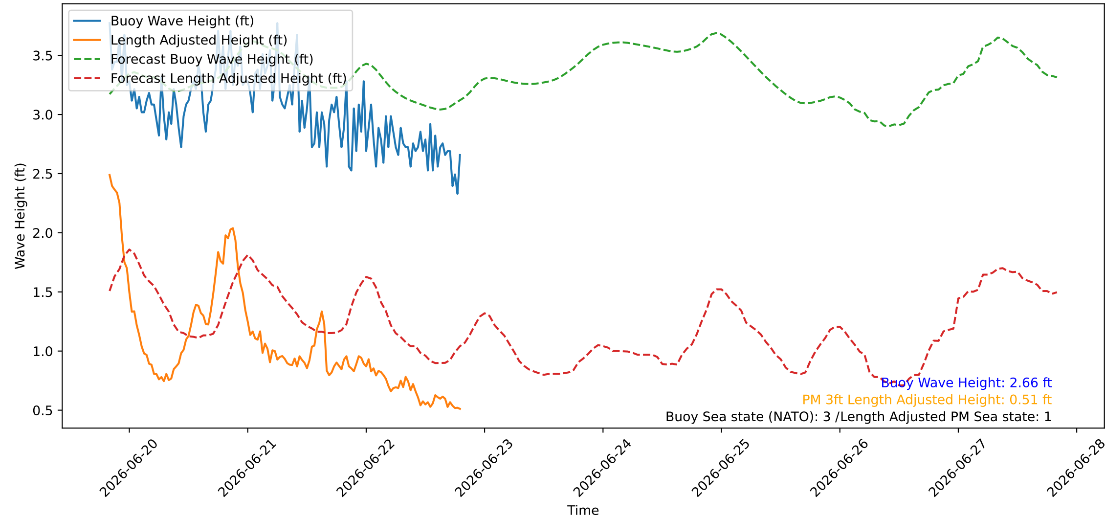
Wave Heights over Time for Red Beach at 2026-06-22 19:40:46
