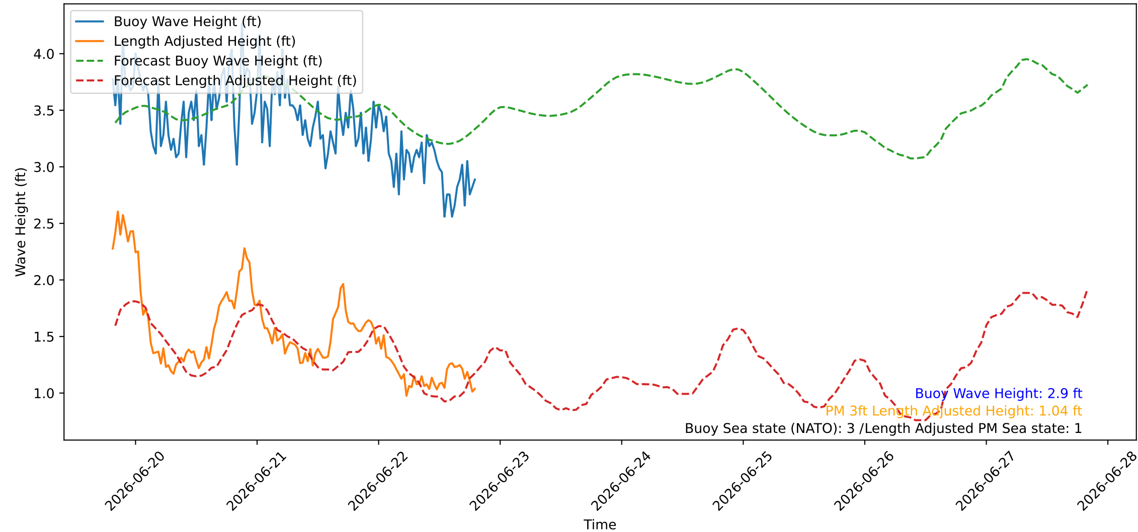
Wave Heights over Time for Oceanside Harbor at 2026-06-22 19:40:26
