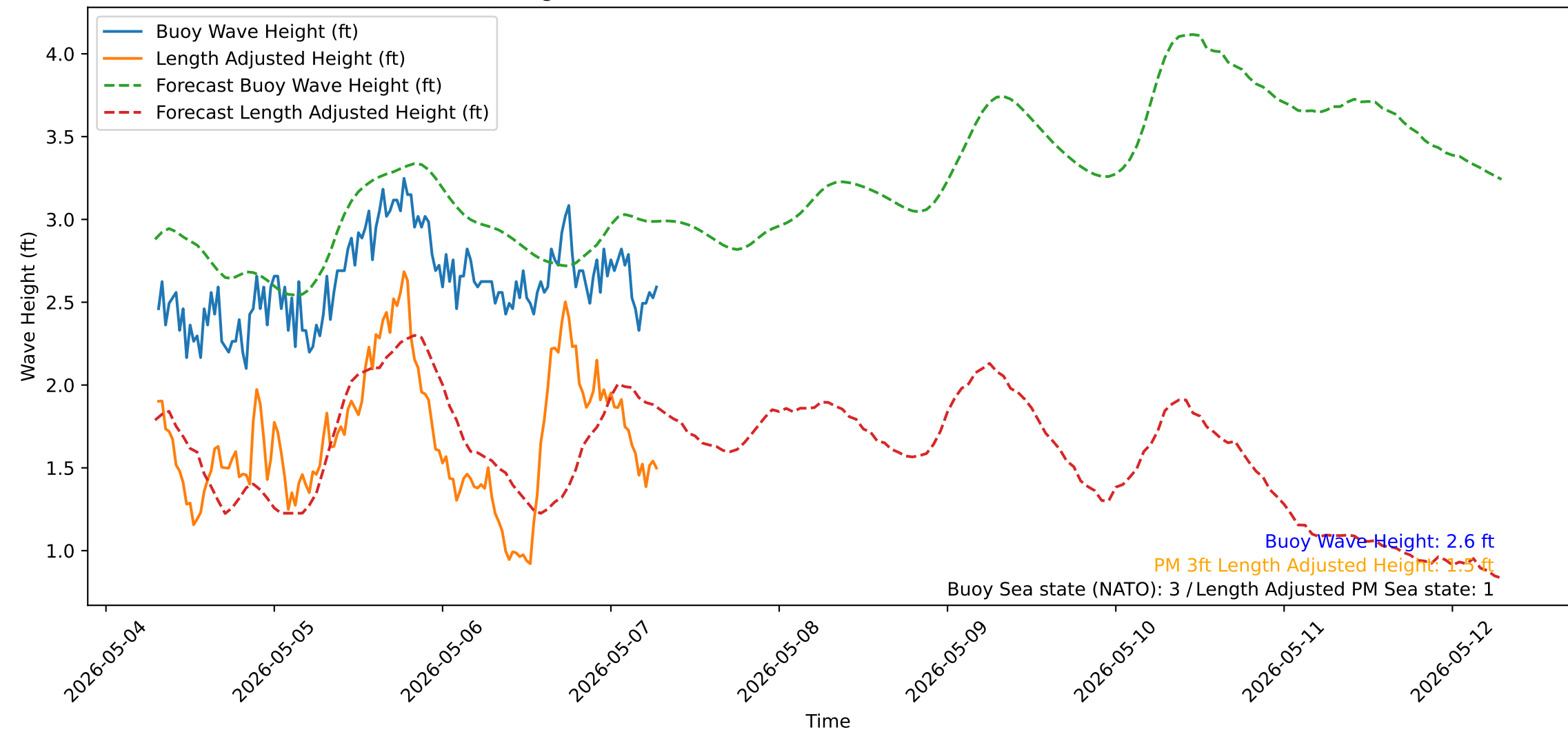
Wave Heights over Time for Oceanside Harbor at 2026-05-07 07:20:31
