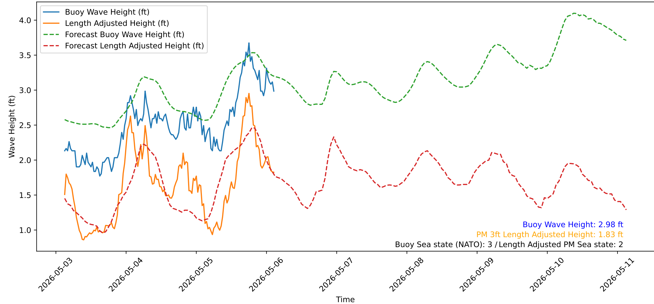
Wave Heights over Time for Green Beach at 2026-05-06 03:11:12
