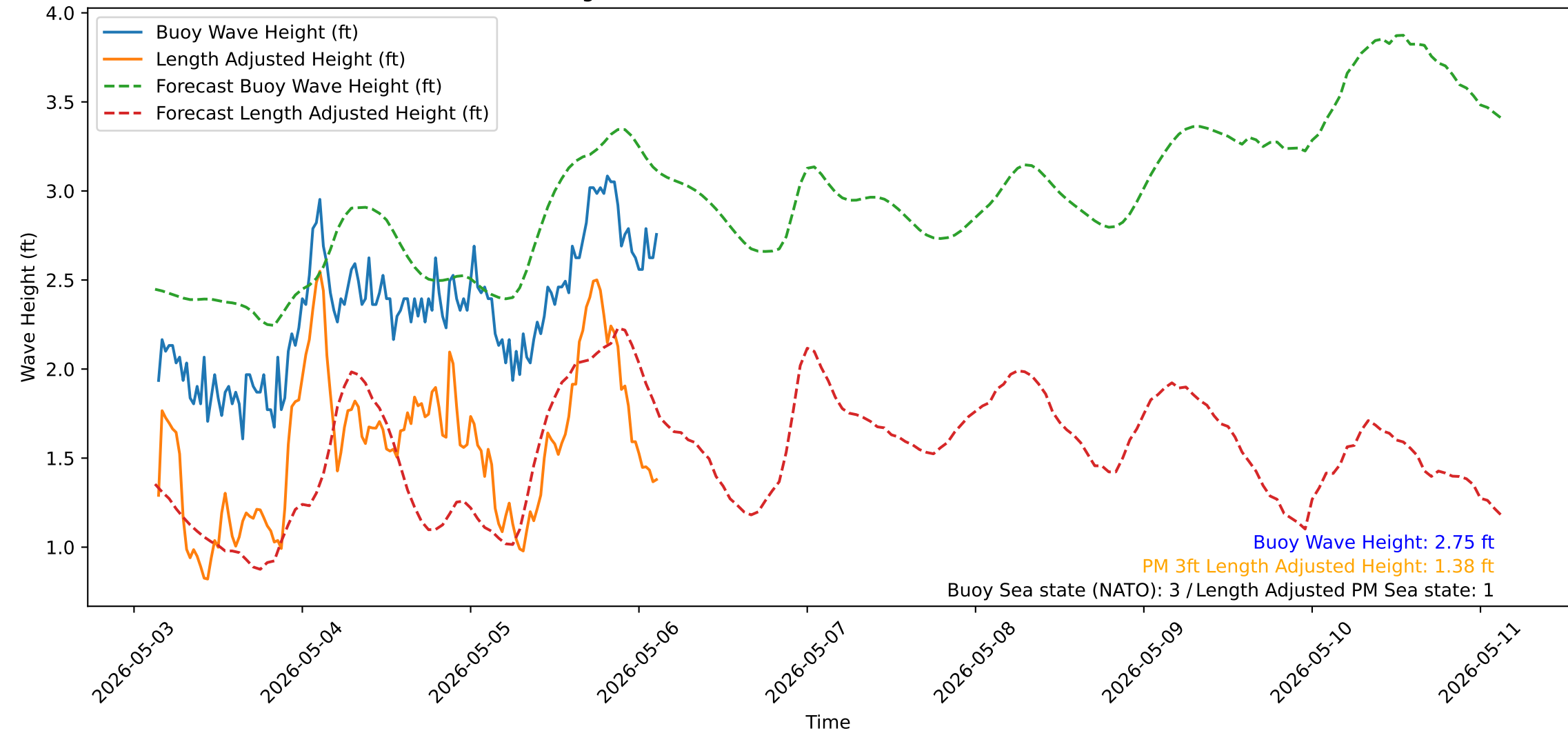
Wave Heights over Time for Red Beach at 2026-05-06 03:10:50
