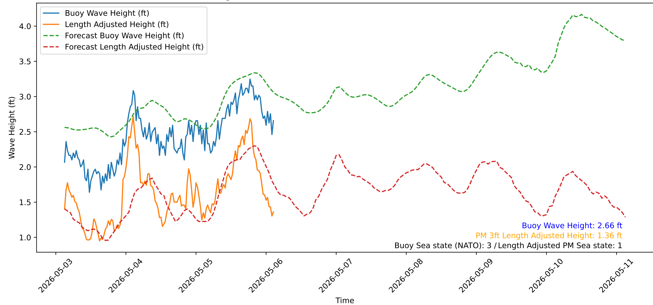
Wave Heights over Time for Oceanside Harbor at 2026-05-06 03:10:31
