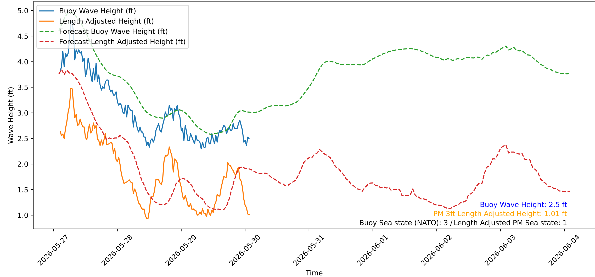
Wave Heights over Time for Red Beach at 2026-05-30 02:20:43
