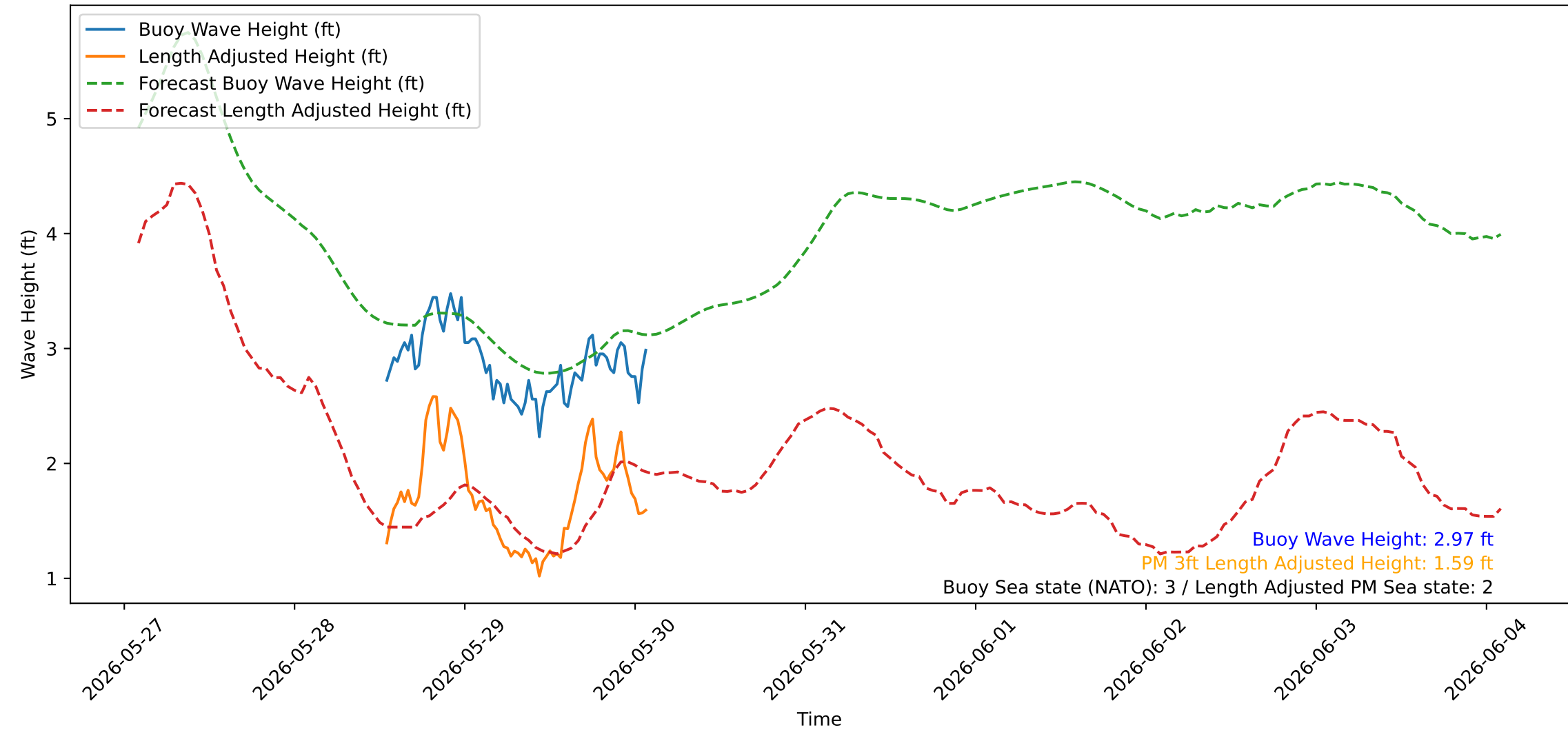
Wave Heights over Time for Oceanside Harbor at 2026-05-30 02:20:22
