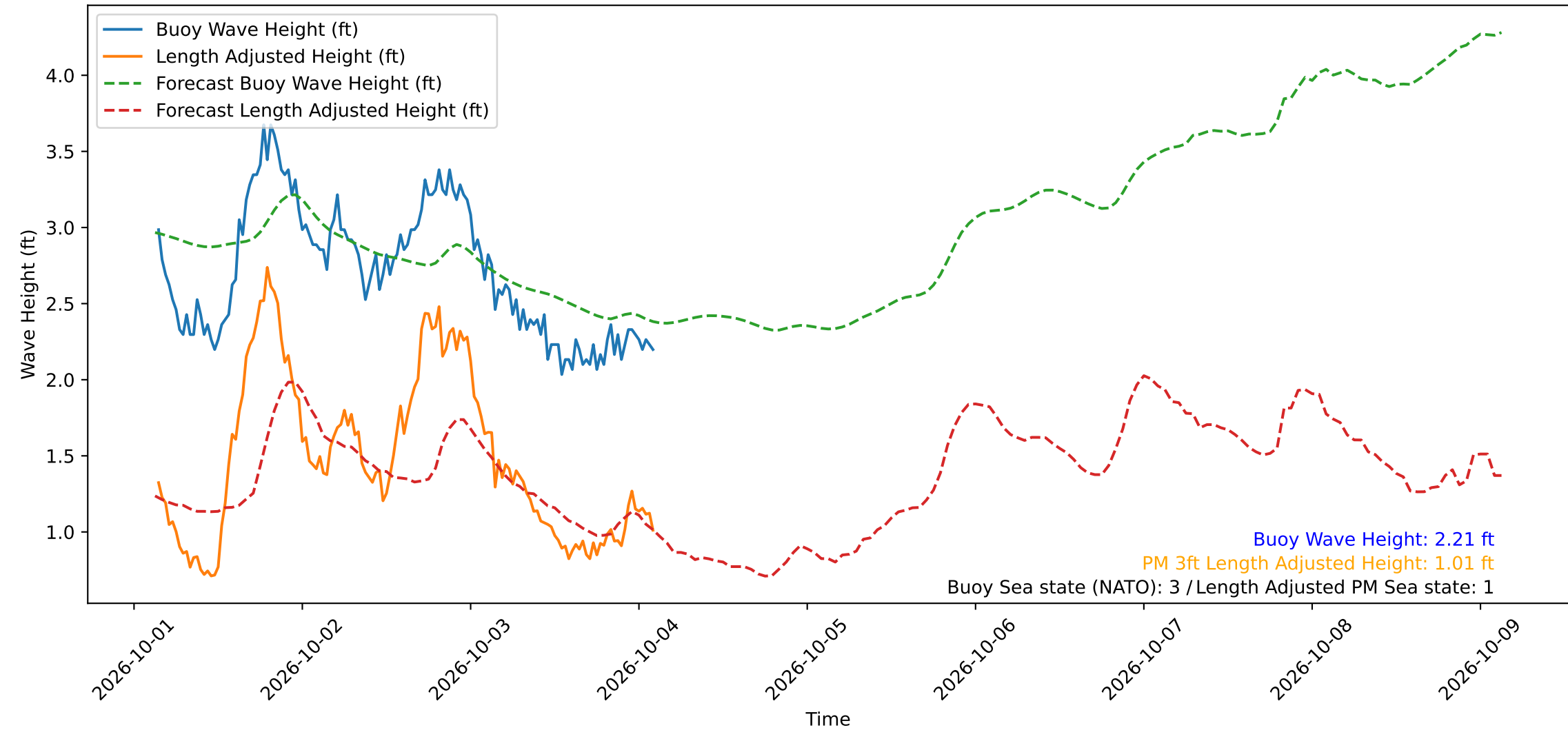
Wave Heights over Time for Green Beach at 2026-10-04 03:01:11
