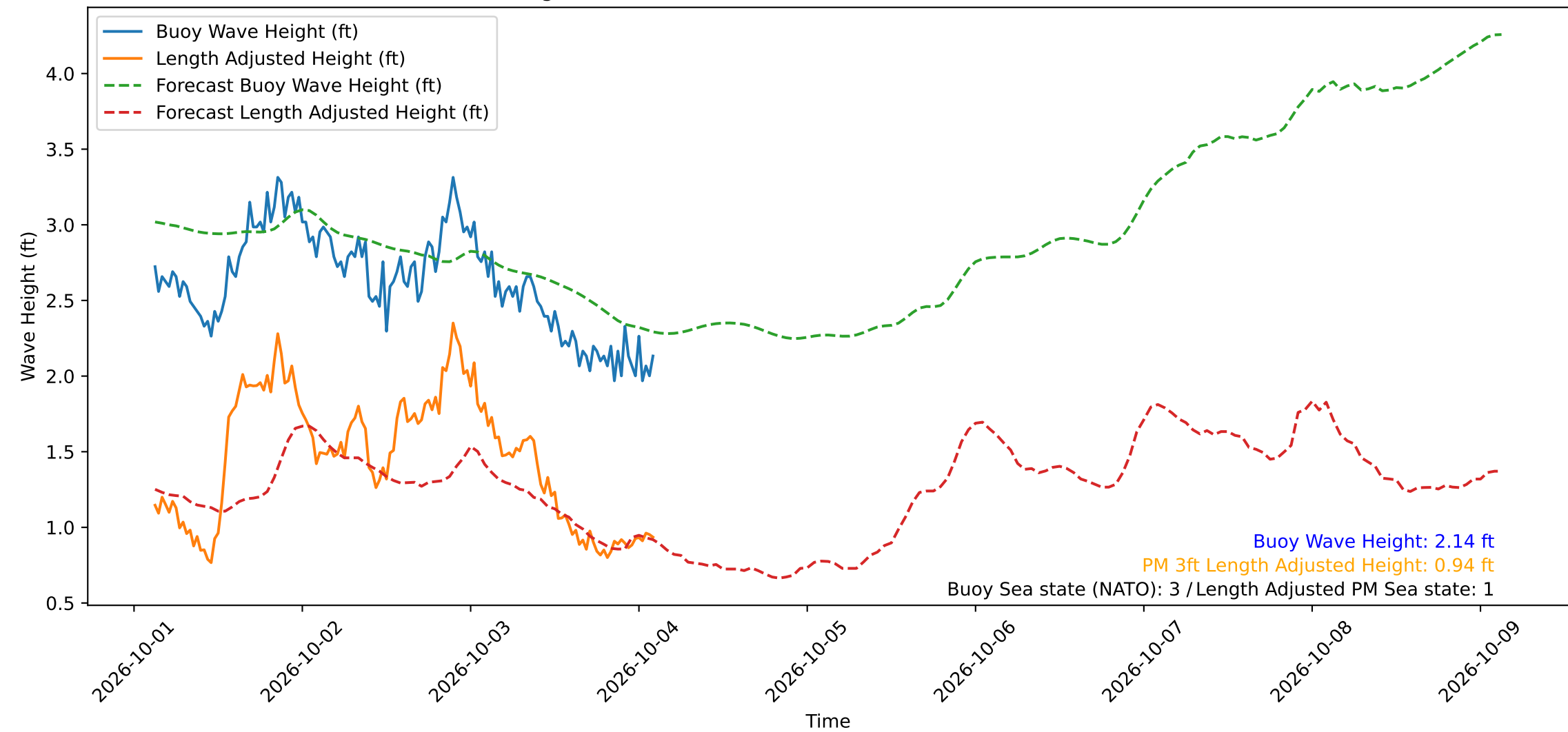
Wave Heights over Time for Oceanside Harbor at 2026-10-04 03:00:30
