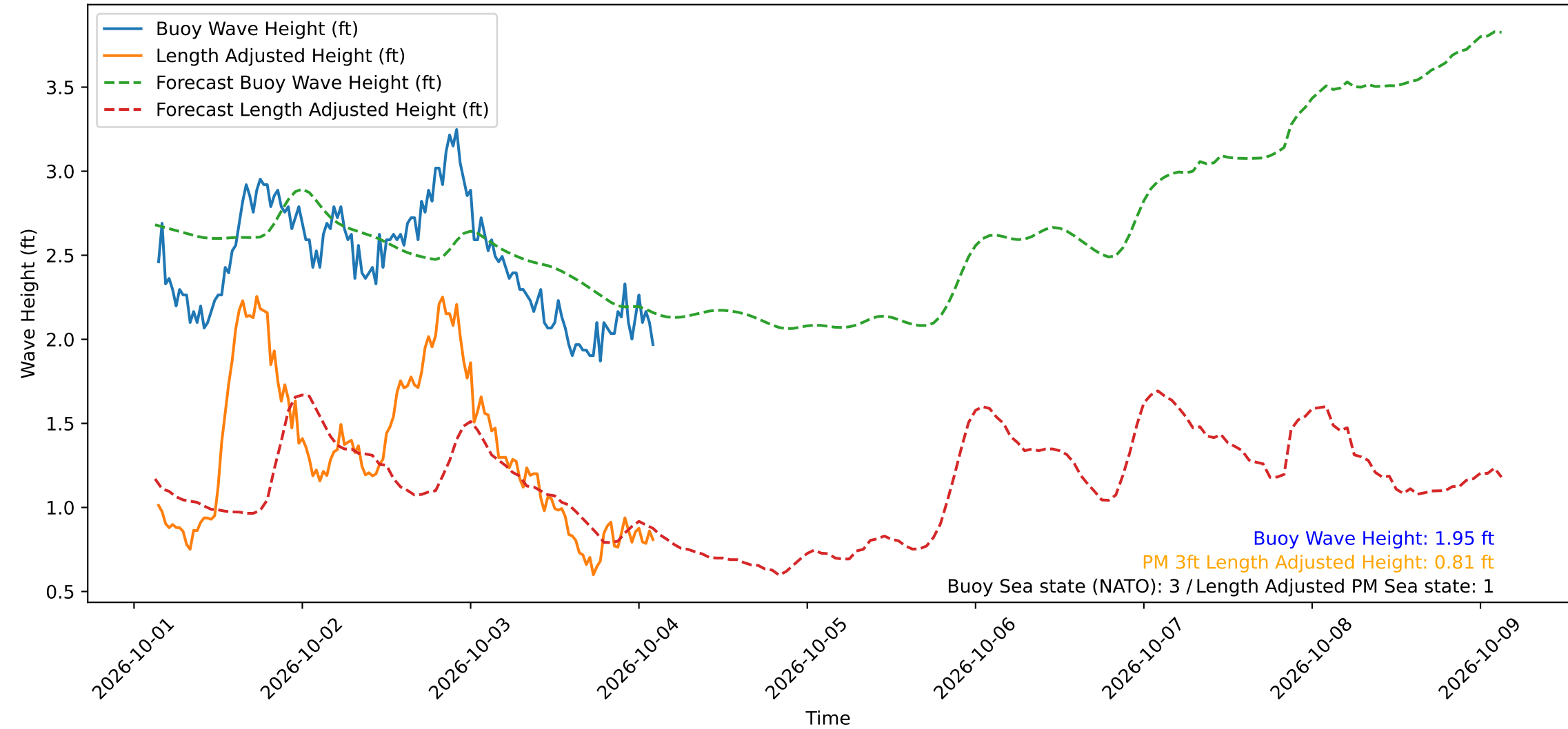
Wave Heights over Time for Red Beach at 2026-10-04 03:00:49
