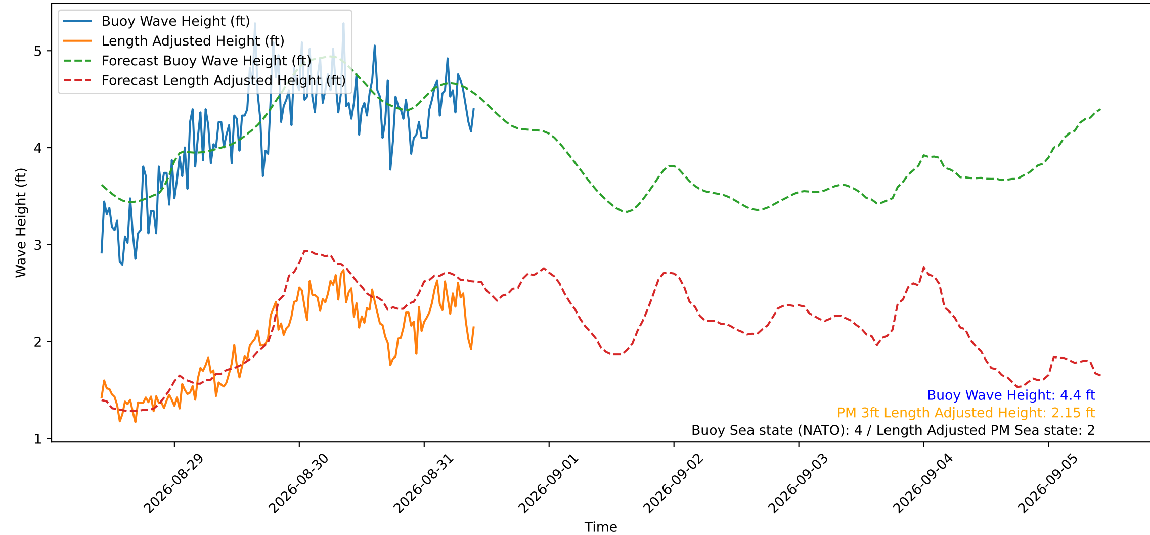
Wave Heights over Time for Oceanside Harbor at 2026-08-31 10:10:29
