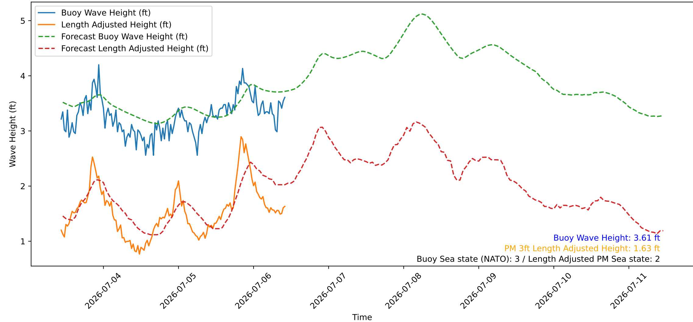
Wave Heights over Time for Green Beach at 2026-07-06 10:41:10
