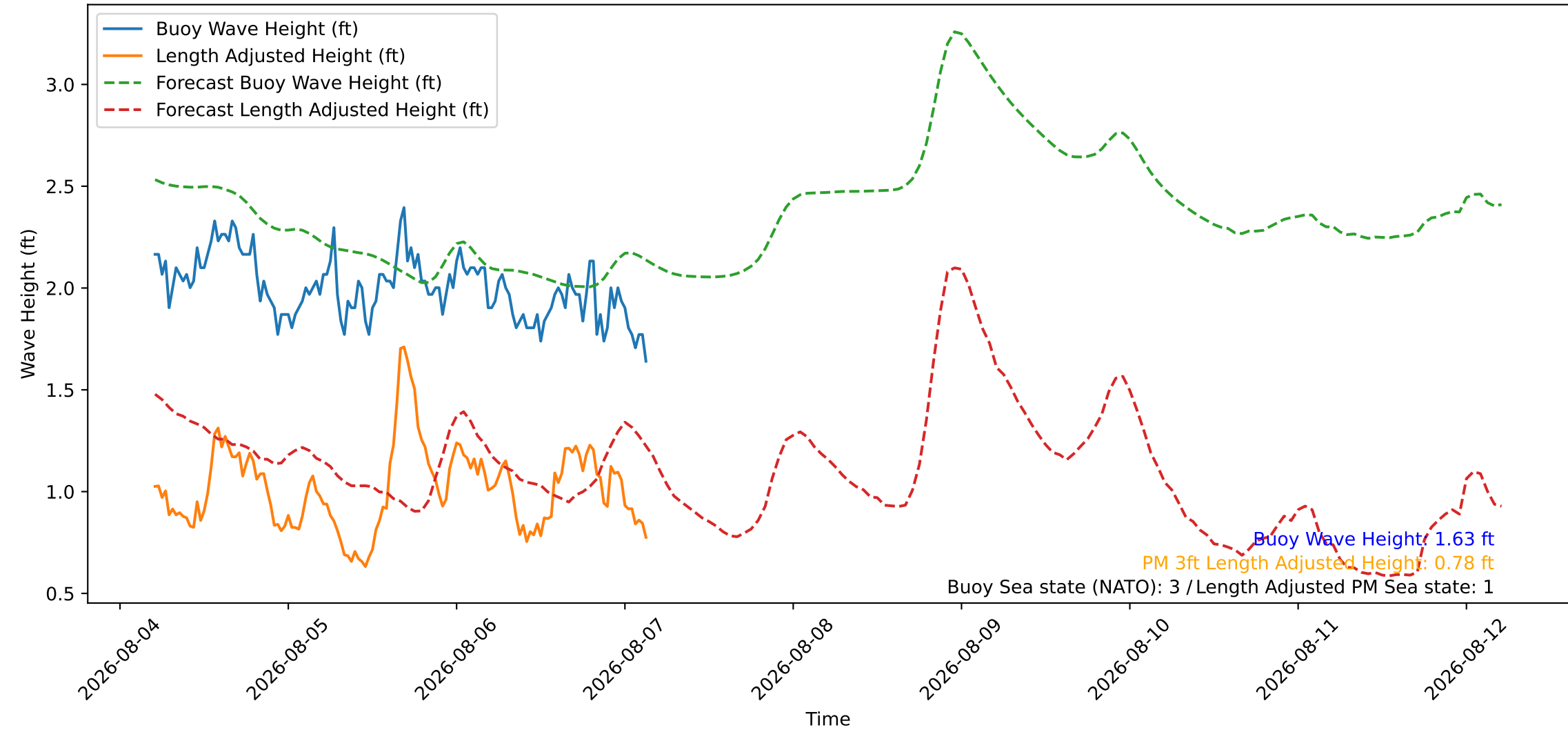
Wave Heights over Time for Red Beach at 2026-08-07 04:30:45
