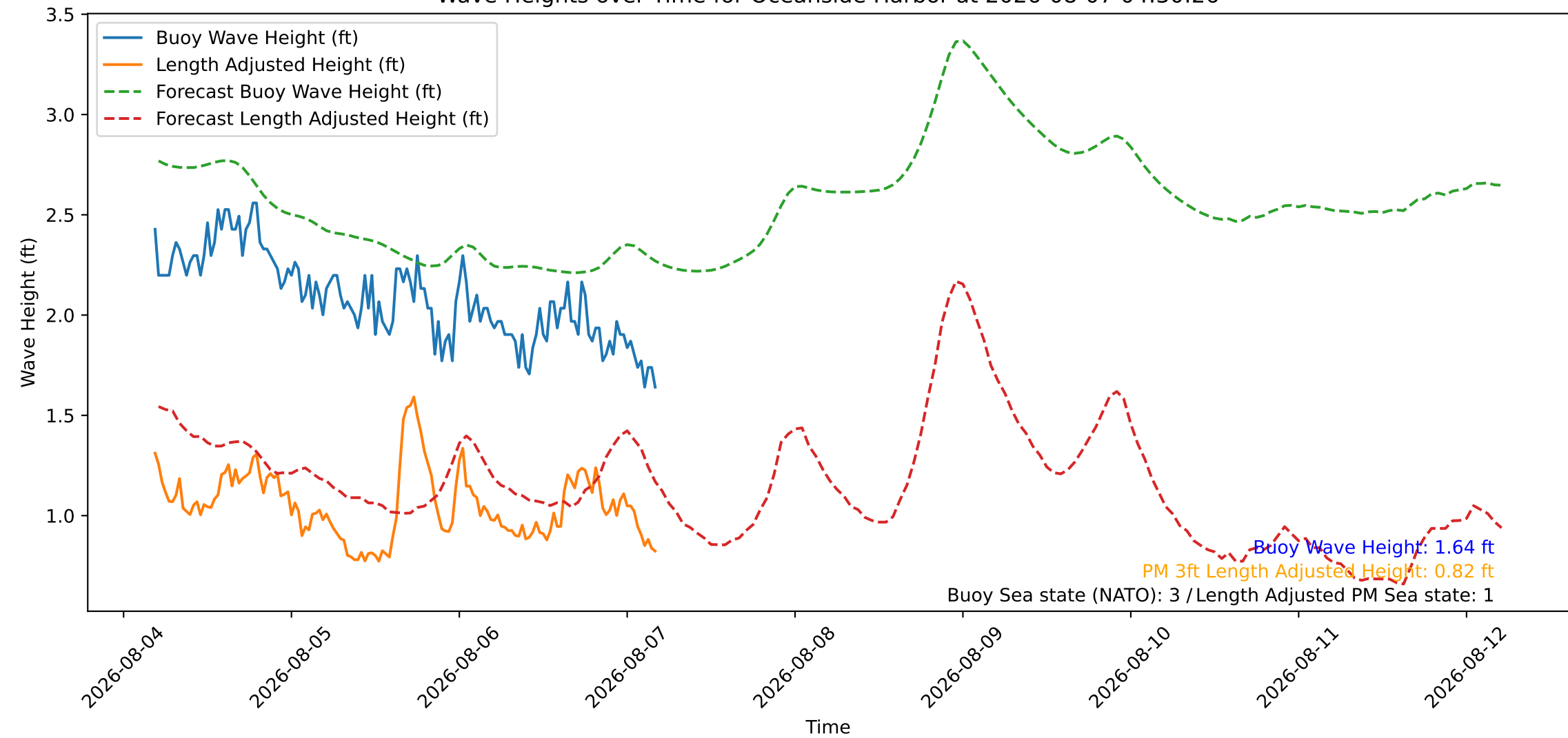
Wave Heights over Time for Oceanside Harbor at 2026-08-07 04:30:26
