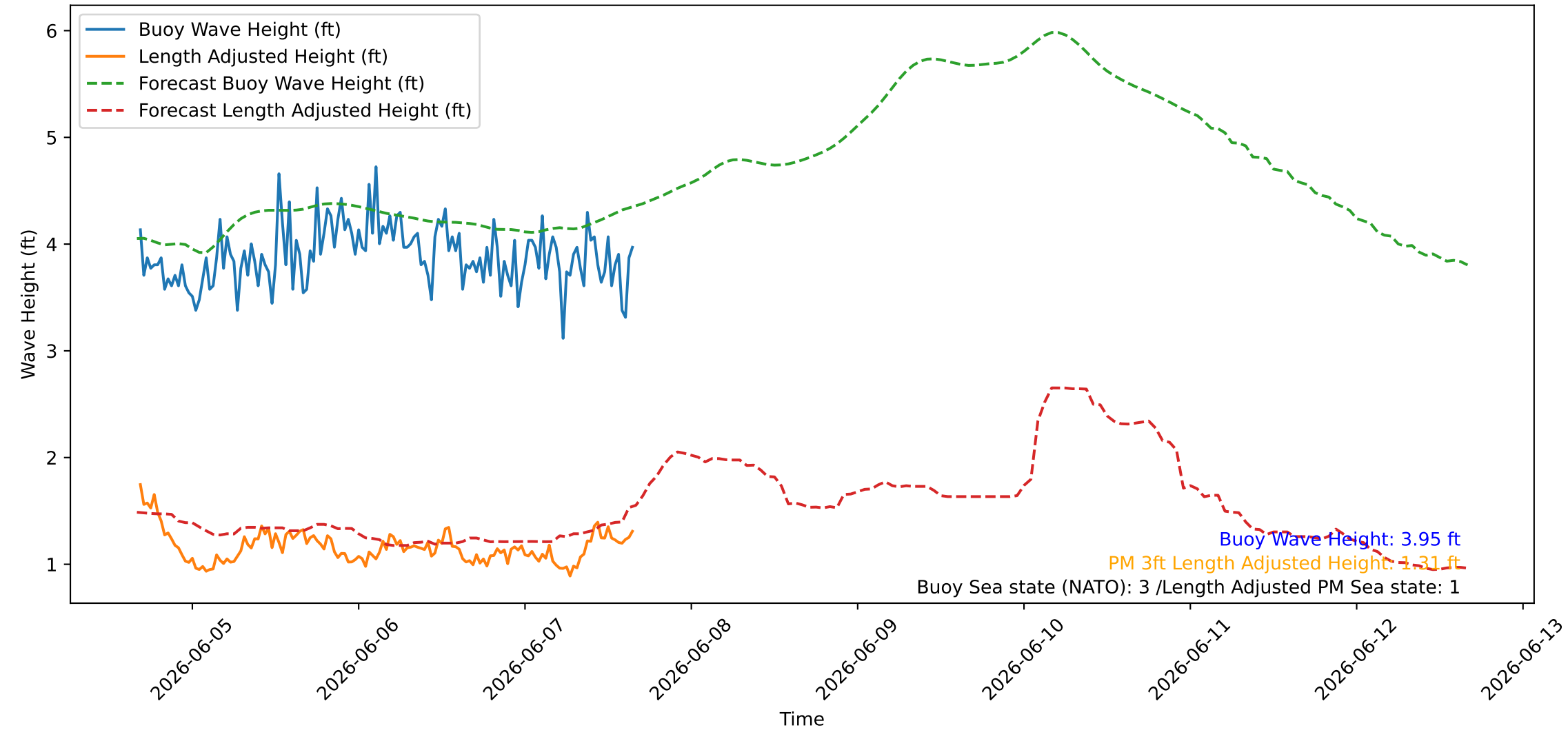
Wave Heights over Time for Green Beach at 2026-06-07 16:21:09
