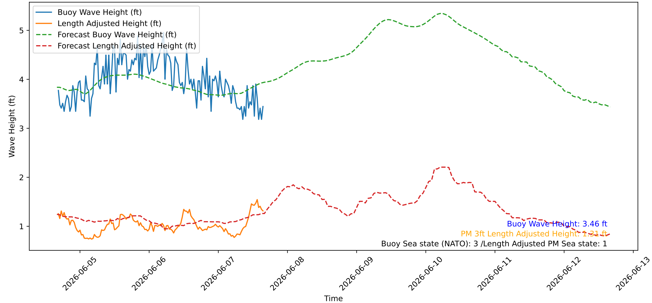
Wave Heights over Time for Red Beach at 2026-06-07 16:20:47
