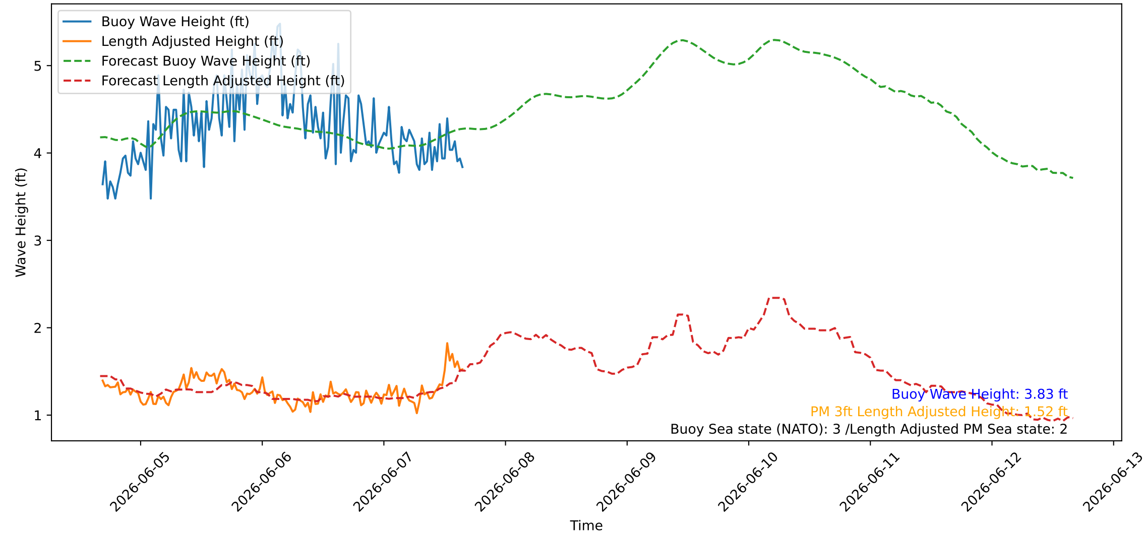
Wave Heights over Time for Oceanside Harbor at 2026-06-07 16:20:26
