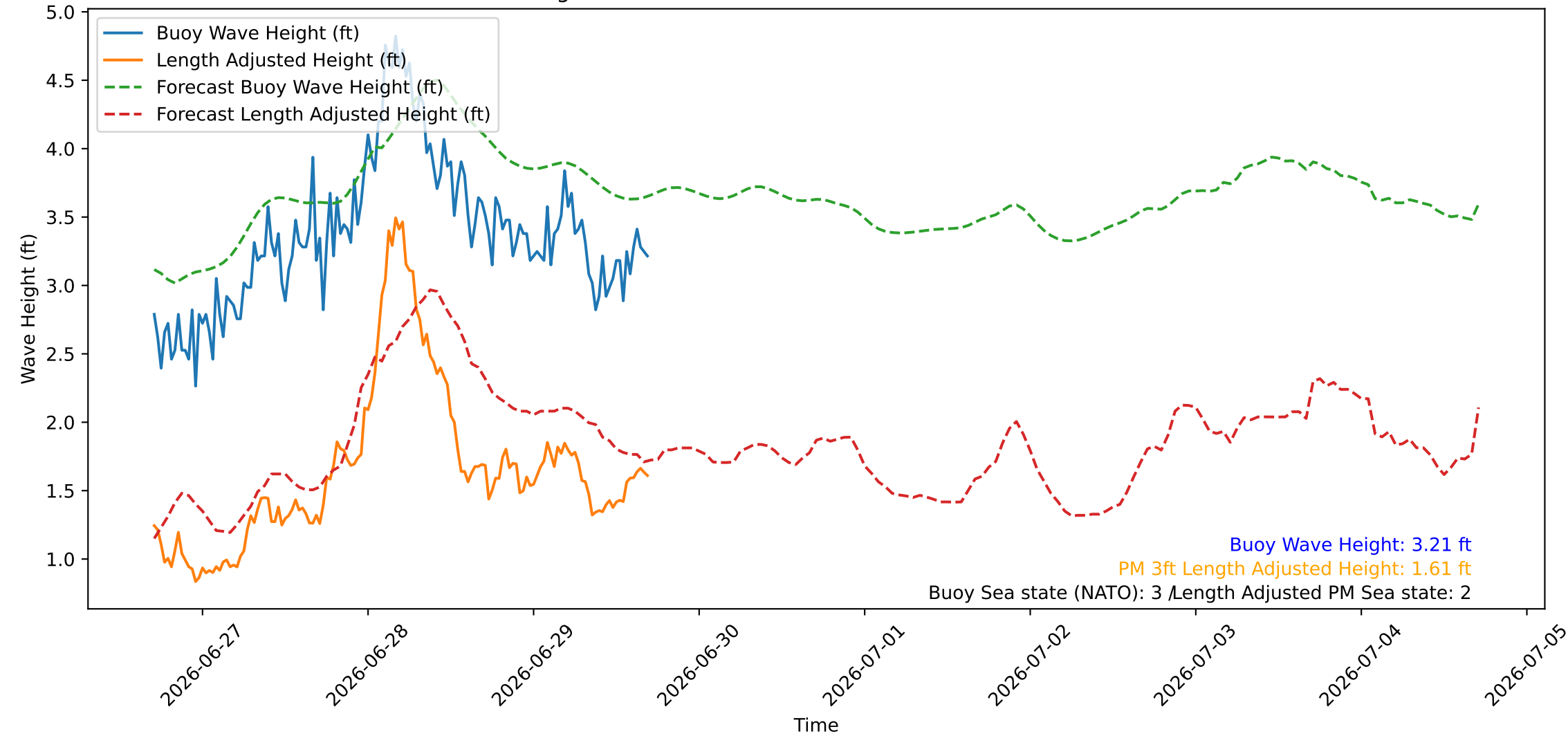
Wave Heights over Time for Green Beach at 2026-06-29 17:11:07
