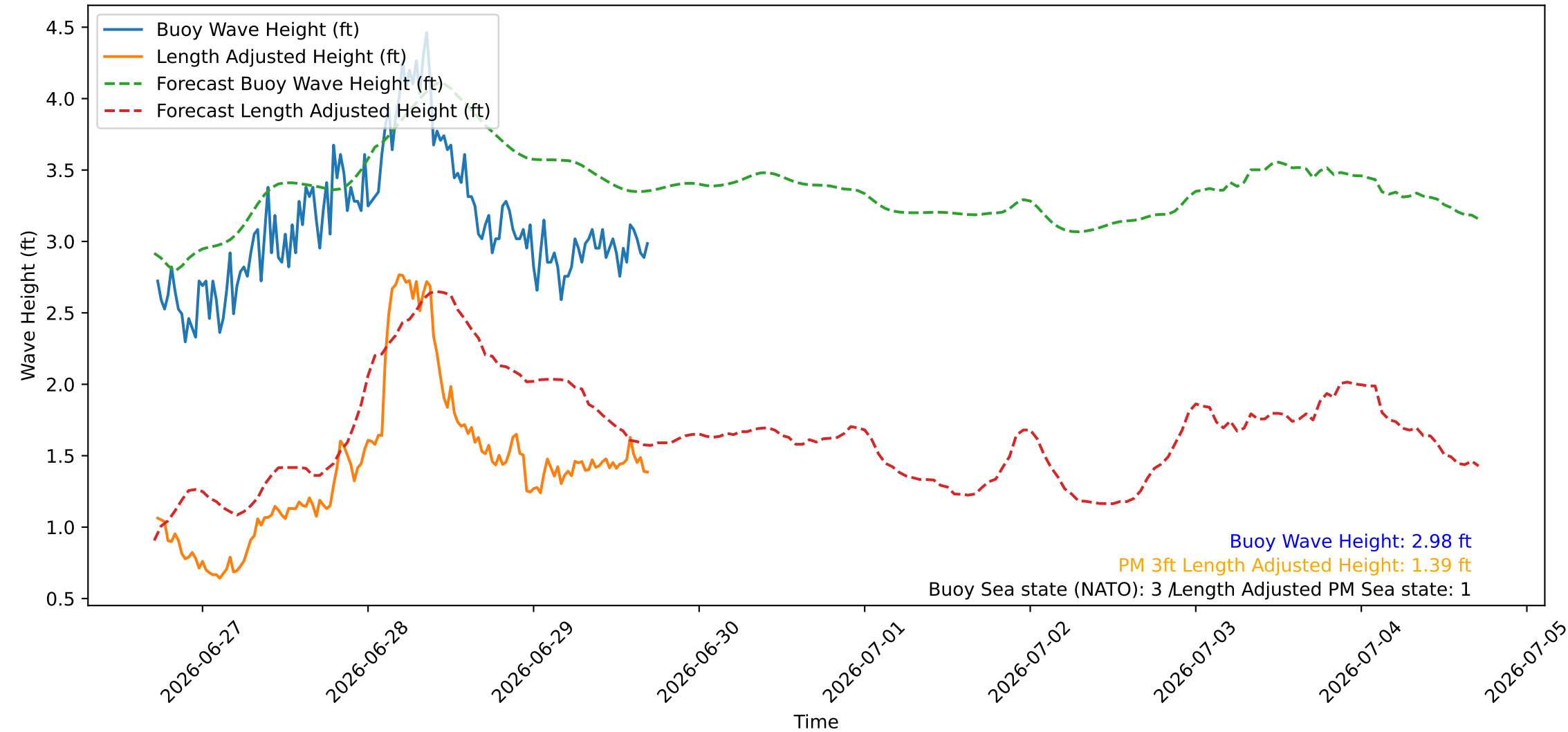
Wave Heights over Time for Red Beach at 2026-06-29 17:10:45
