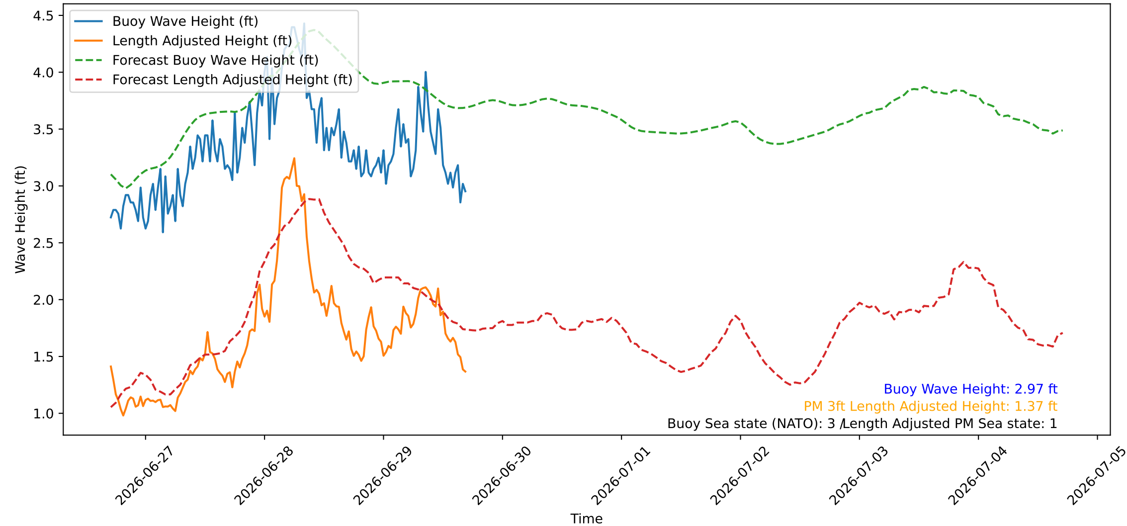
Wave Heights over Time for Oceanside Harbor at 2026-06-29 17:10:26
