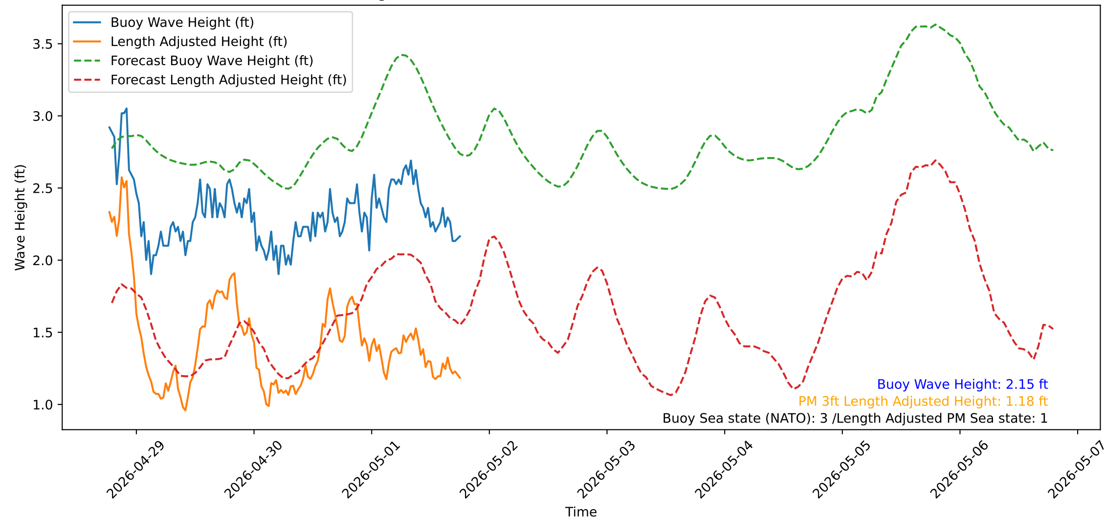
Wave Heights over Time for Oceanside Harbor at 2026-05-01 18:40:31
