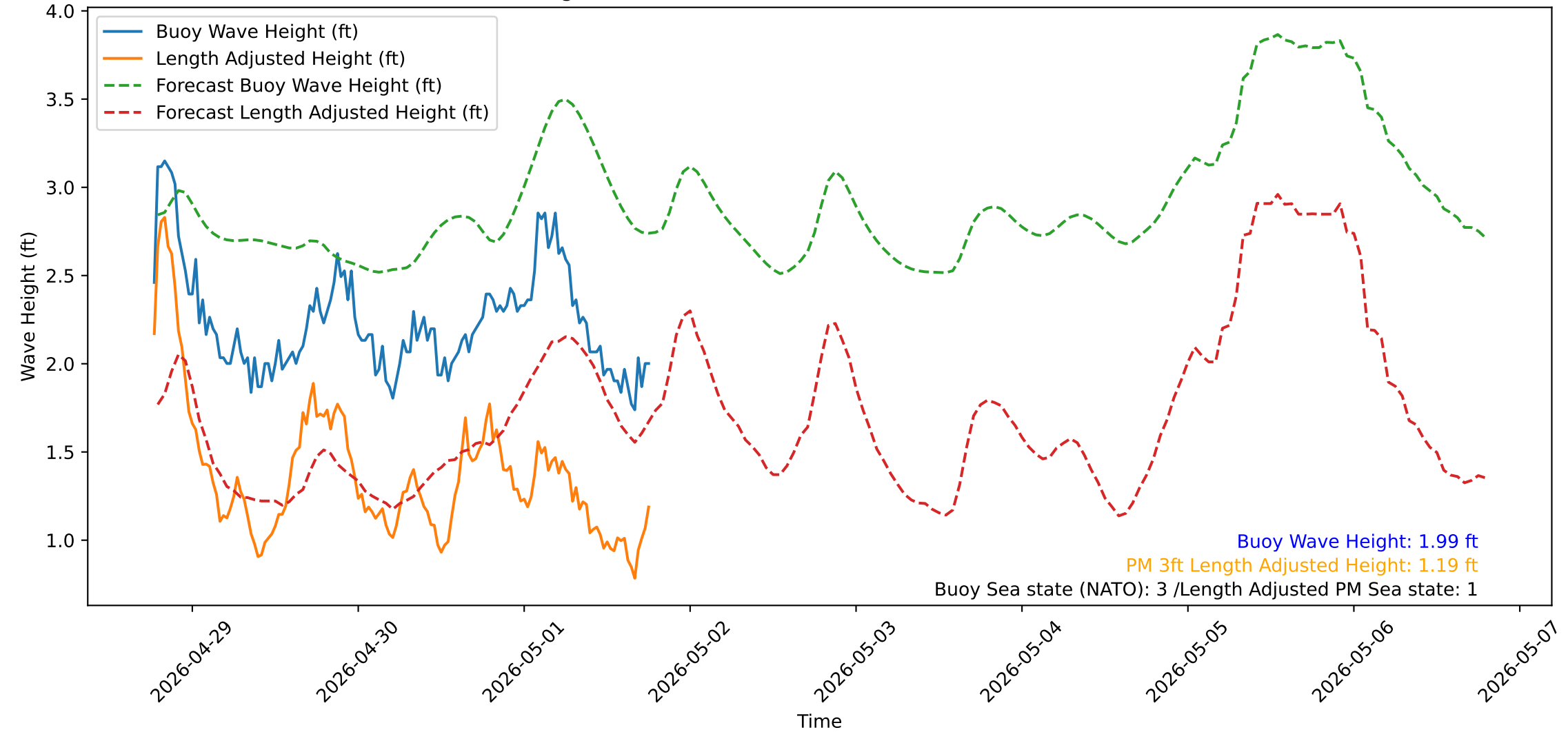
Wave Heights over Time for Green Beach at 2026-05-01 18:41:14
