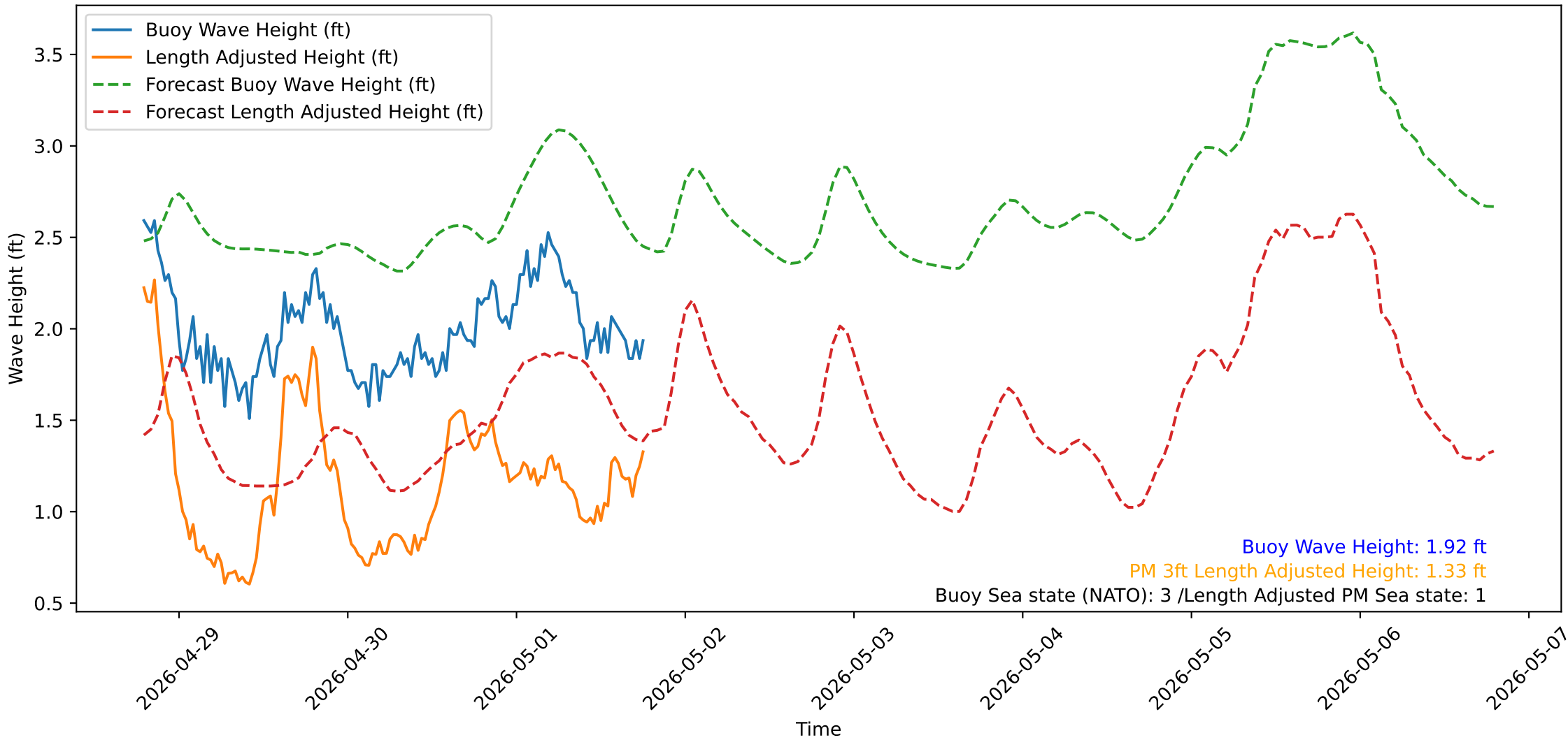
Wave Heights over Time for Red Beach at 2026-05-01 18:40:52
