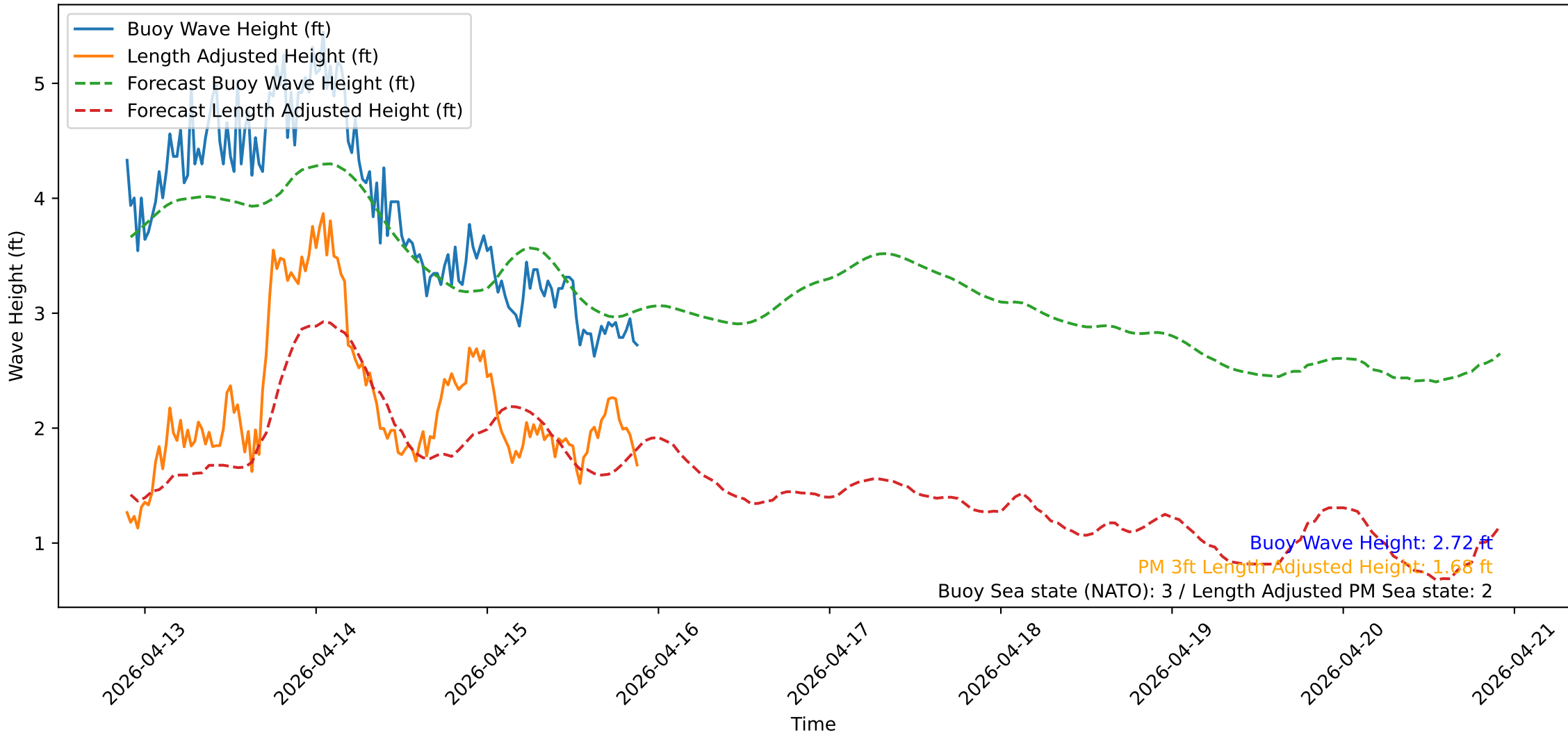
Wave Heights over Time for Oceanside Harbor at 2026-04-15 21:40:32
