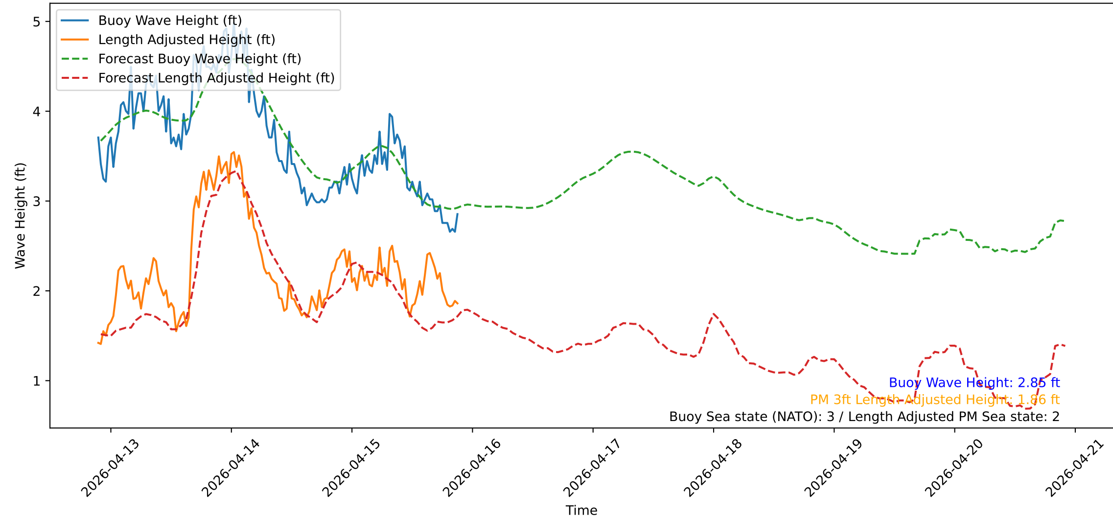
Wave Heights over Time for Green Beach at 2026-04-15 21:41:14
