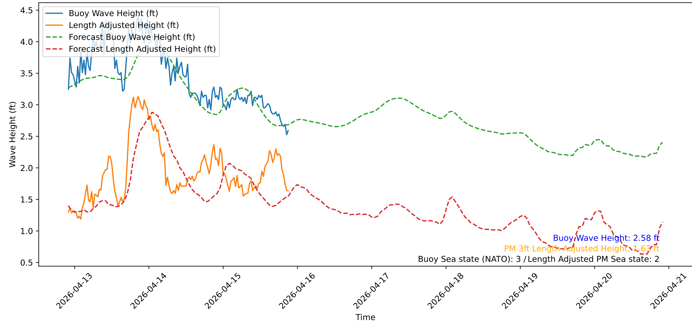
Wave Heights over Time for Red Beach at 2026-04-15 21:40:51
