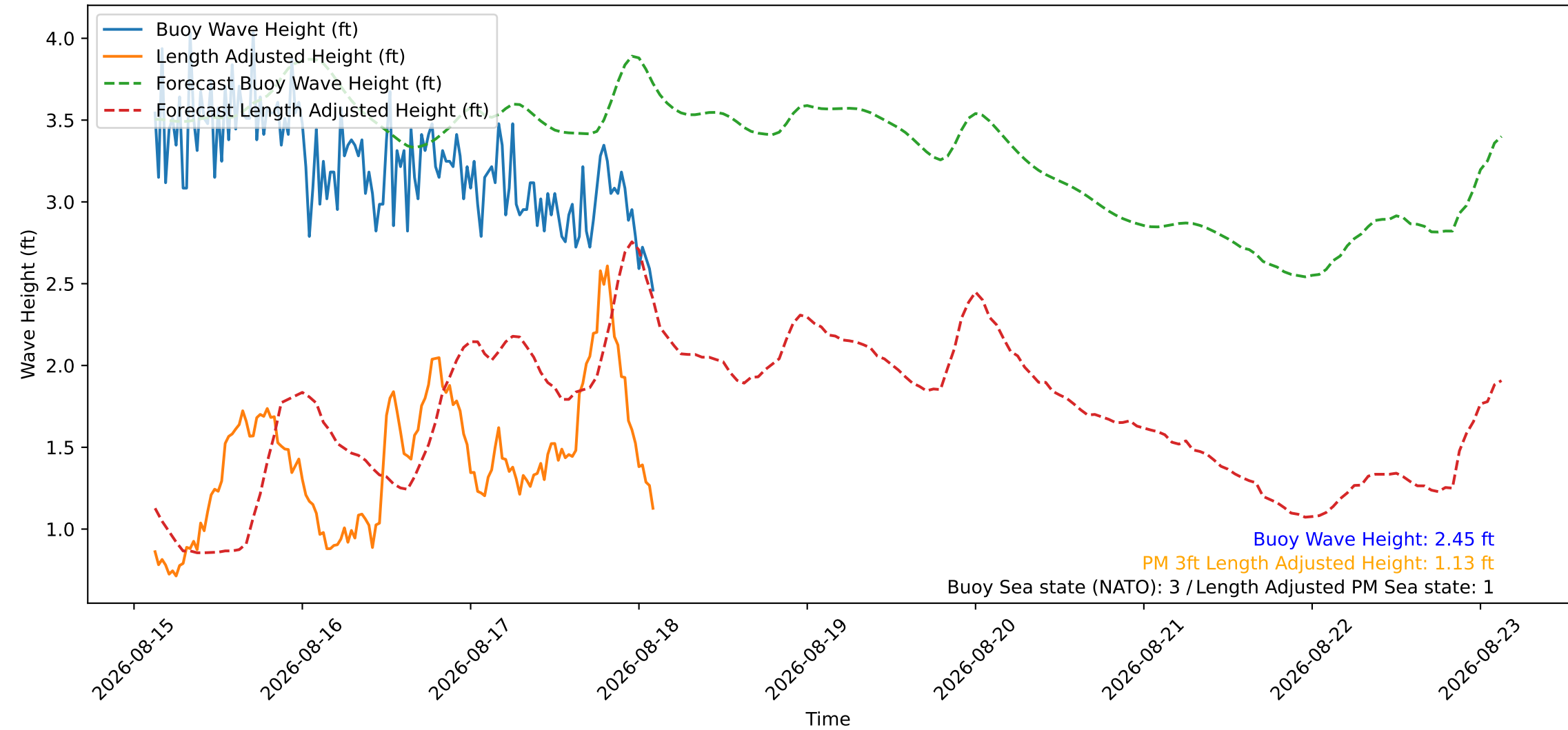
Wave Heights over Time for Red Beach at 2026-08-18 02:50:48
