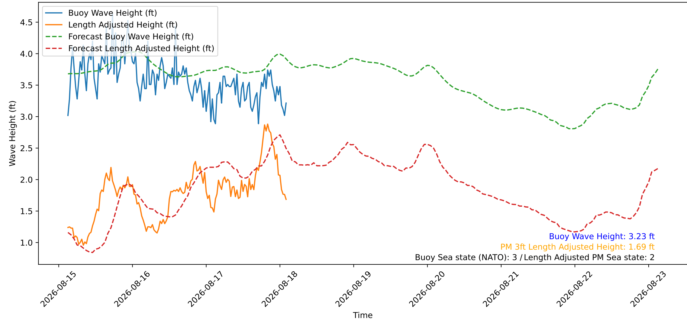
Wave Heights over Time for Oceanside Harbor at 2026-08-18 02:50:27
