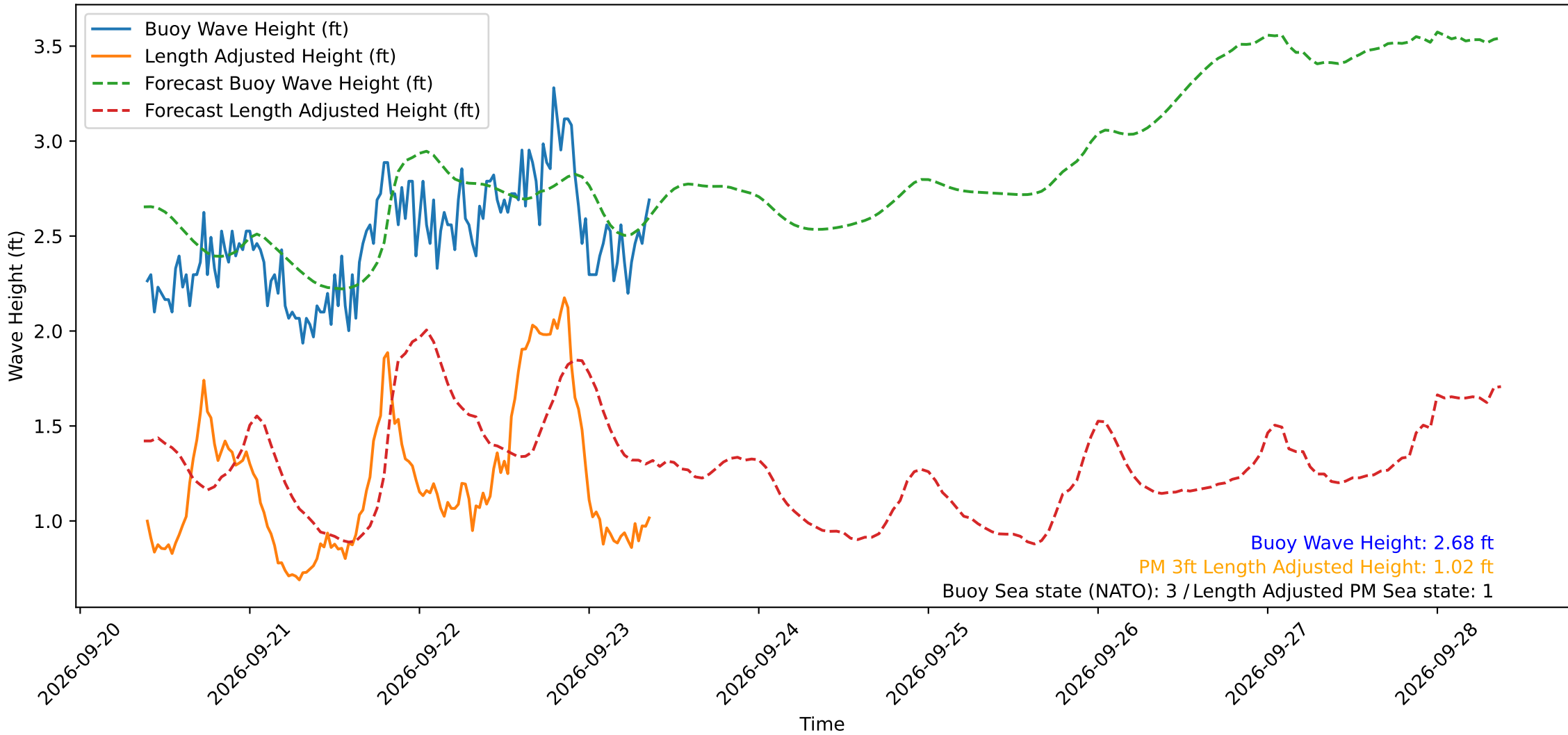
Wave Heights over Time for Red Beach at 2026-09-23 09:10:49
