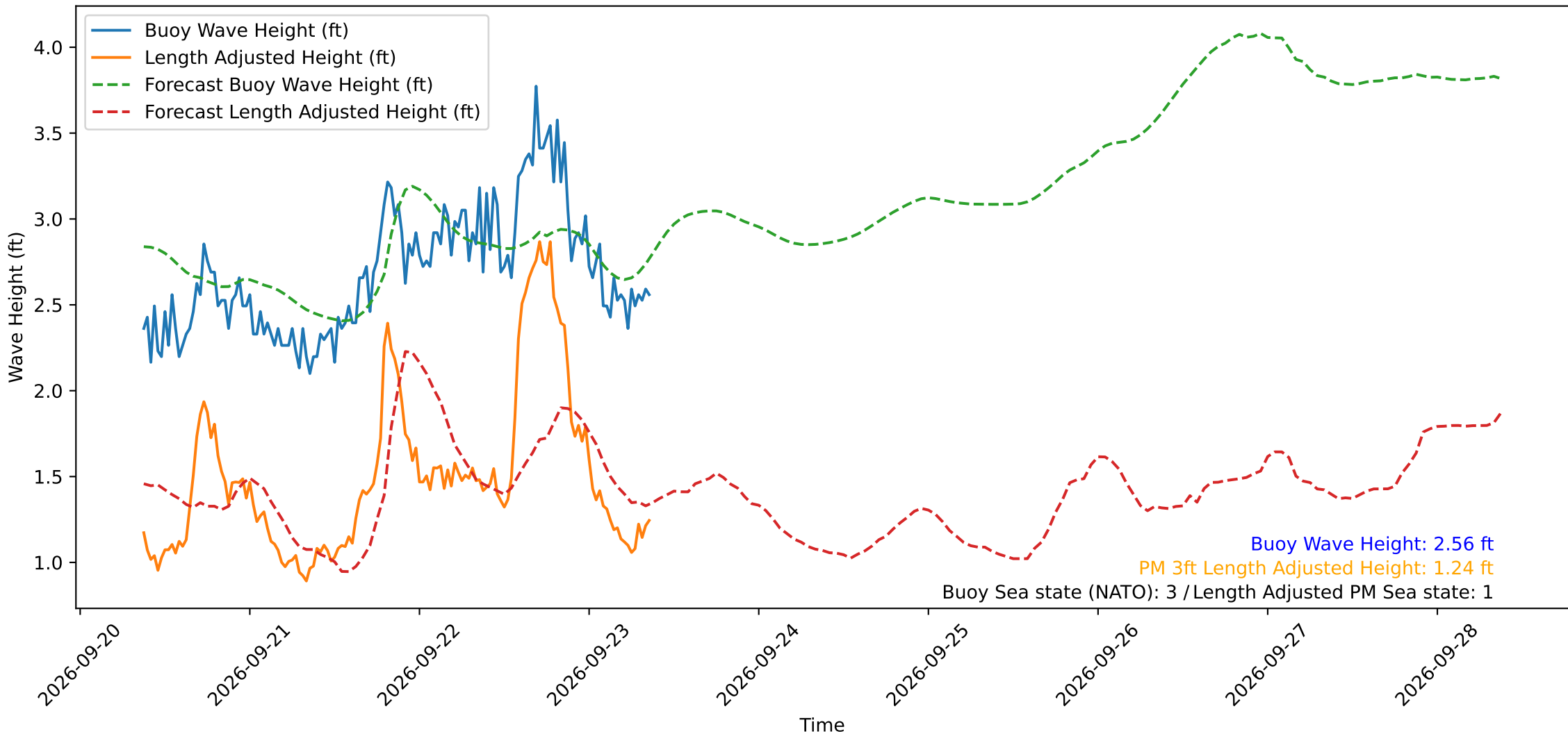
Wave Heights over Time for Oceanside Harbor at 2026-09-23 09:10:29
