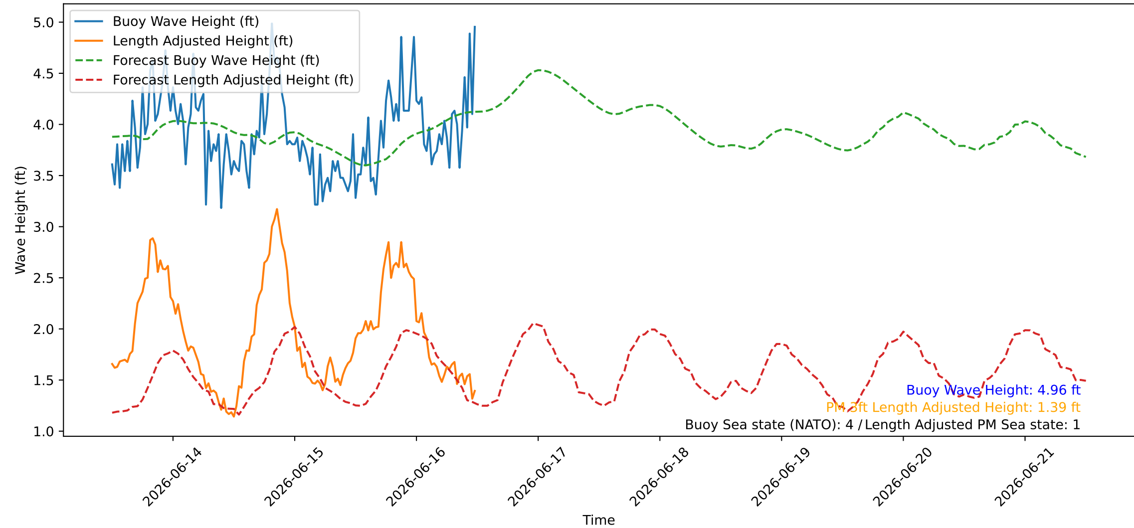
Wave Heights over Time for Oceanside Harbor at 2026-06-16 12:10:26
