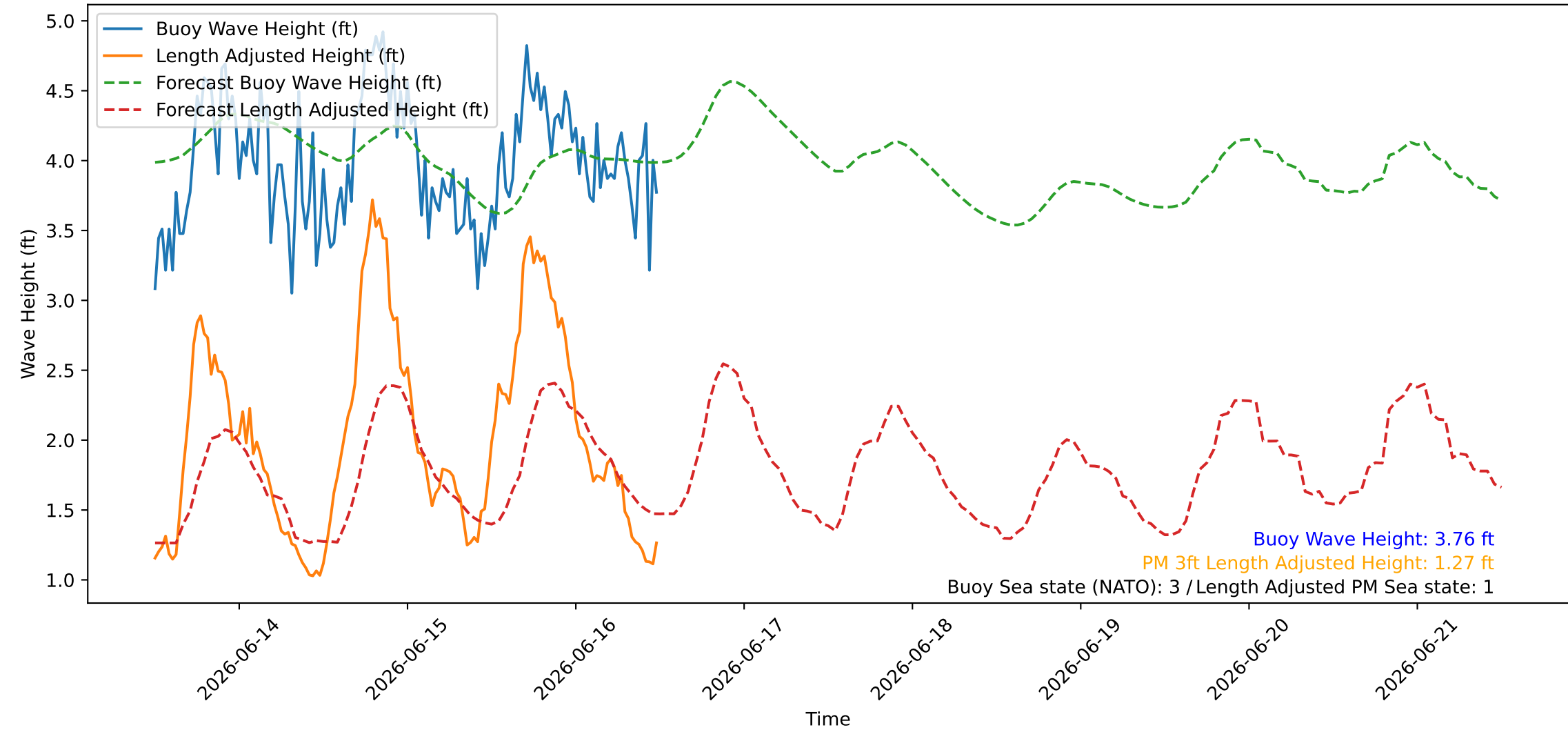
Wave Heights over Time for Green Beach at 2026-06-16 12:11:08
