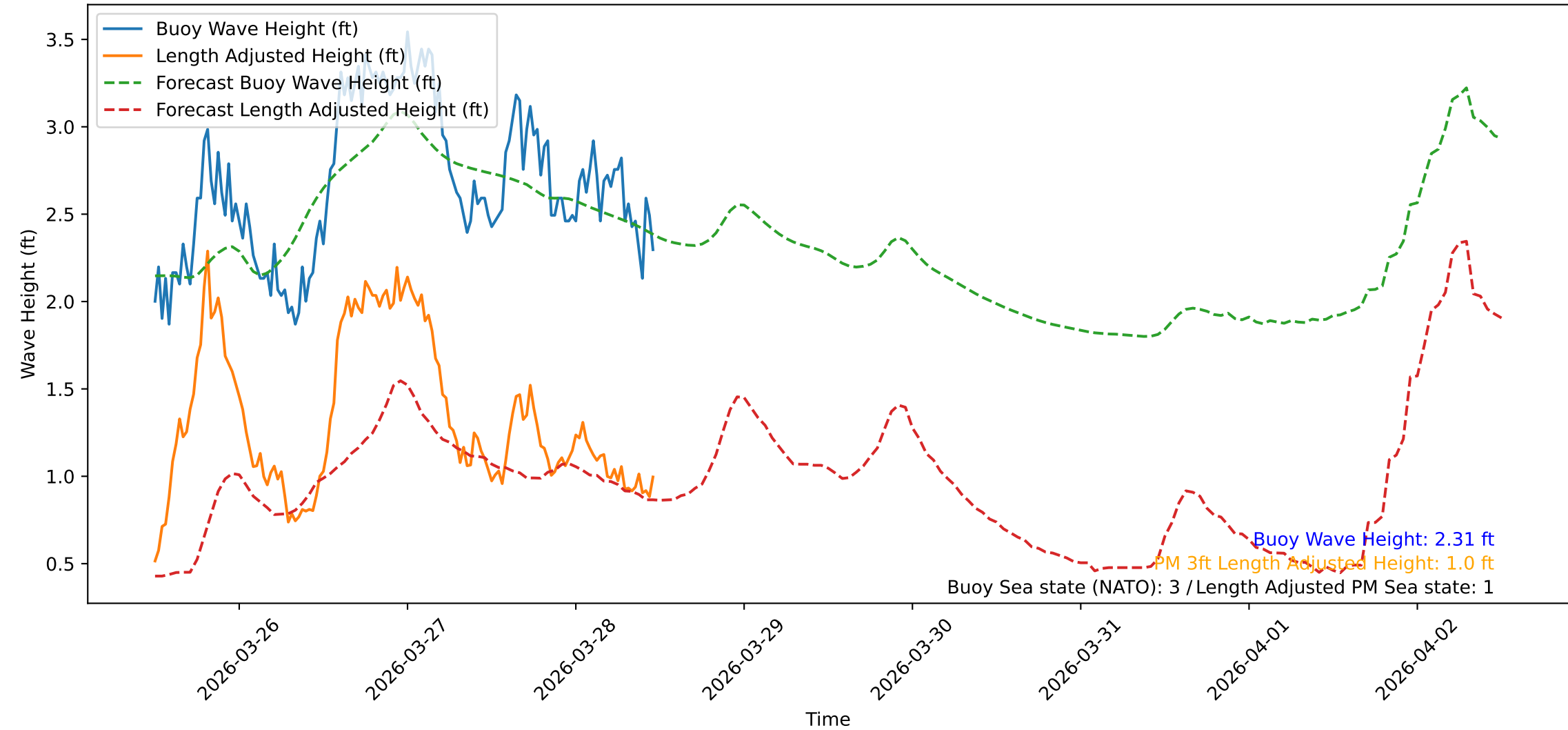
Wave Heights over Time for Green Beach at 2026-03-28 11:51:09
