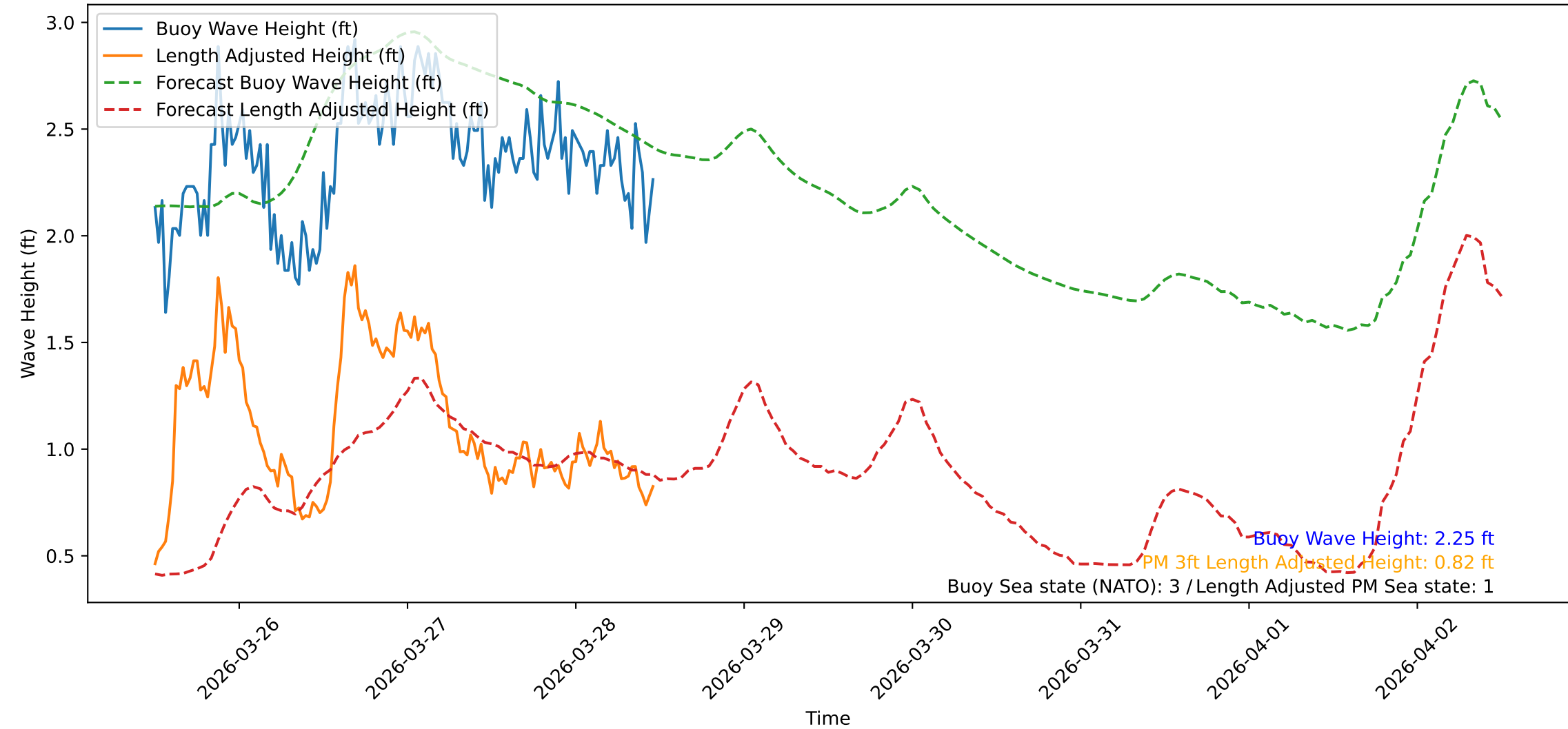
Wave Heights over Time for Oceanside Harbor at 2026-03-28 11:50:31
