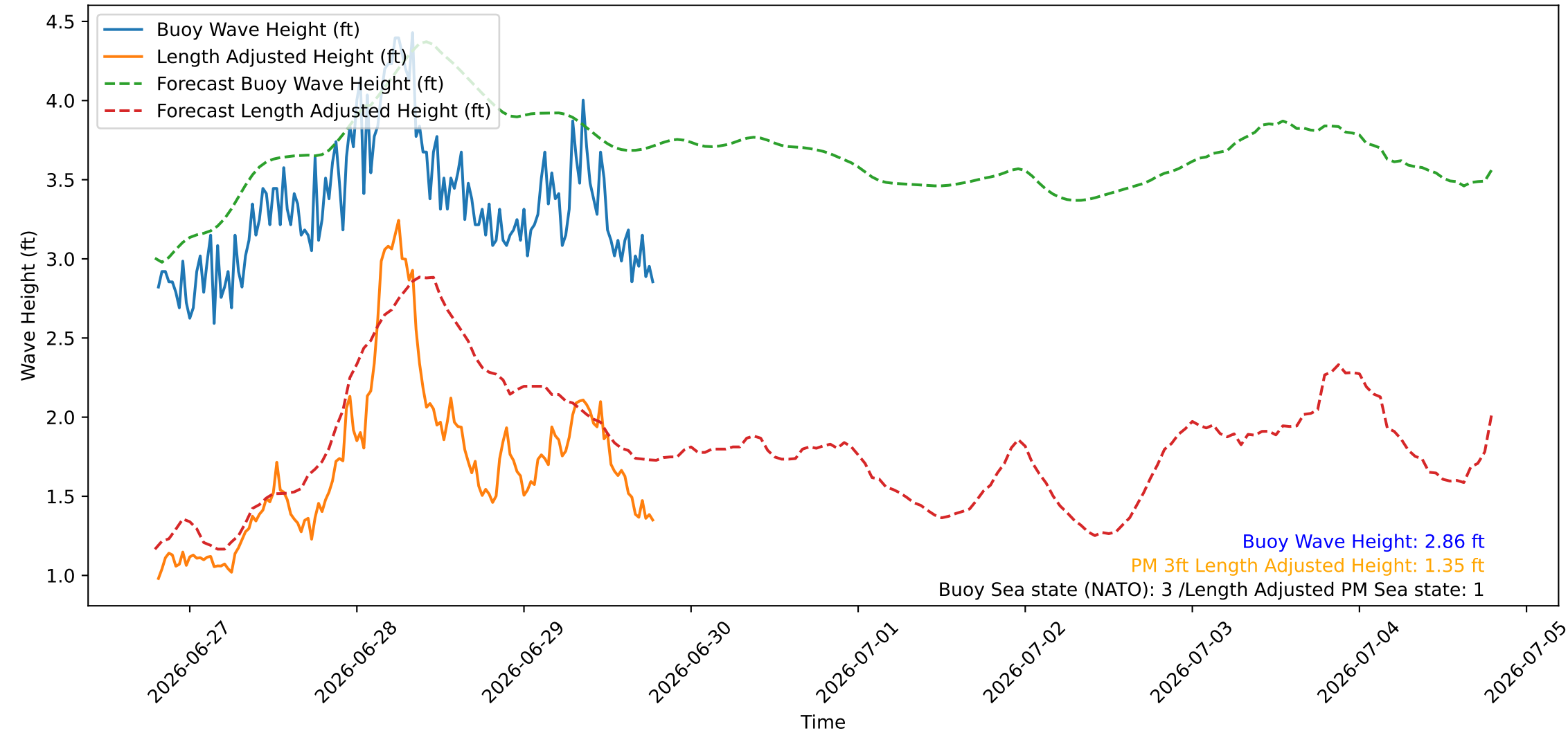
Wave Heights over Time for Oceanside Harbor at 2026-06-29 19:20:26
