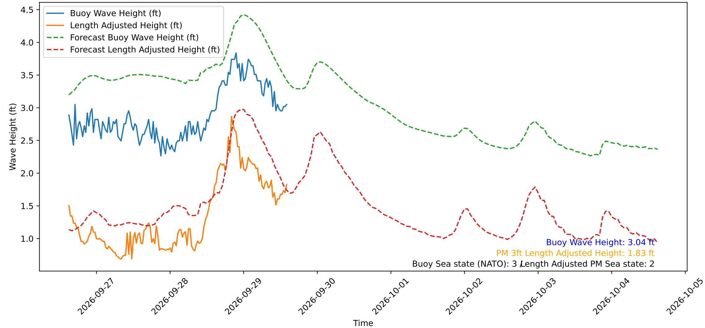
Wave Heights over Time for Red Beach at 2026-09-29 14:40:50
