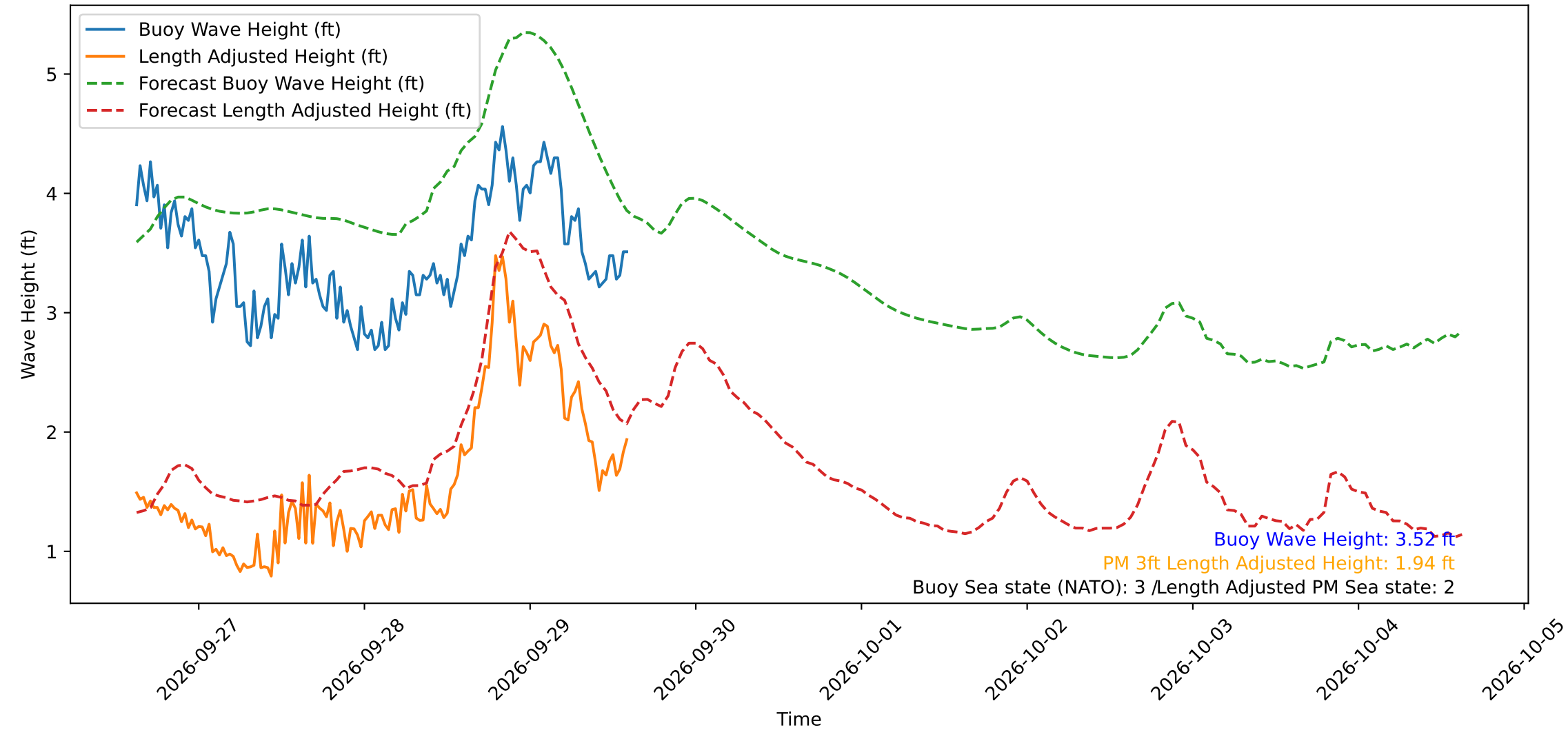
Wave Heights over Time for Green Beach at 2026-09-29 14:41:12
