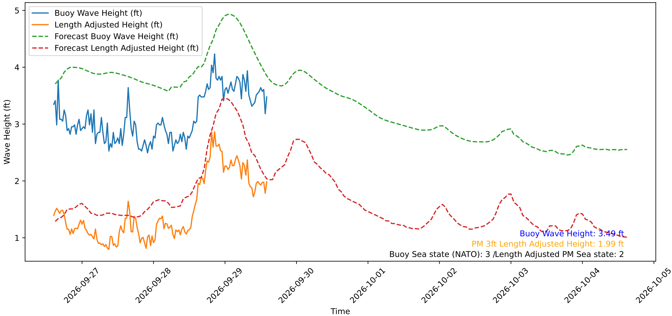
Wave Heights over Time for Oceanside Harbor at 2026-09-29 14:40:30
