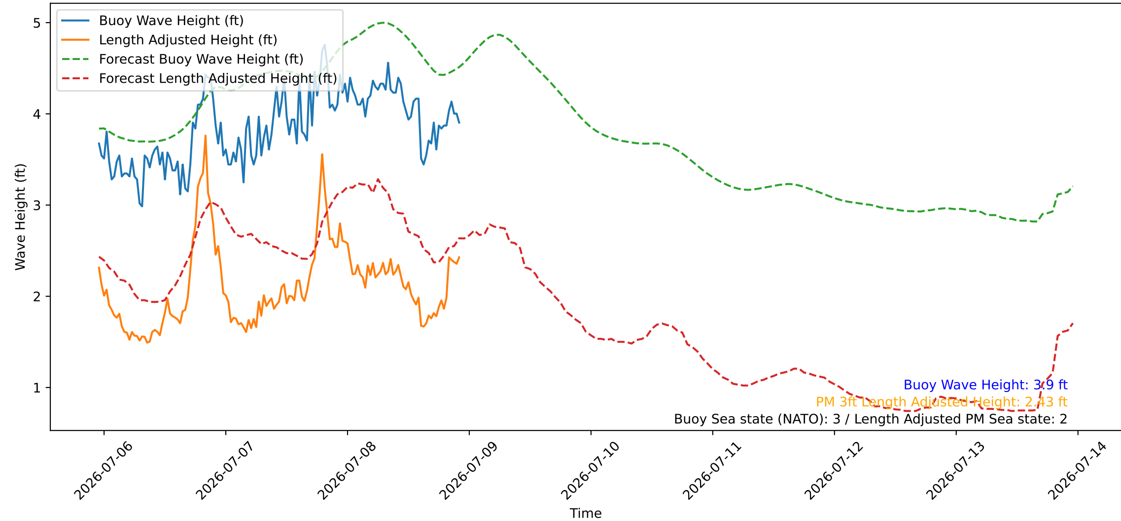
Wave Heights over Time for Green Beach at 2026-07-08 23:01:09
