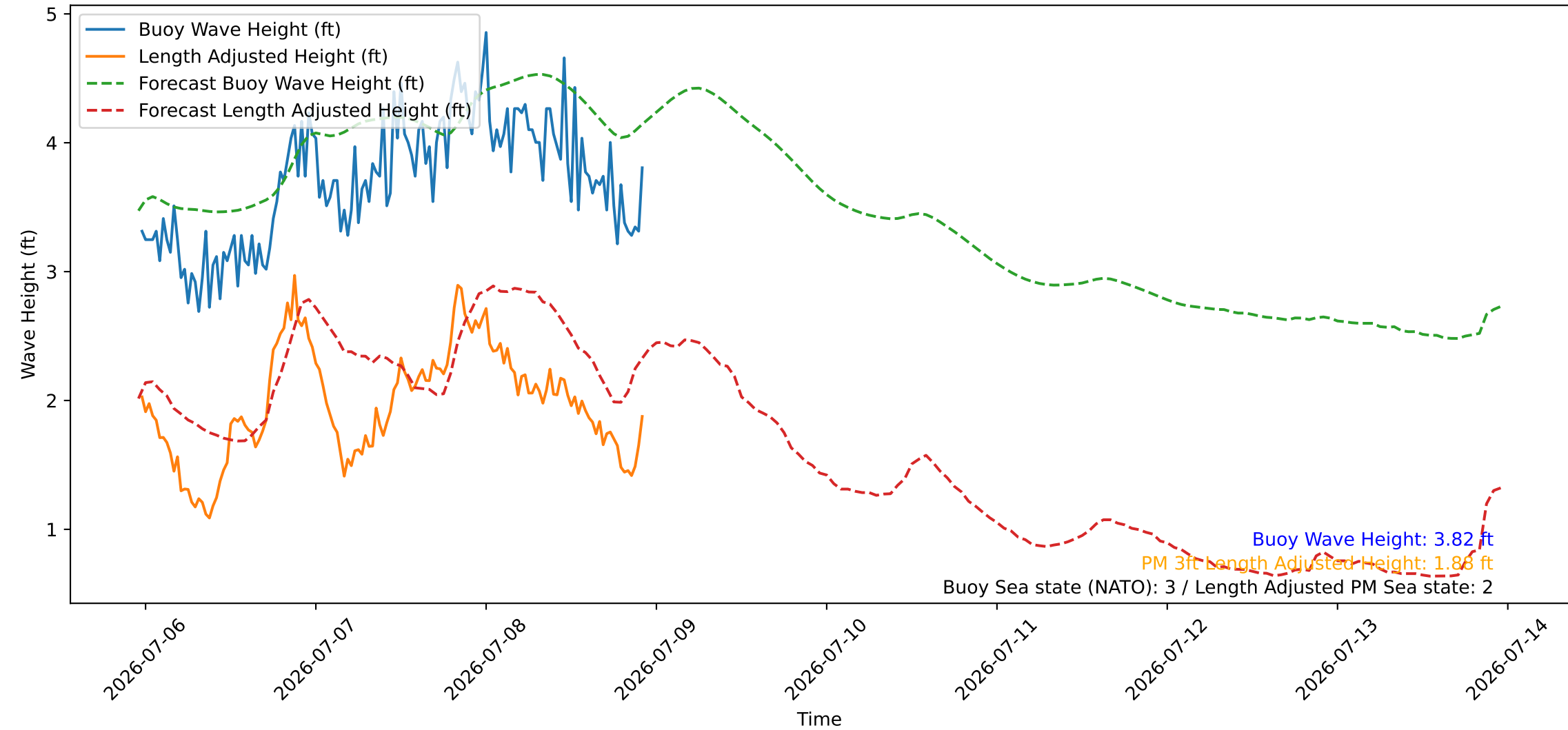
Wave Heights over Time for Red Beach at 2026-07-08 23:00:46
