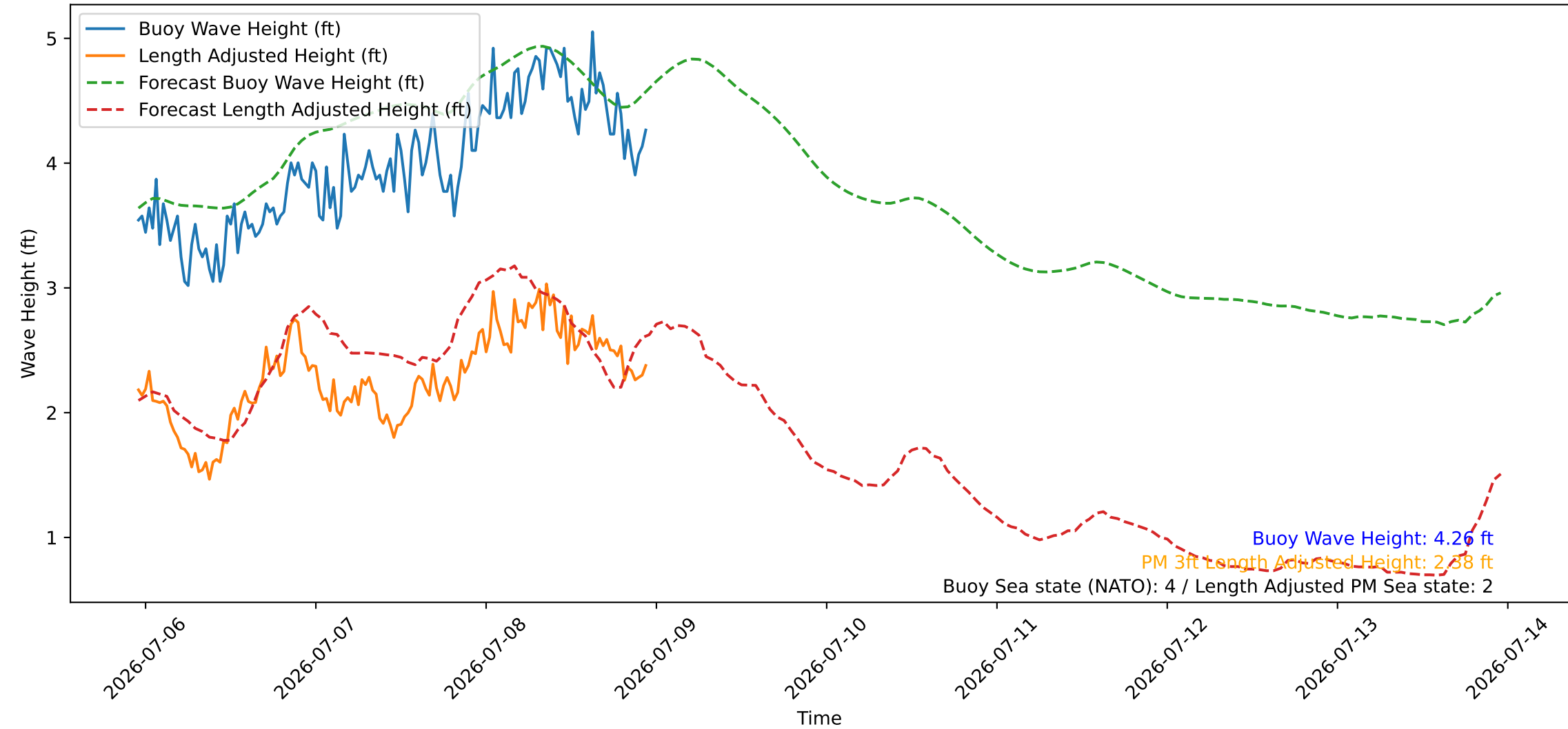
Wave Heights over Time for Oceanside Harbor at 2026-07-08 23:00:26
