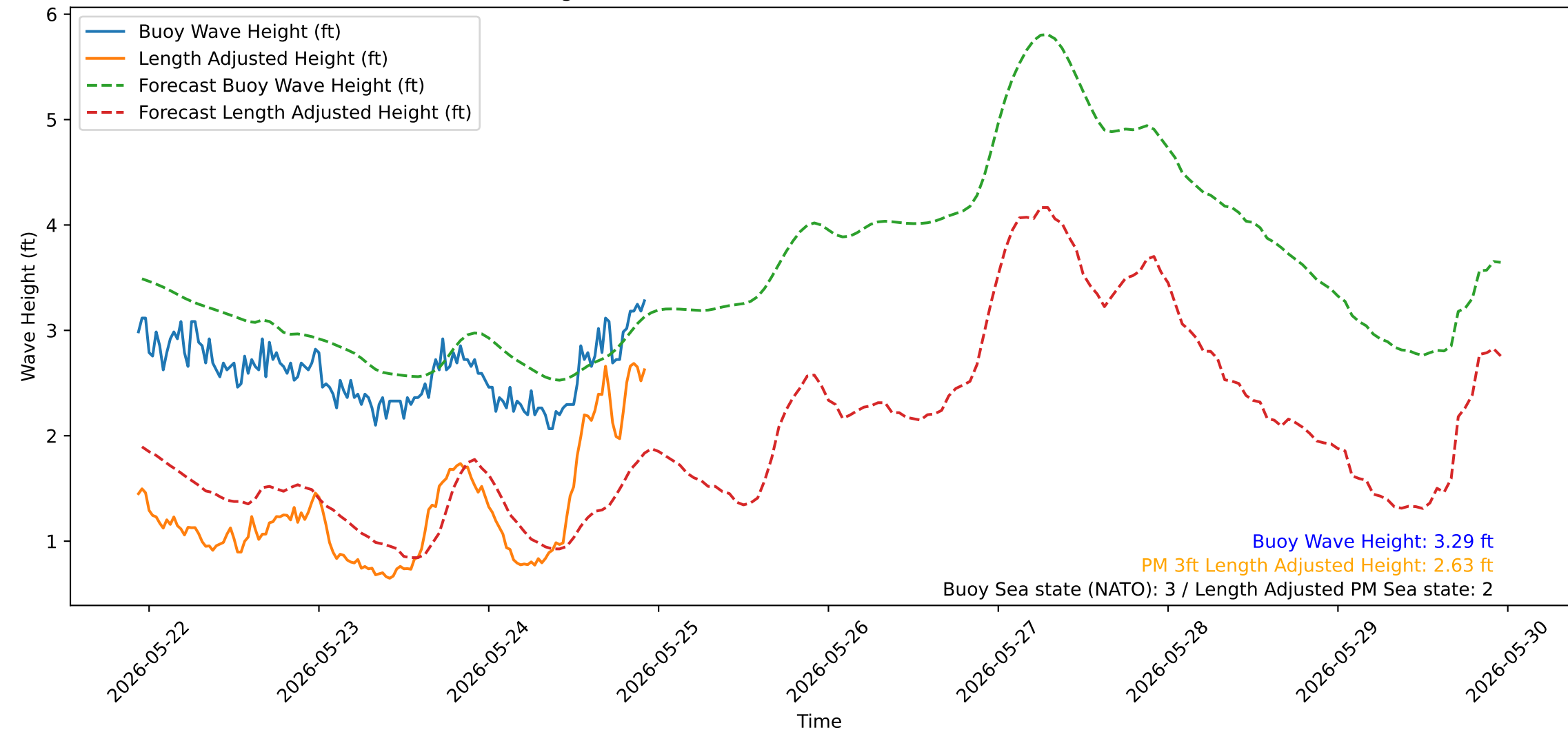
Wave Heights over Time for Green Beach at 2026-05-24 22:41:13
