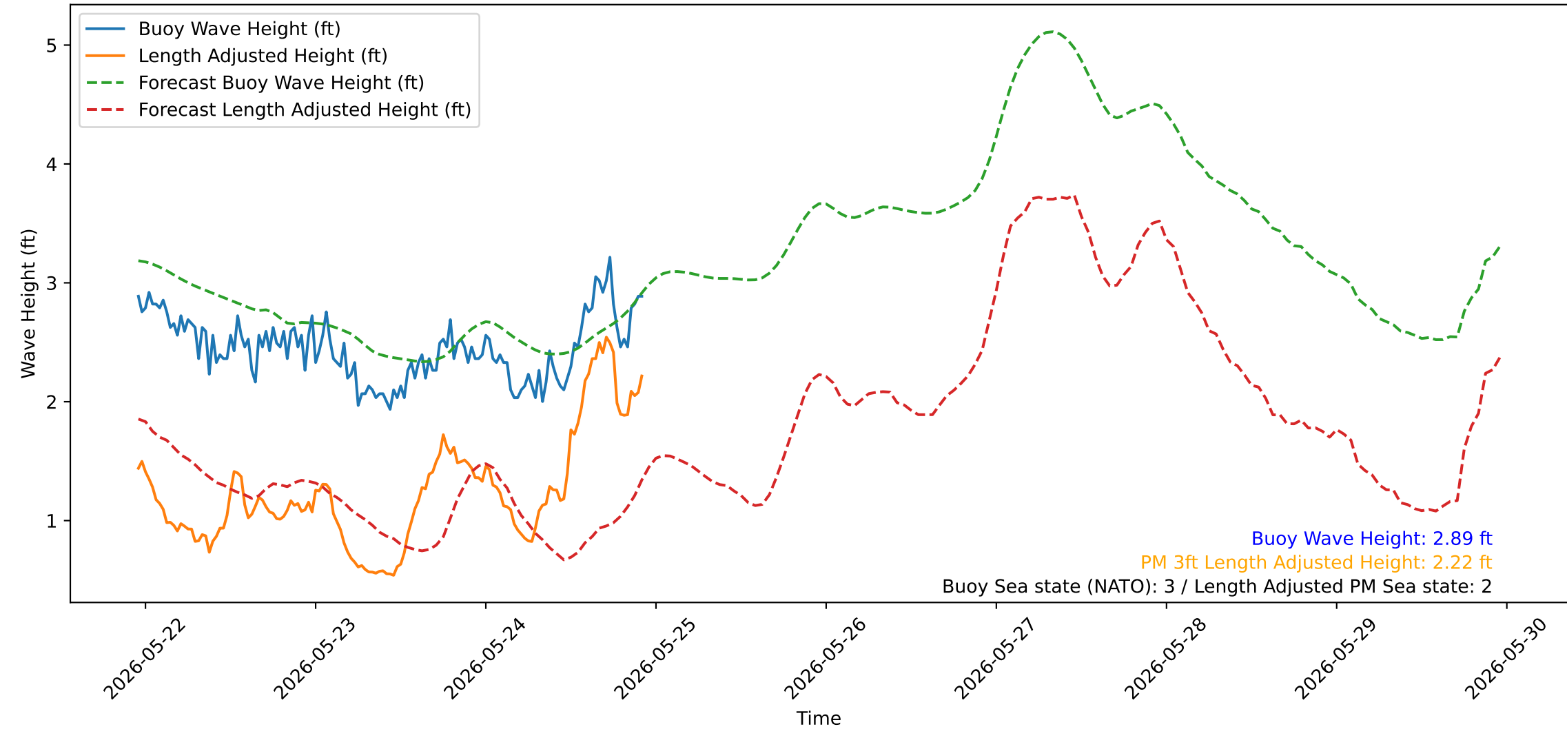
Wave Heights over Time for Red Beach at 2026-05-24 22:40:50
