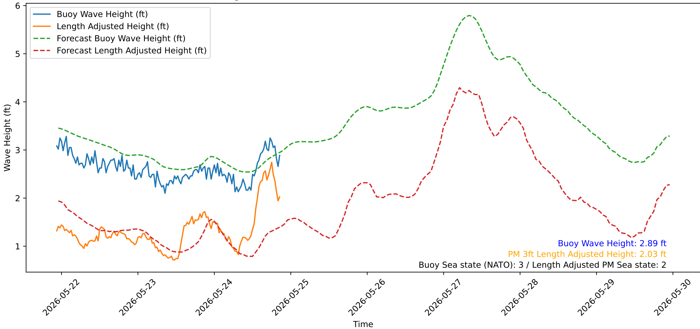
Wave Heights over Time for Oceanside Harbor at 2026-05-24 22:40:31
