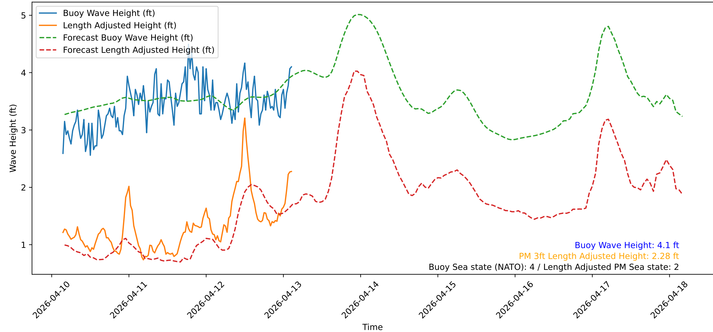
Wave Heights over Time for Green Beach at 2026-04-13 03:31:11
