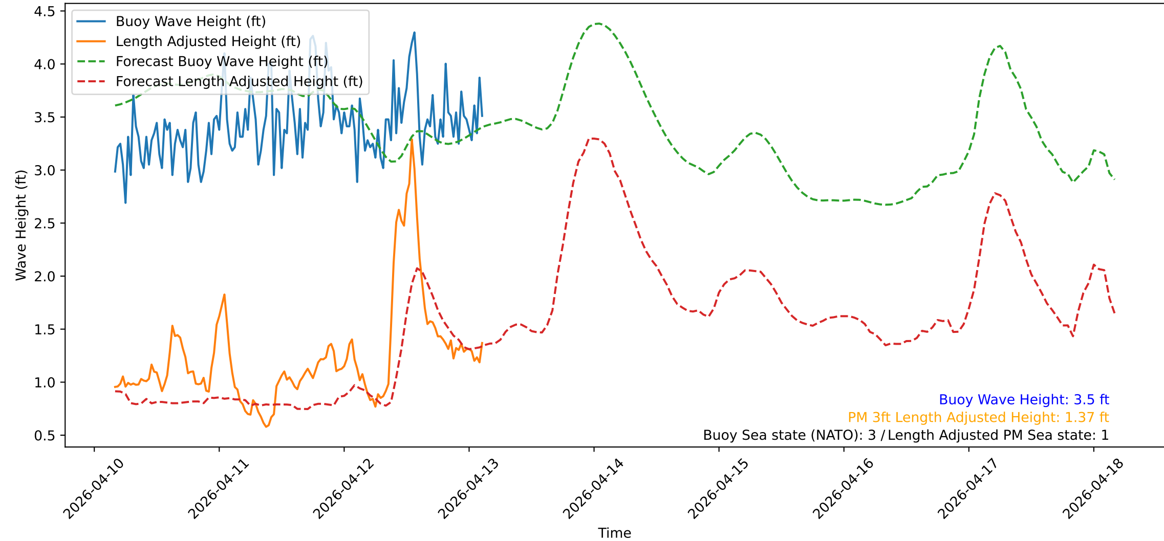
Wave Heights over Time for Red Beach at 2026-04-13 03:30:49
