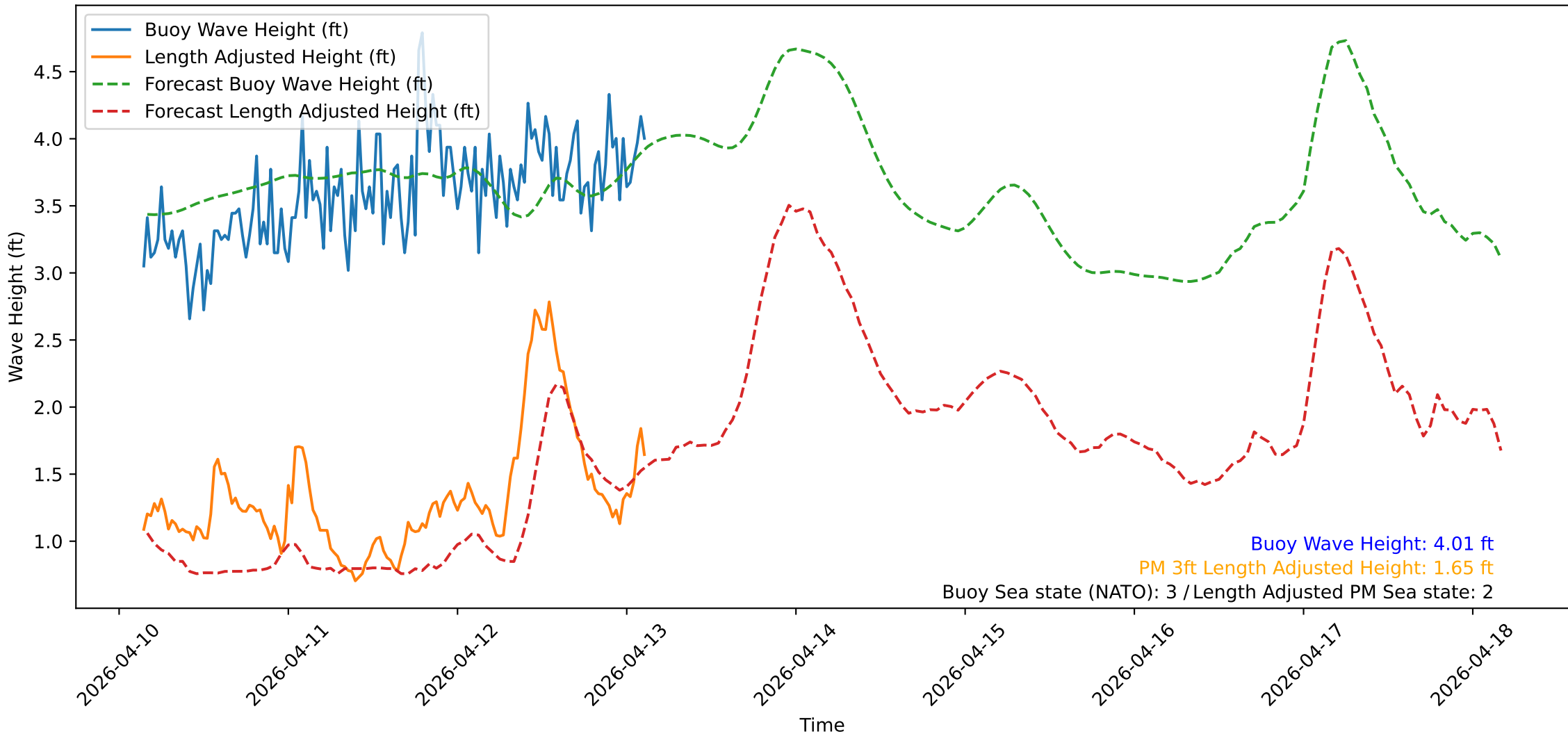
Wave Heights over Time for Oceanside Harbor at 2026-04-13 03:30:30
