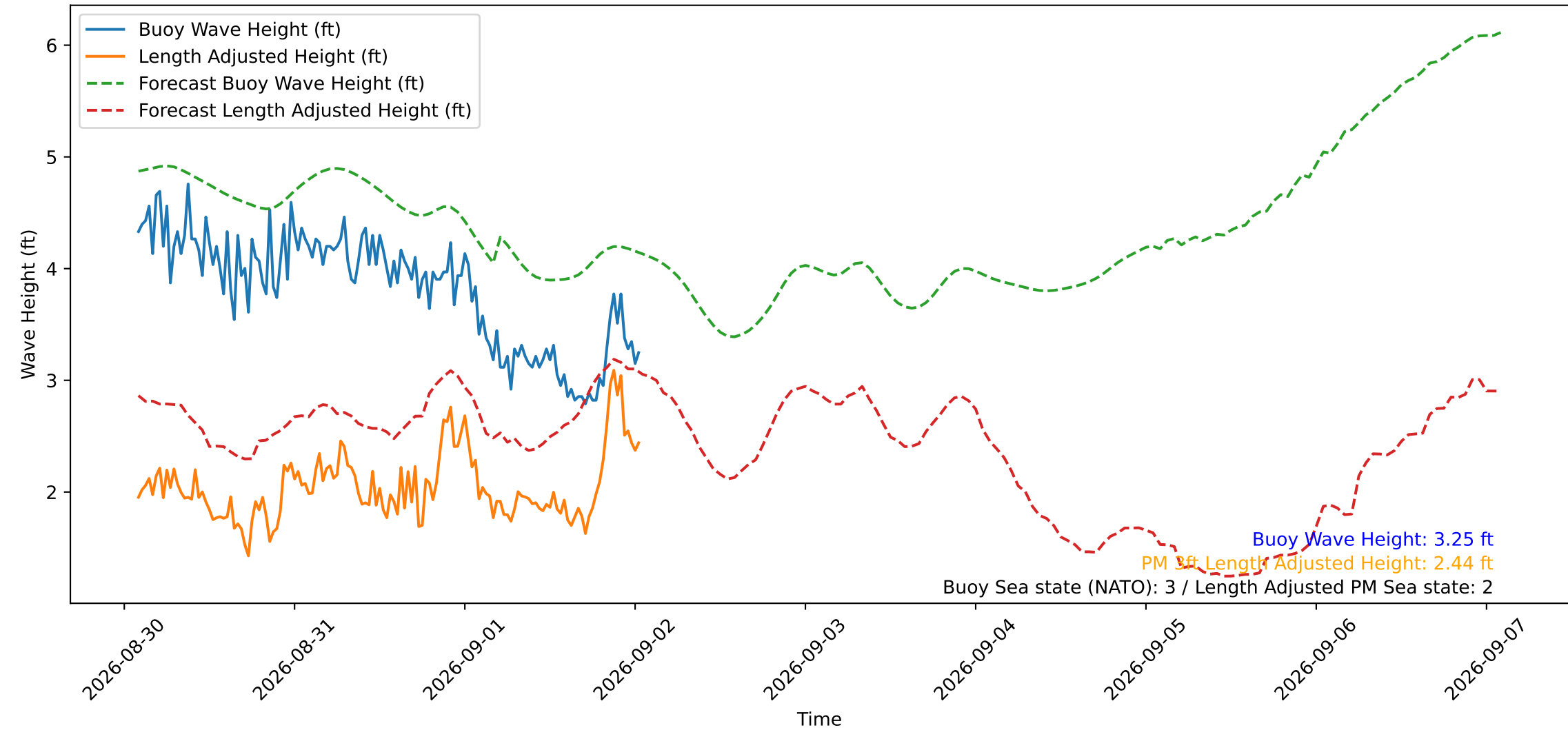
Wave Heights over Time for Green Beach at 2026-09-02 01:31:13
