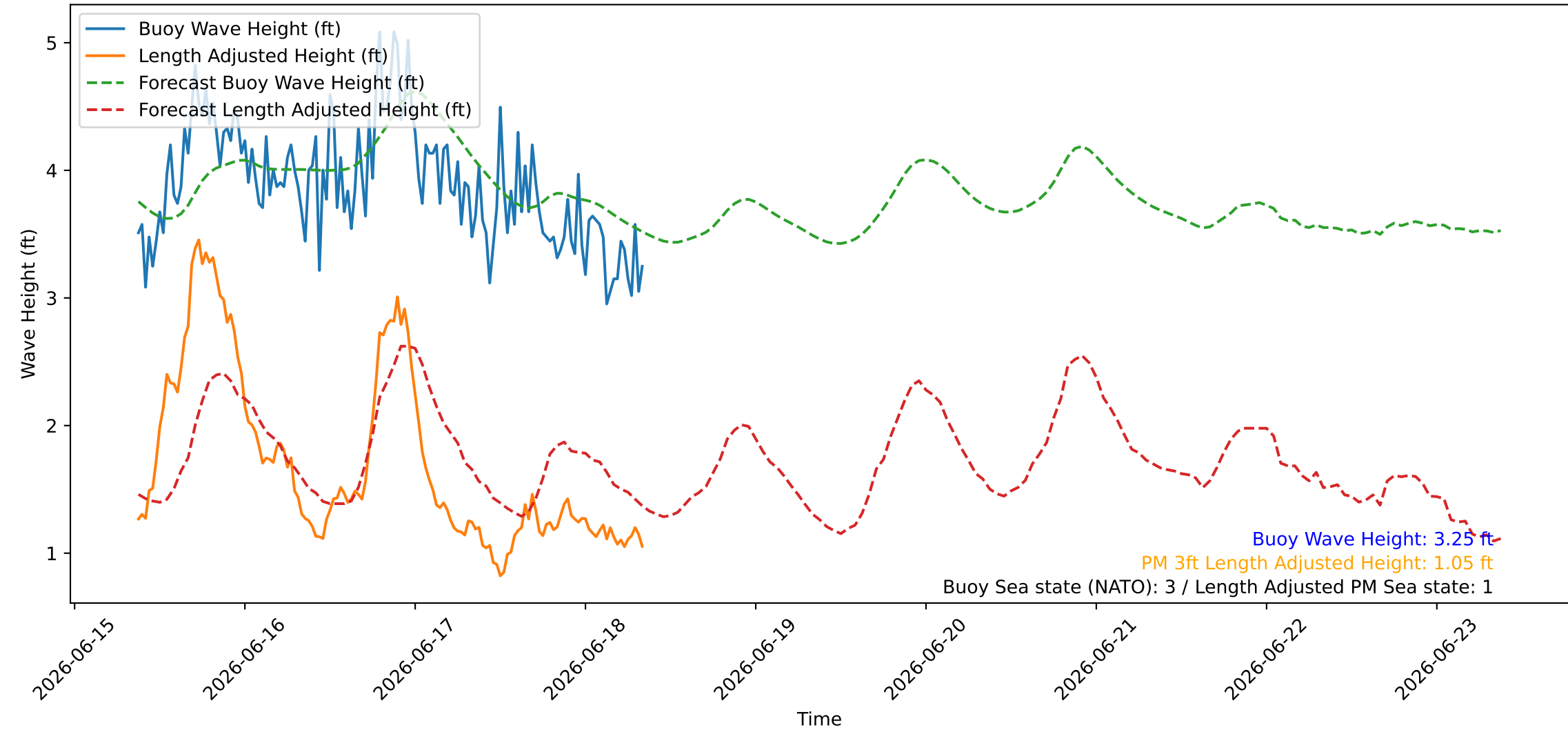
Wave Heights over Time for Green Beach at 2026-06-18 08:51:10
