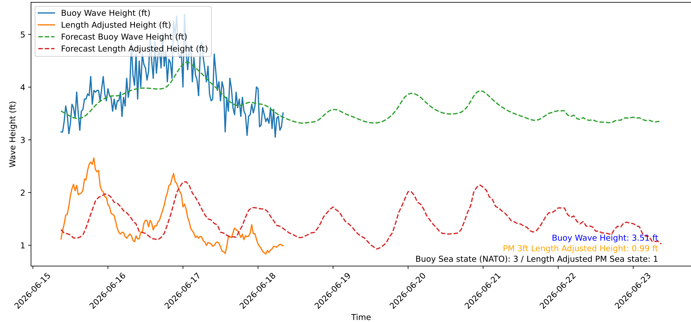
Wave Heights over Time for Red Beach at 2026-06-18 08:50:47
