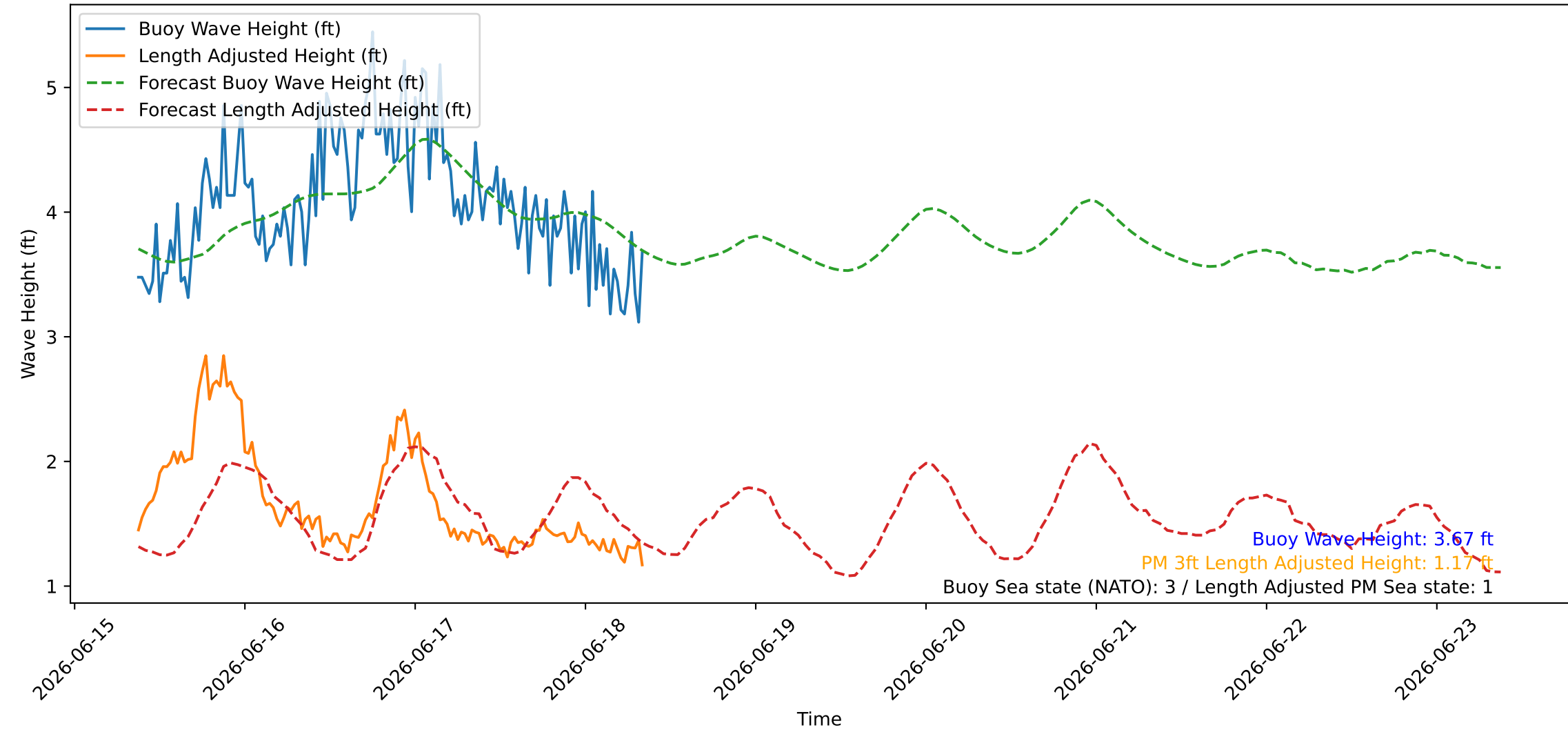
Wave Heights over Time for Oceanside Harbor at 2026-06-18 08:50:26
