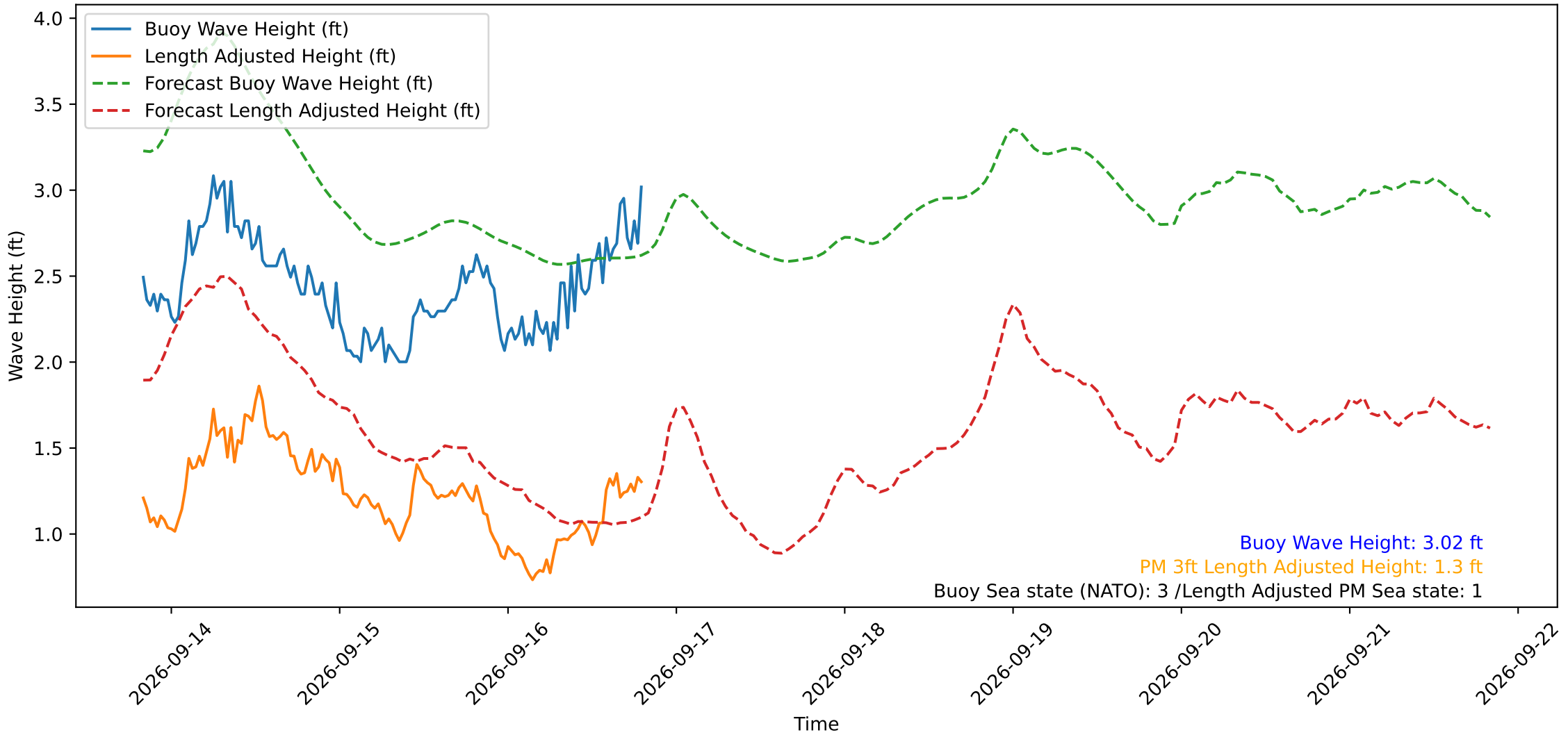
Wave Heights over Time for Red Beach at 2026-09-16 19:50:51
