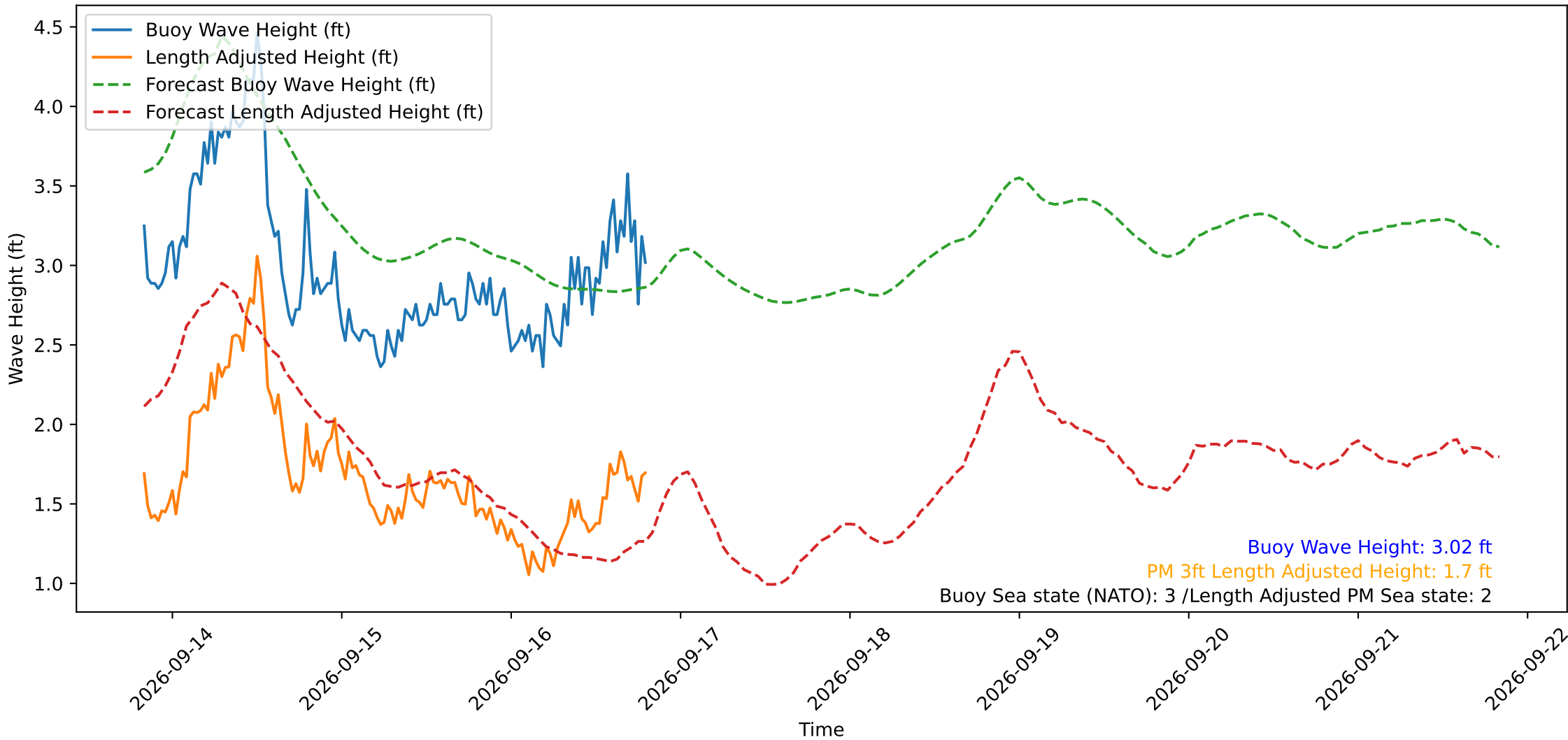
Wave Heights over Time for Oceanside Harbor at 2026-09-16 19:50:30
