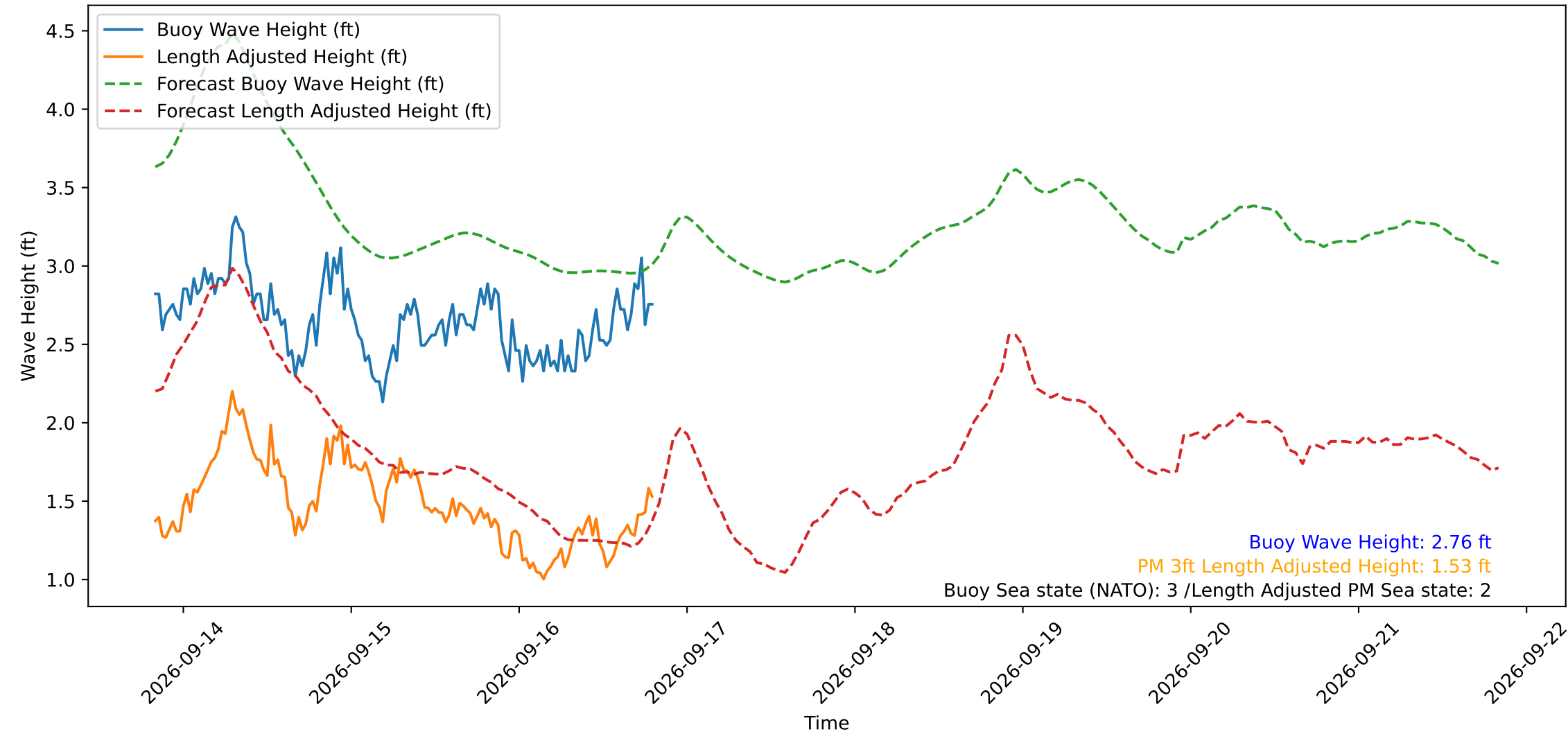
Wave Heights over Time for Green Beach at 2026-09-16 19:51:15
