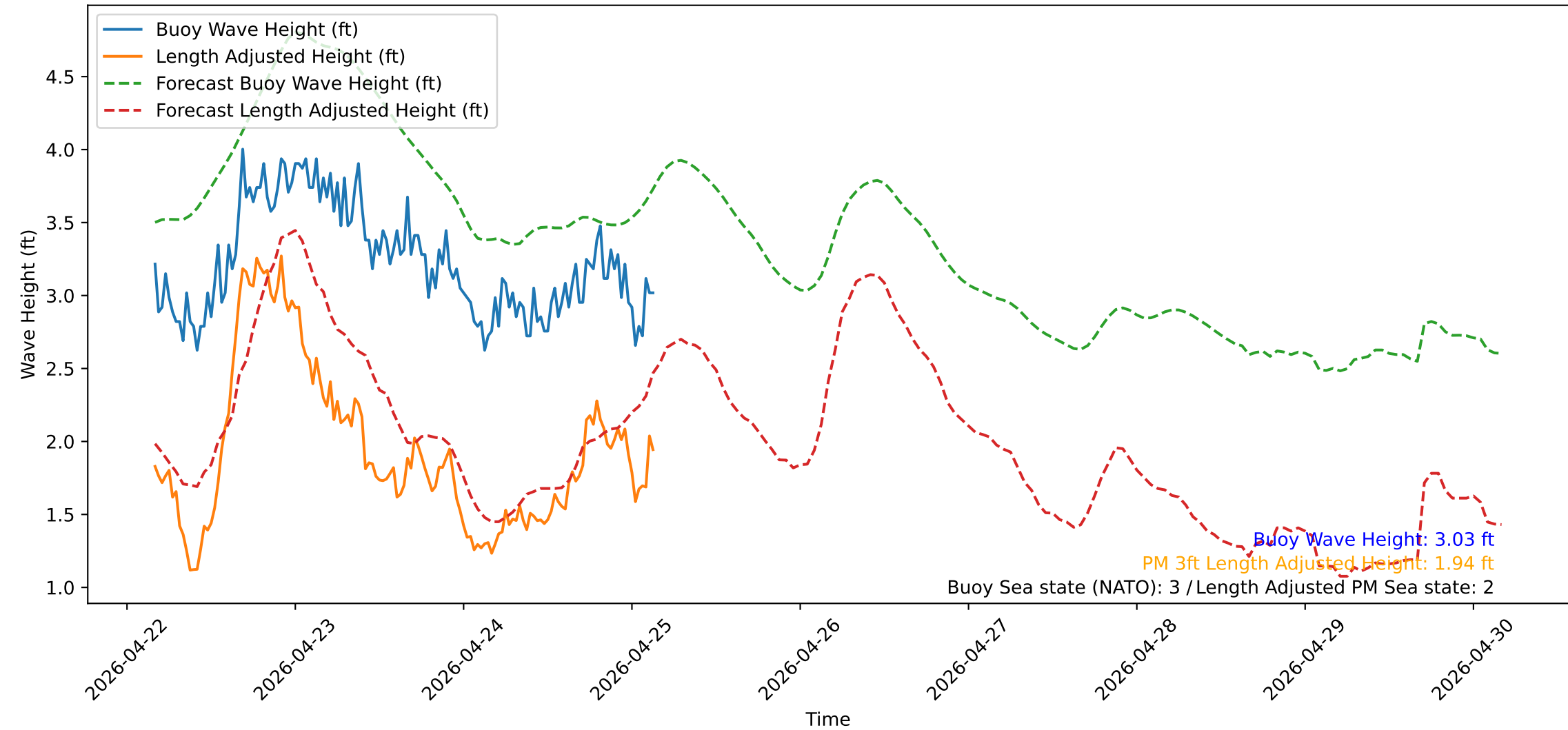
Wave Heights over Time for Green Beach at 2026-04-25 03:51:15
