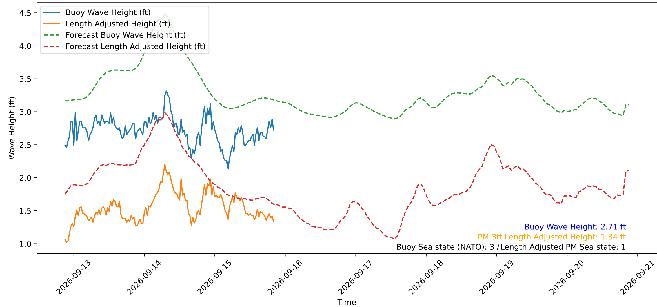
Wave Heights over Time for Green Beach at 2026-09-15 20:51:13
