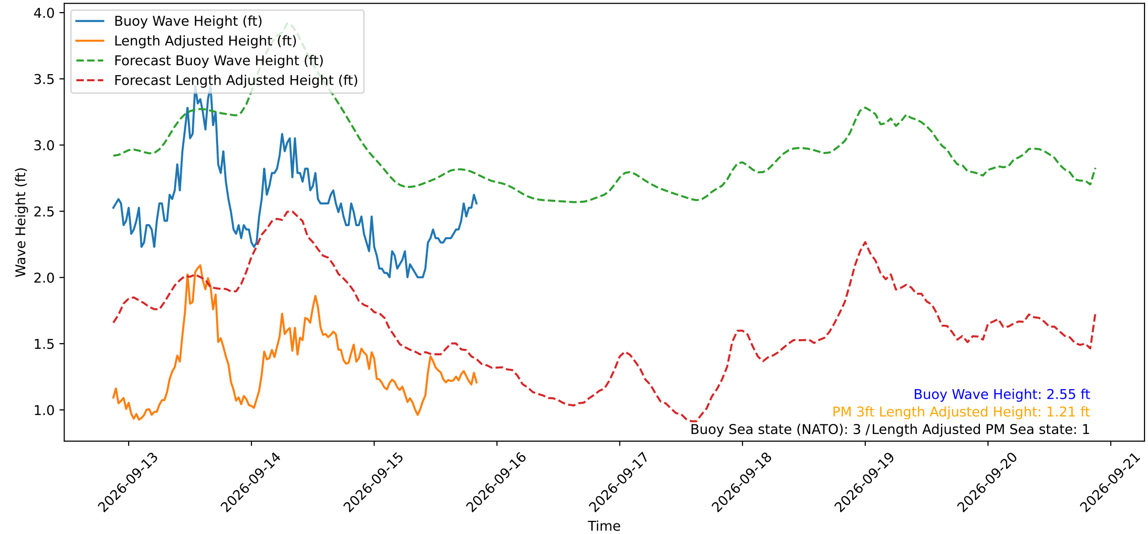
Wave Heights over Time for Red Beach at 2026-09-15 20:50:50
