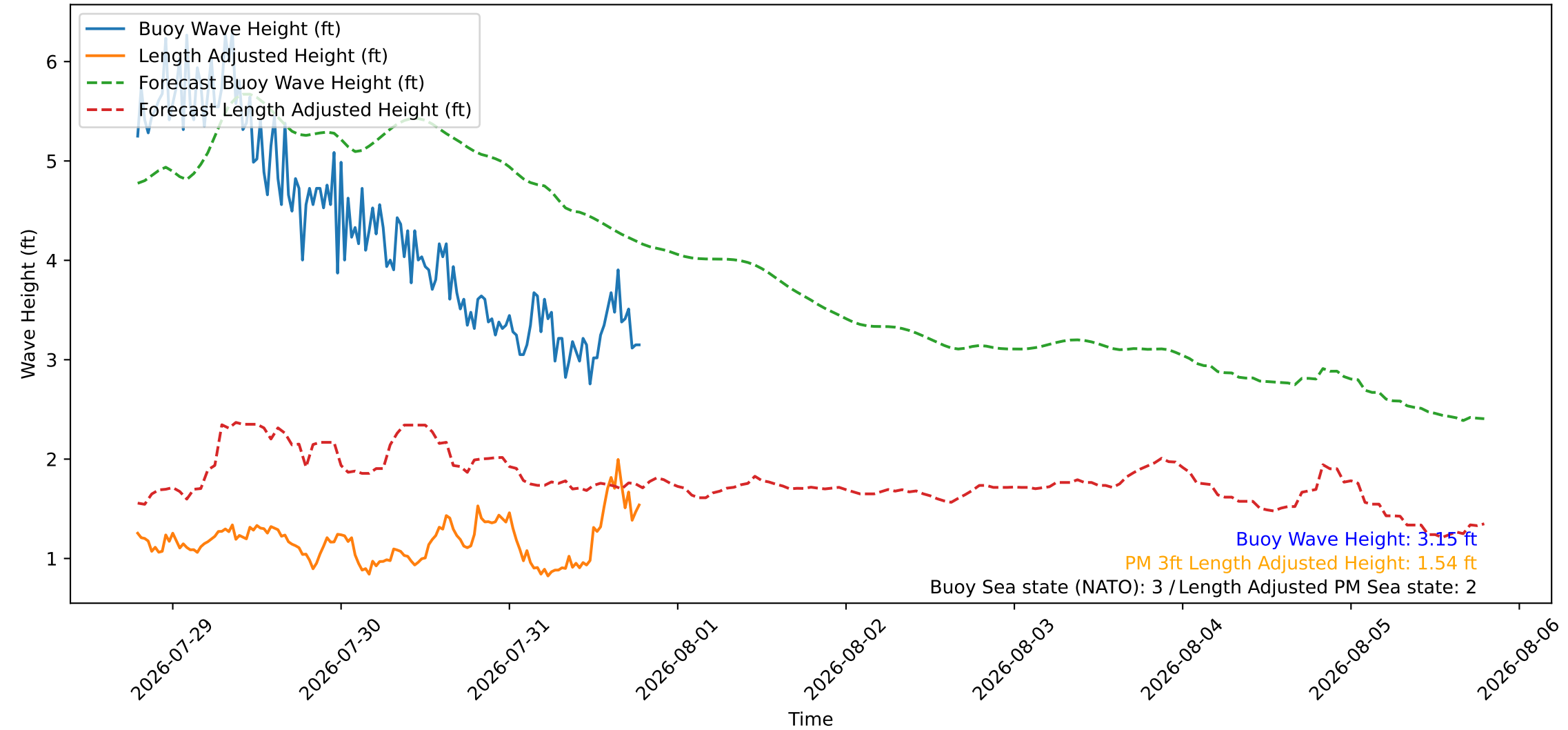
Wave Heights over Time for Green Beach at 2026-07-31 19:11:08
