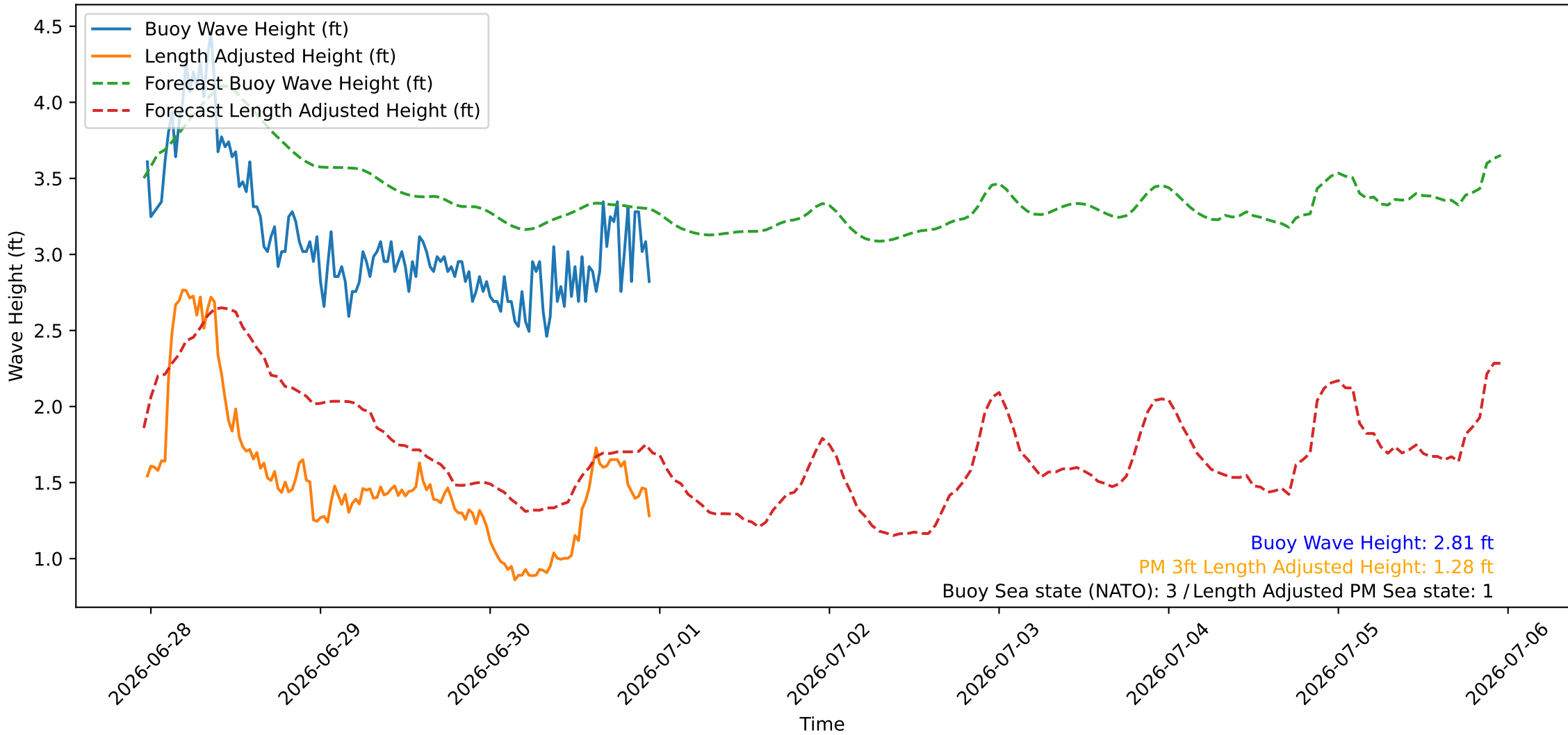
Wave Heights over Time for Red Beach at 2026-06-30 23:10:45
