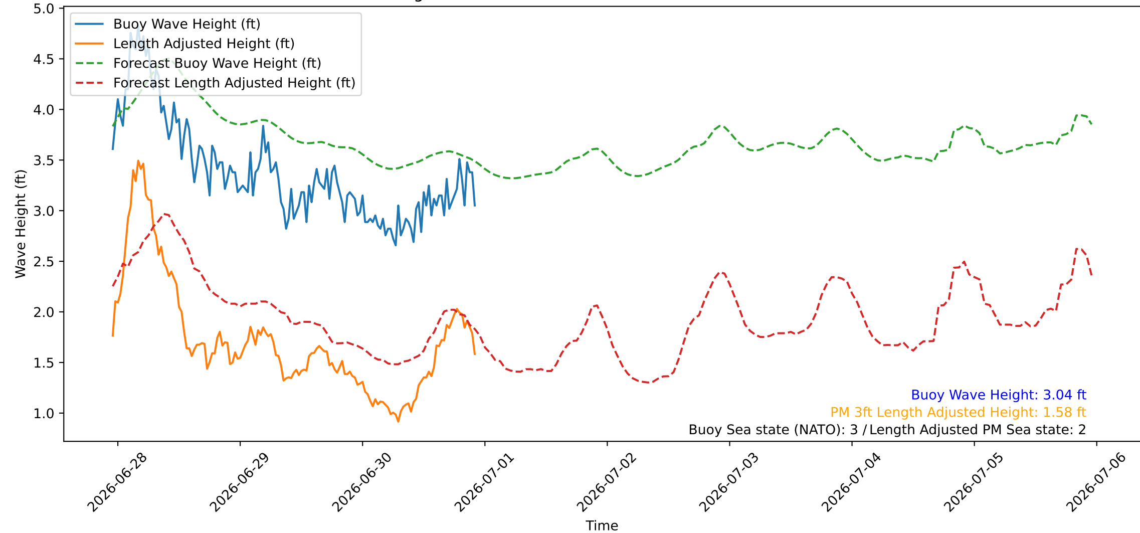
Wave Heights over Time for Green Beach at 2026-06-30 23:11:07
