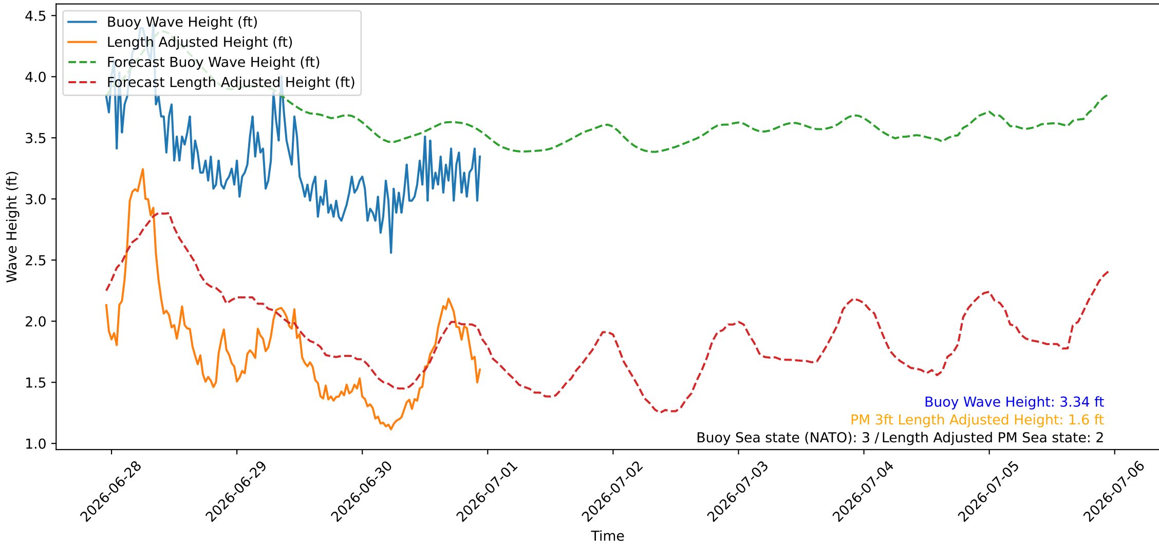
Wave Heights over Time for Oceanside Harbor at 2026-06-30 23:10:26
