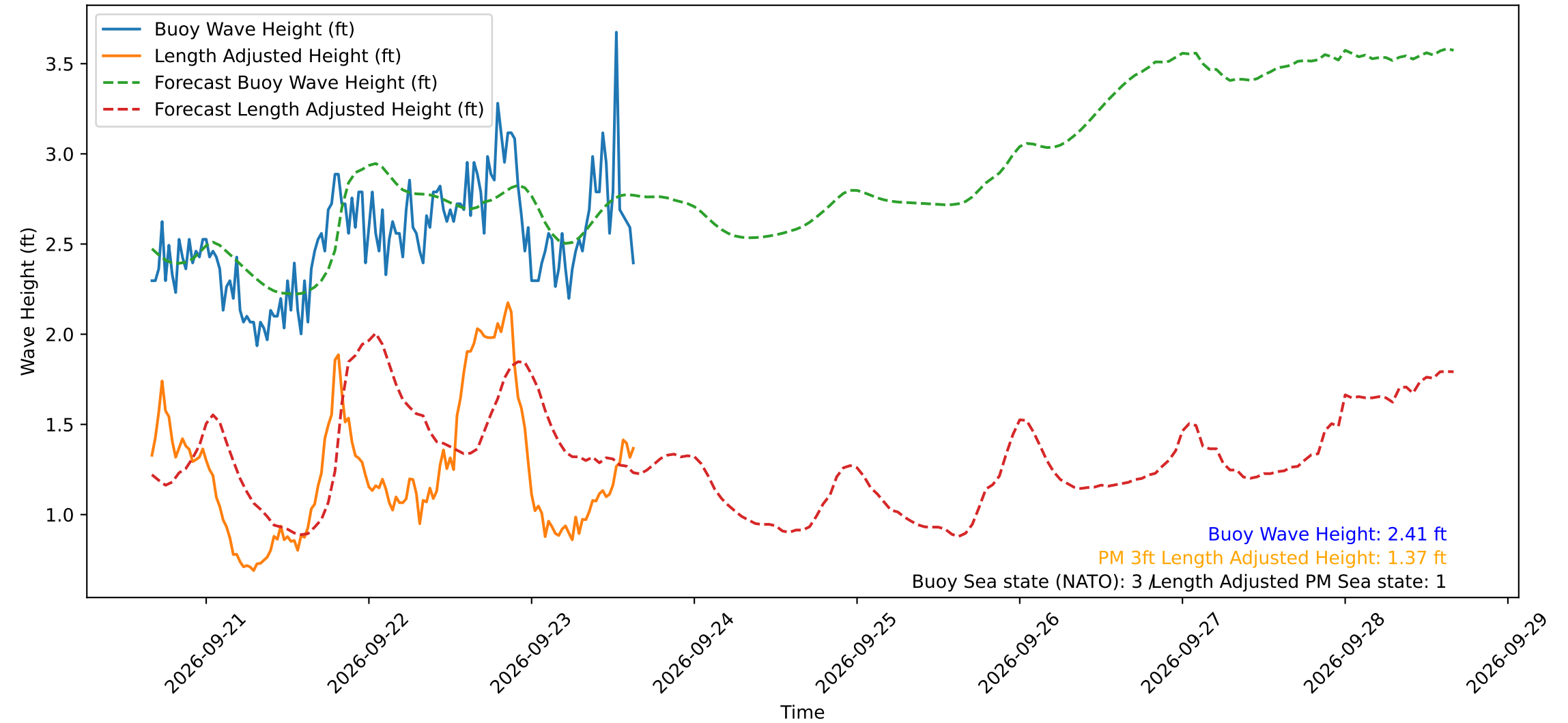
Wave Heights over Time for Red Beach at 2026-09-23 15:50:50
