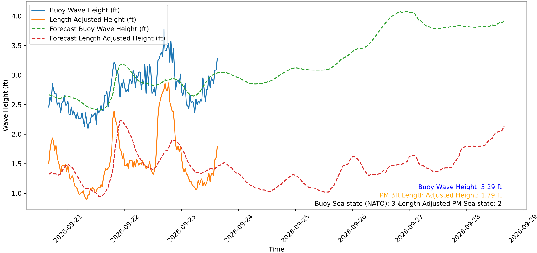
Wave Heights over Time for Oceanside Harbor at 2026-09-23 15:50:29
