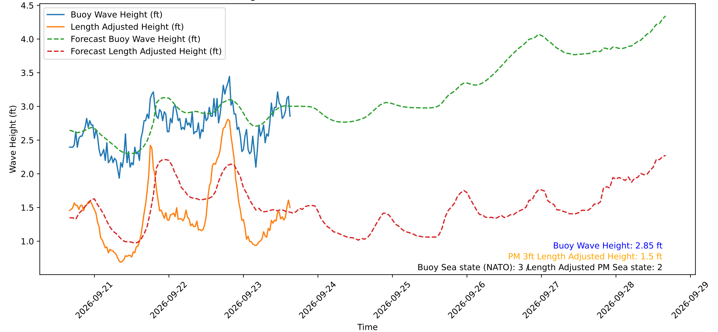
Wave Heights over Time for Green Beach at 2026-09-23 15:51:14
