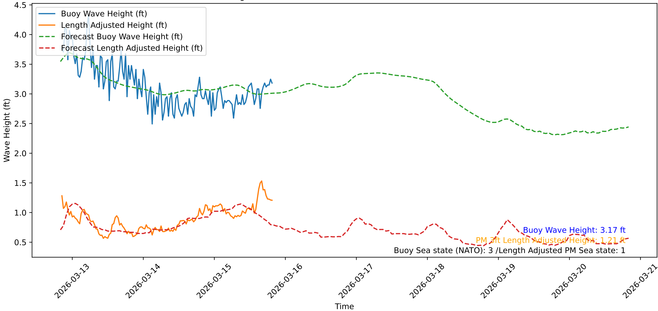
Wave Heights over Time for Red Beach at 2026-03-15 20:21:19
