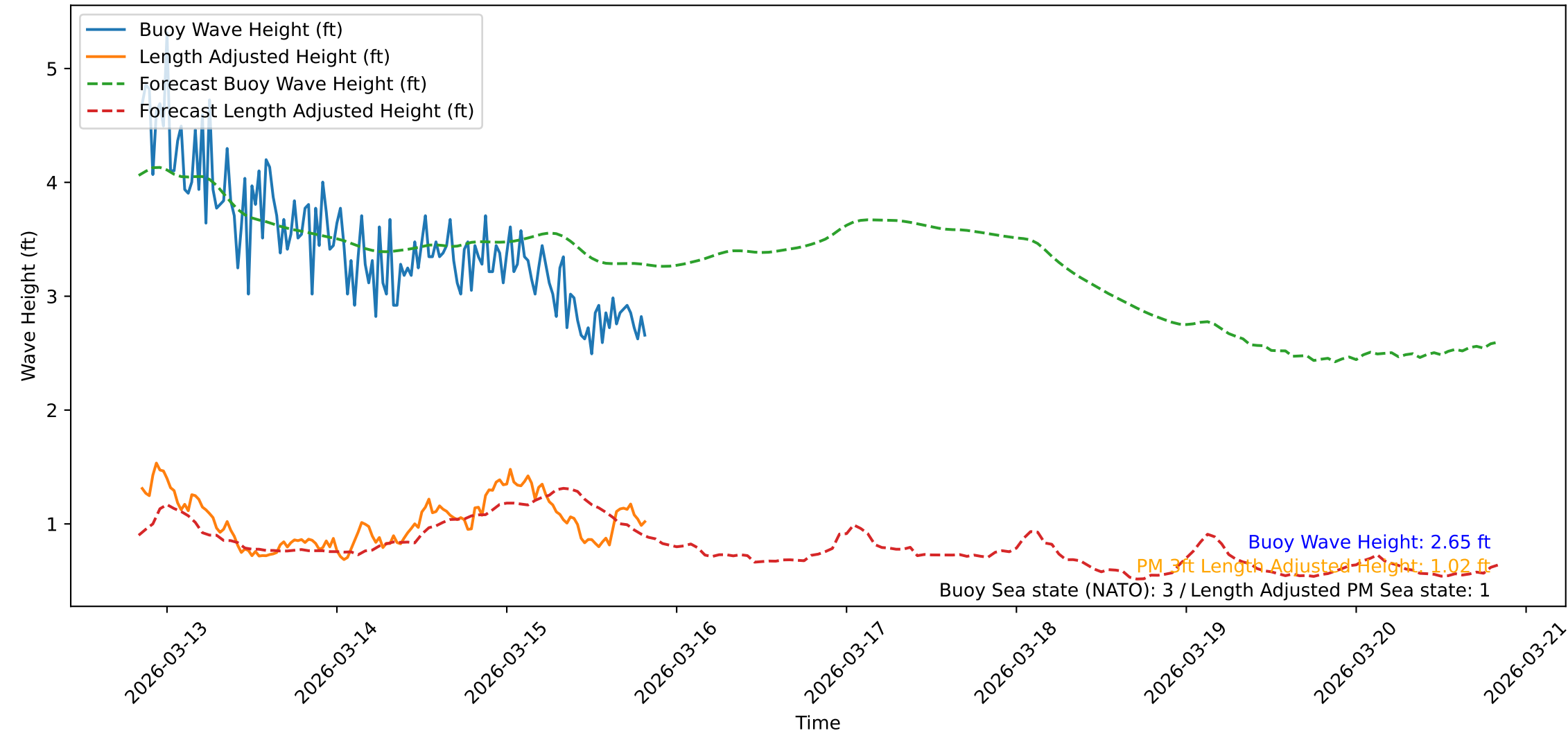
Wave Heights over Time for Oceanside Harbor at 2026-03-15 20:20:43
