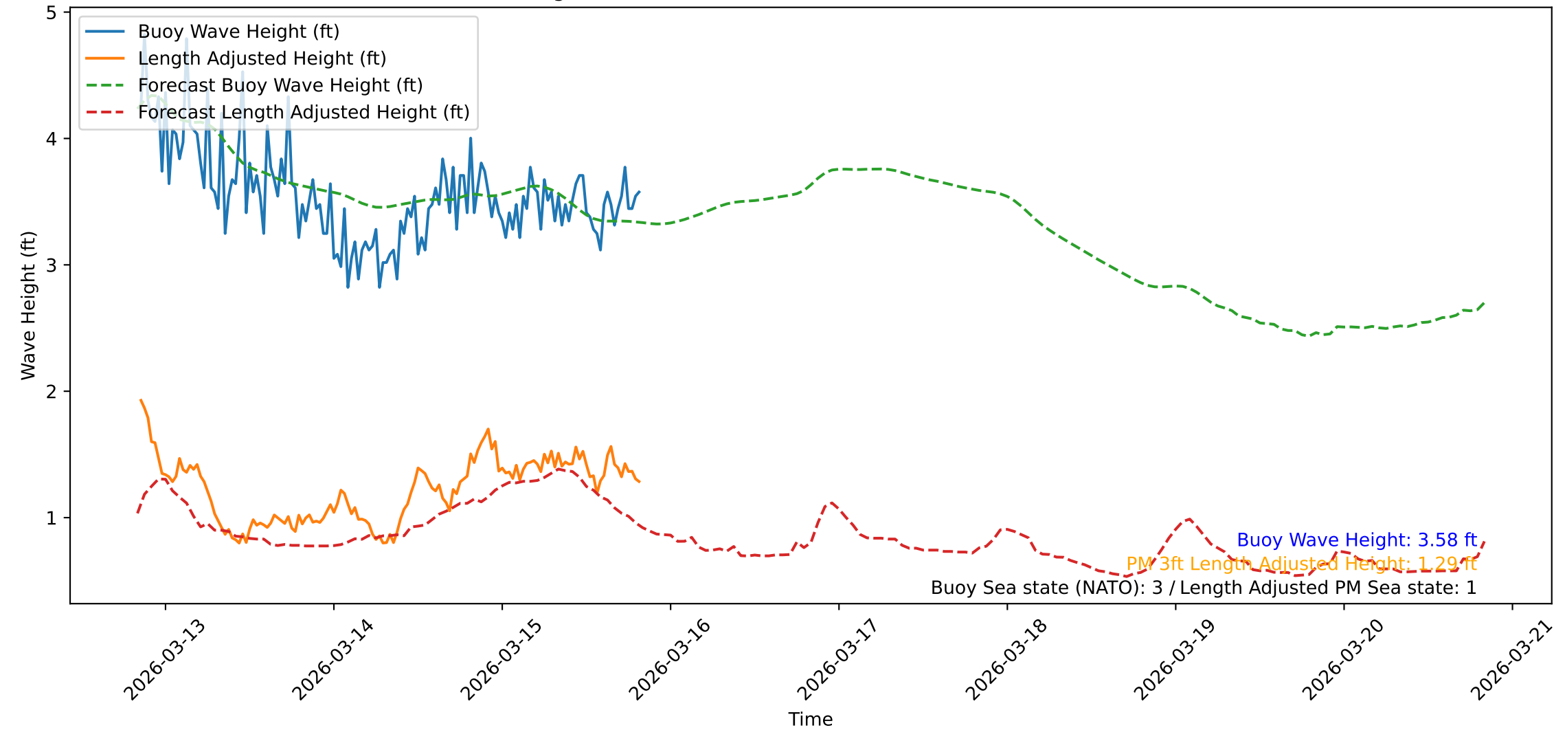
Wave Heights over Time for Green Beach at 2026-03-15 20:21:53
