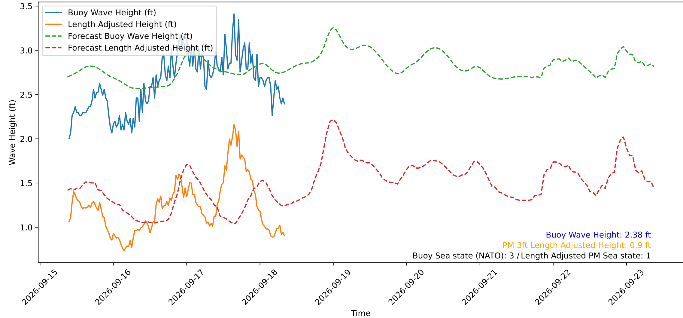
Wave Heights over Time for Red Beach at 2026-09-18 09:00:50
