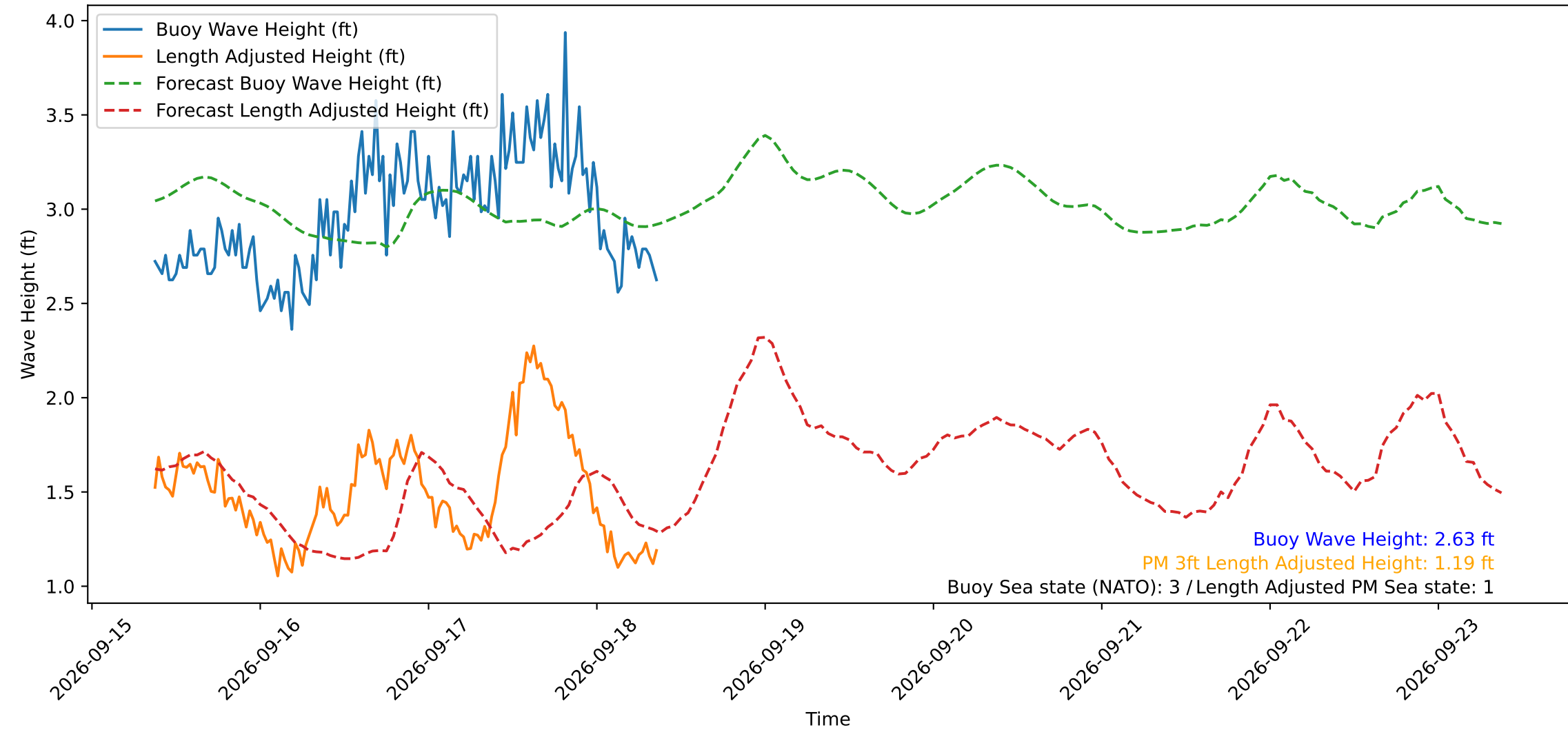
Wave Heights over Time for Oceanside Harbor at 2026-09-18 09:00:30
