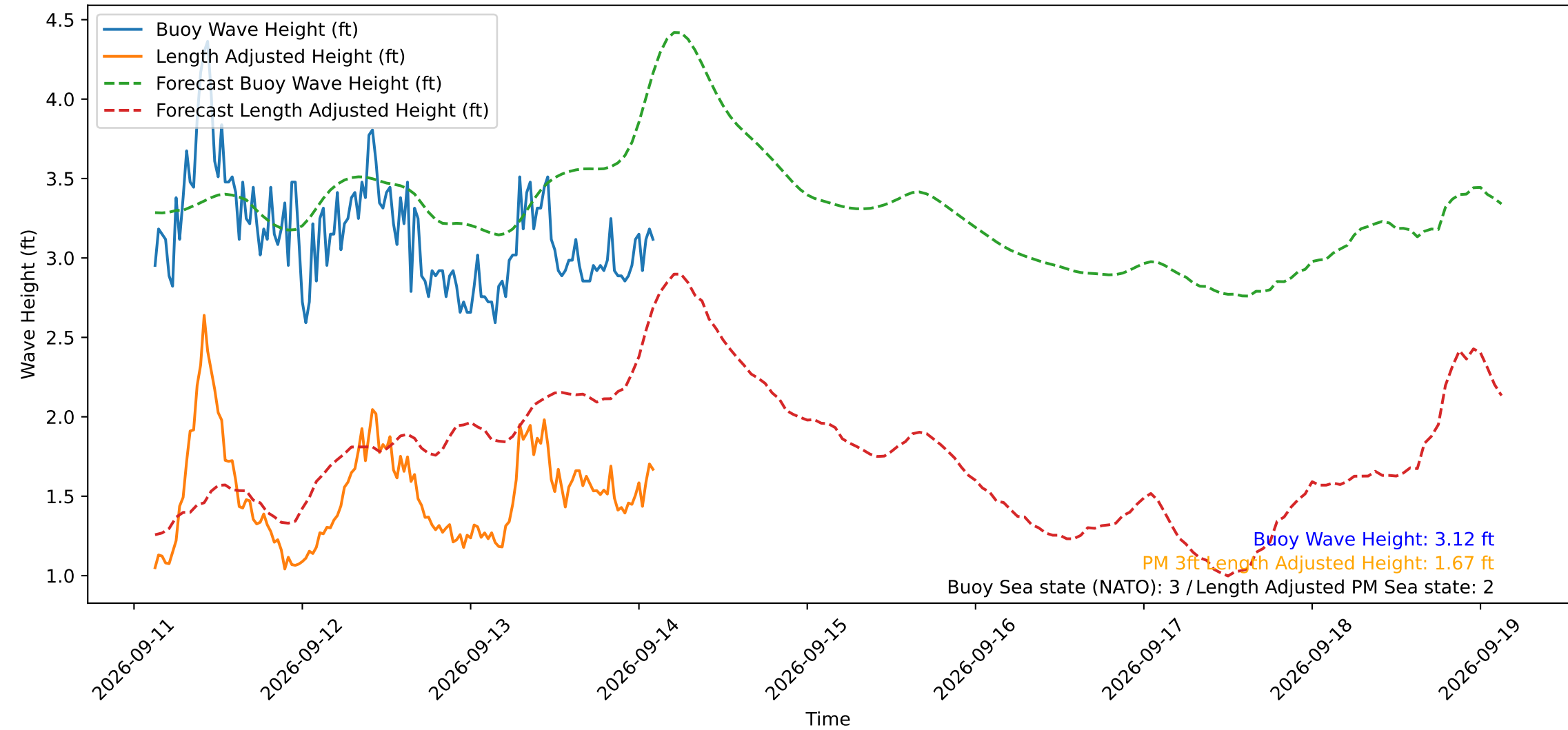
Wave Heights over Time for Oceanside Harbor at 2026-09-14 03:00:29
