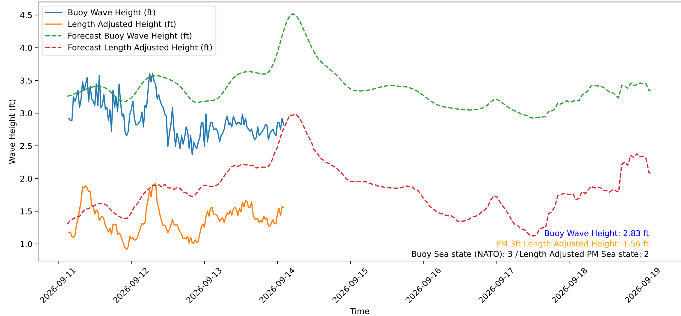
Wave Heights over Time for Green Beach at 2026-09-14 03:01:11
