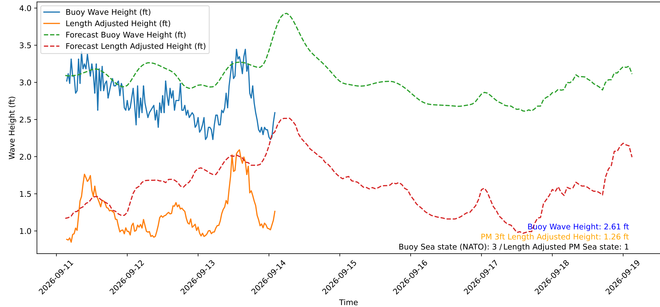
Wave Heights over Time for Red Beach at 2026-09-14 03:00:48
