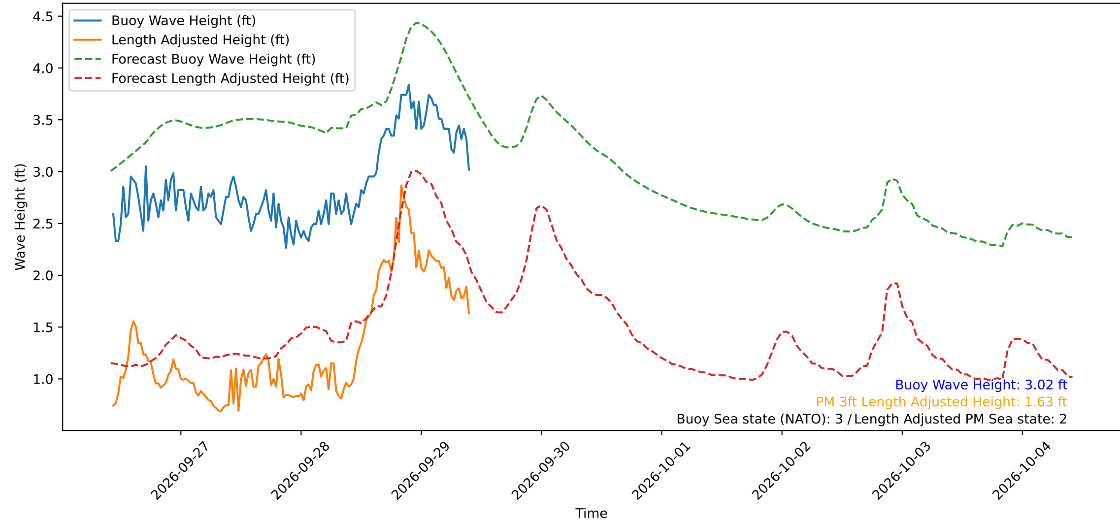
Wave Heights over Time for Red Beach at 2026-09-29 10:10:49
