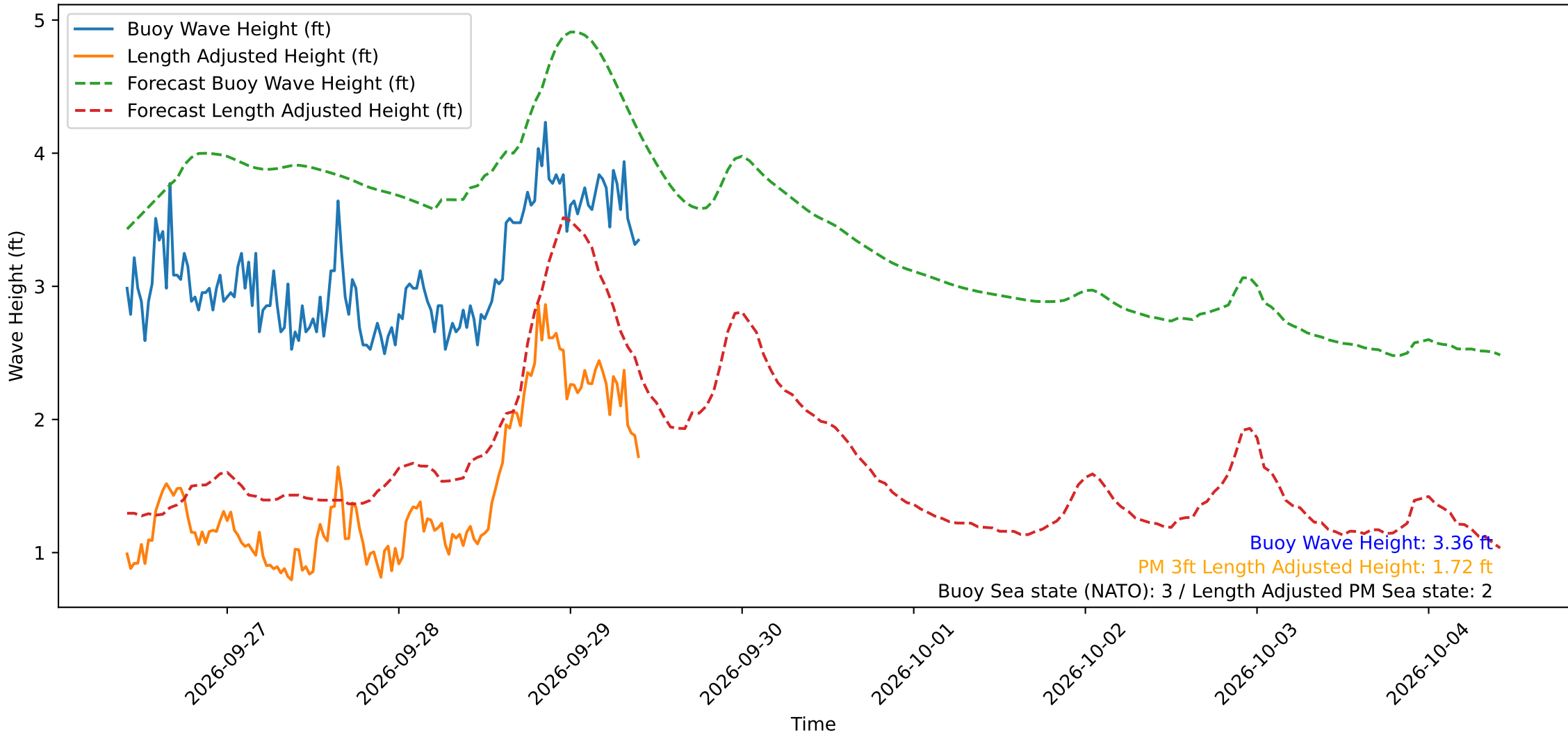
Wave Heights over Time for Oceanside Harbor at 2026-09-29 10:10:29
