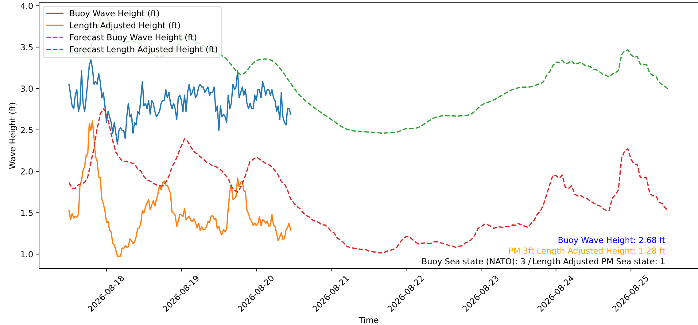
Wave Heights over Time for Red Beach at 2026-08-20 11:50:47
