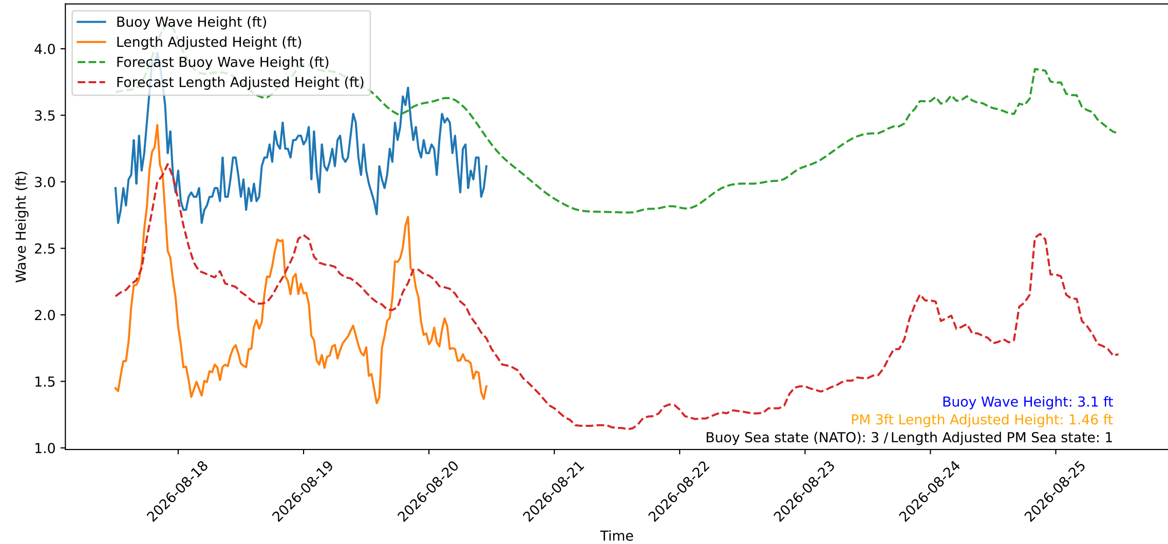
Wave Heights over Time for Green Beach at 2026-08-20 11:51:11
