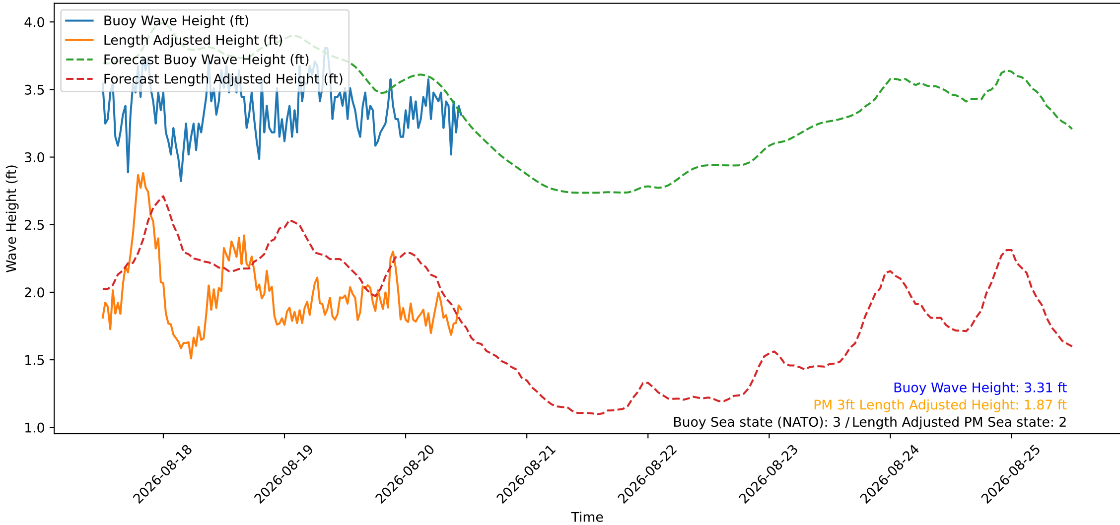
Wave Heights over Time for Oceanside Harbor at 2026-08-20 11:50:26
