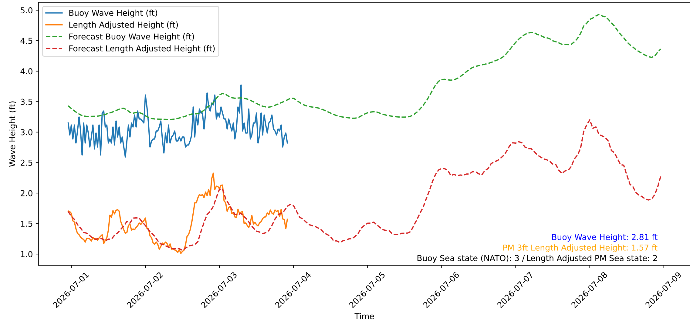
Wave Heights over Time for Oceanside Harbor at 2026-07-03 22:50:26
