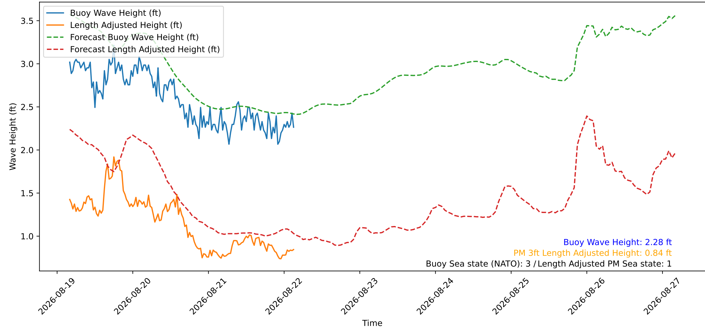
Wave Heights over Time for Red Beach at 2026-08-22 03:40:49
