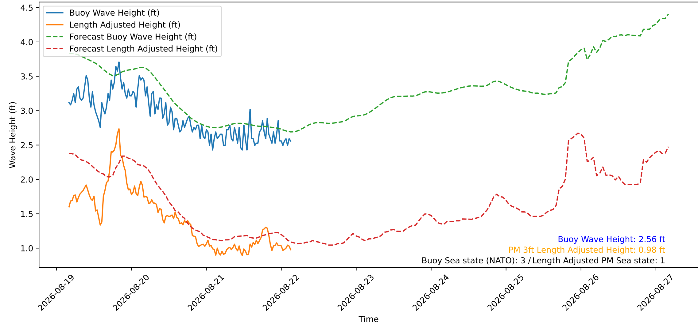
Wave Heights over Time for Green Beach at 2026-08-22 03:41:11
