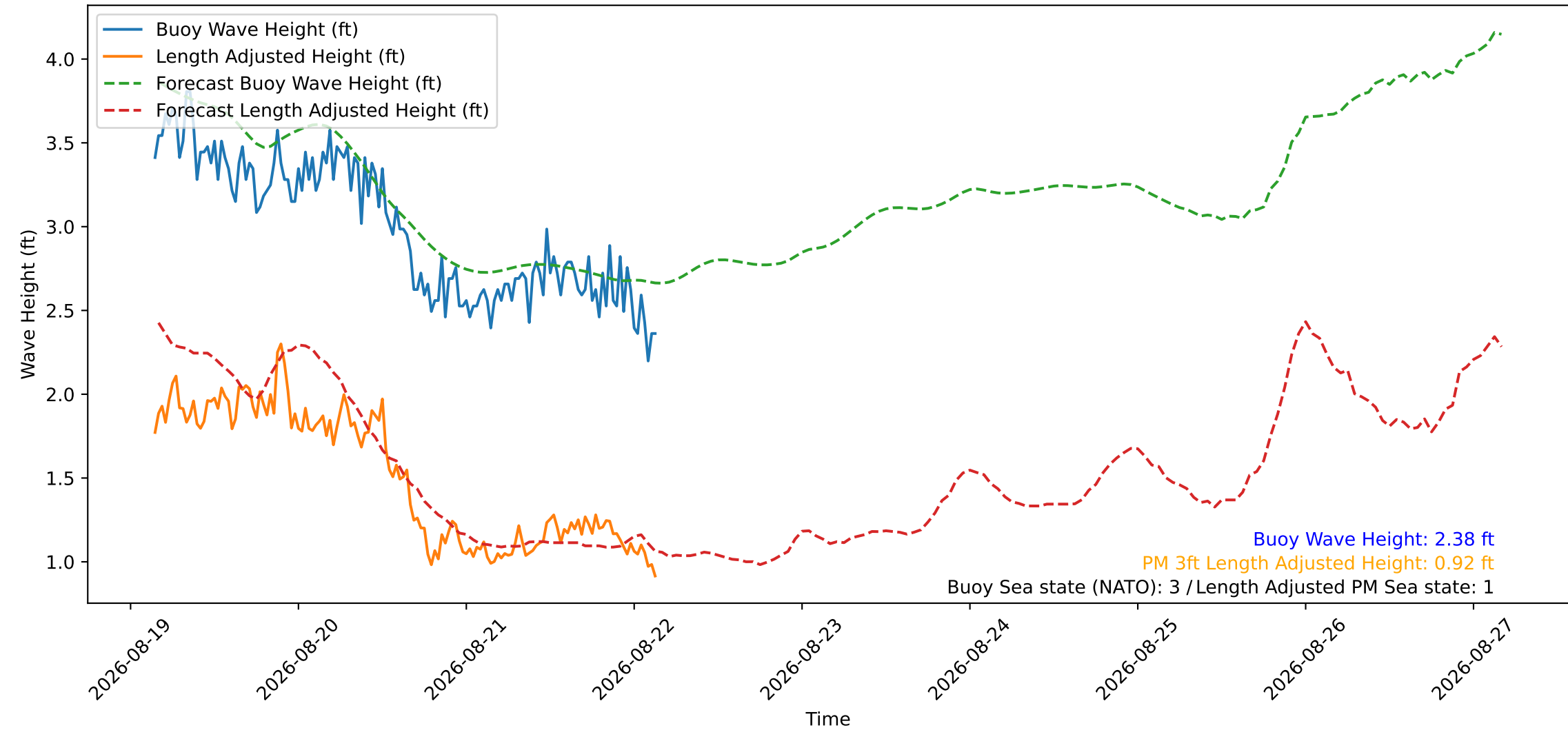
Wave Heights over Time for Oceanside Harbor at 2026-08-22 03:40:29
