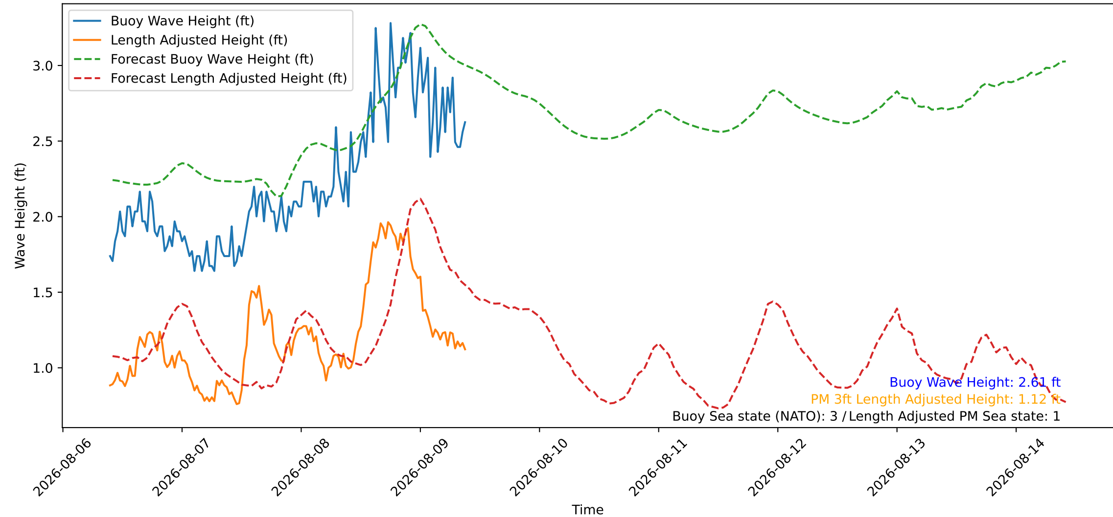
Wave Heights over Time for Oceanside Harbor at 2026-08-09 09:40:27
