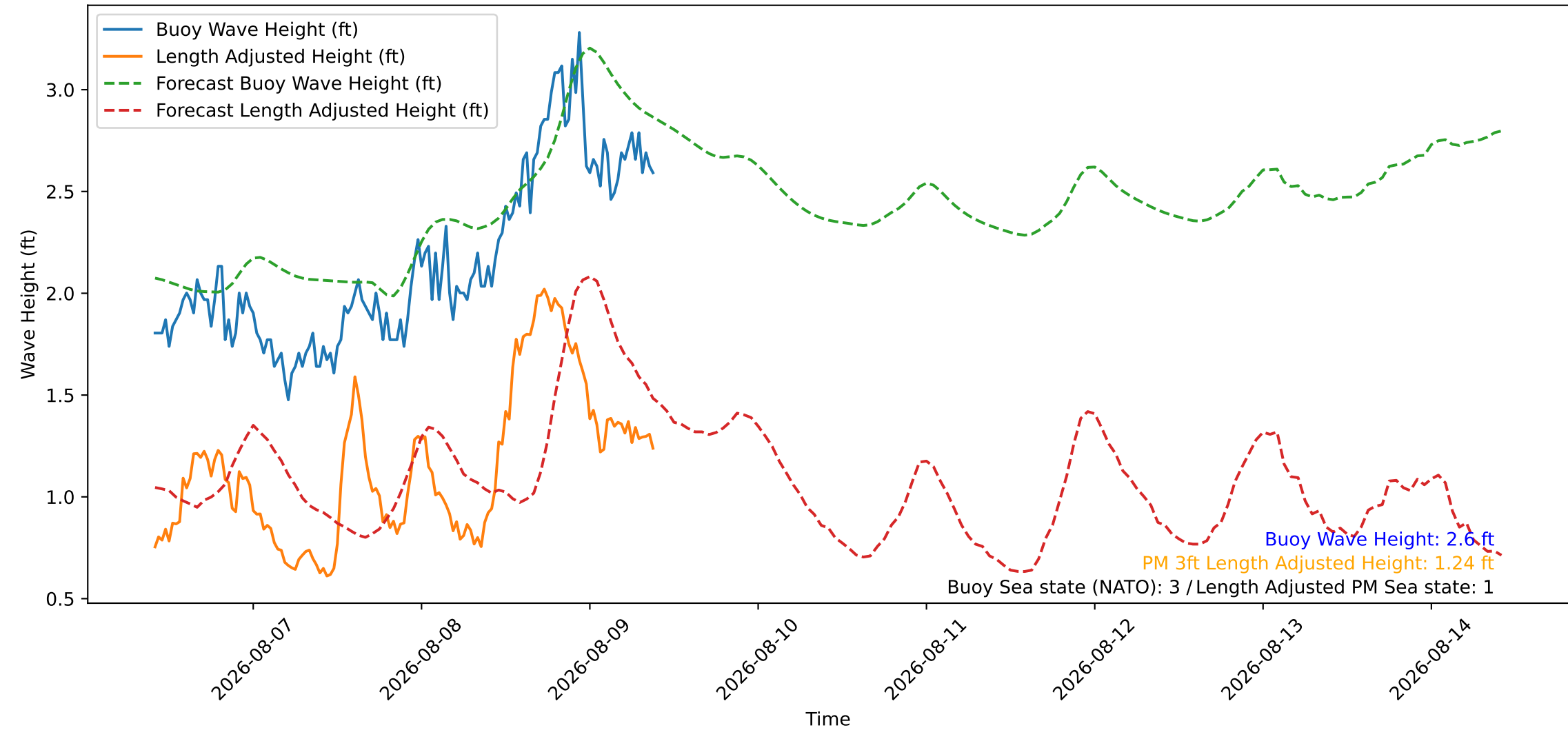
Wave Heights over Time for Red Beach at 2026-08-09 09:40:46
