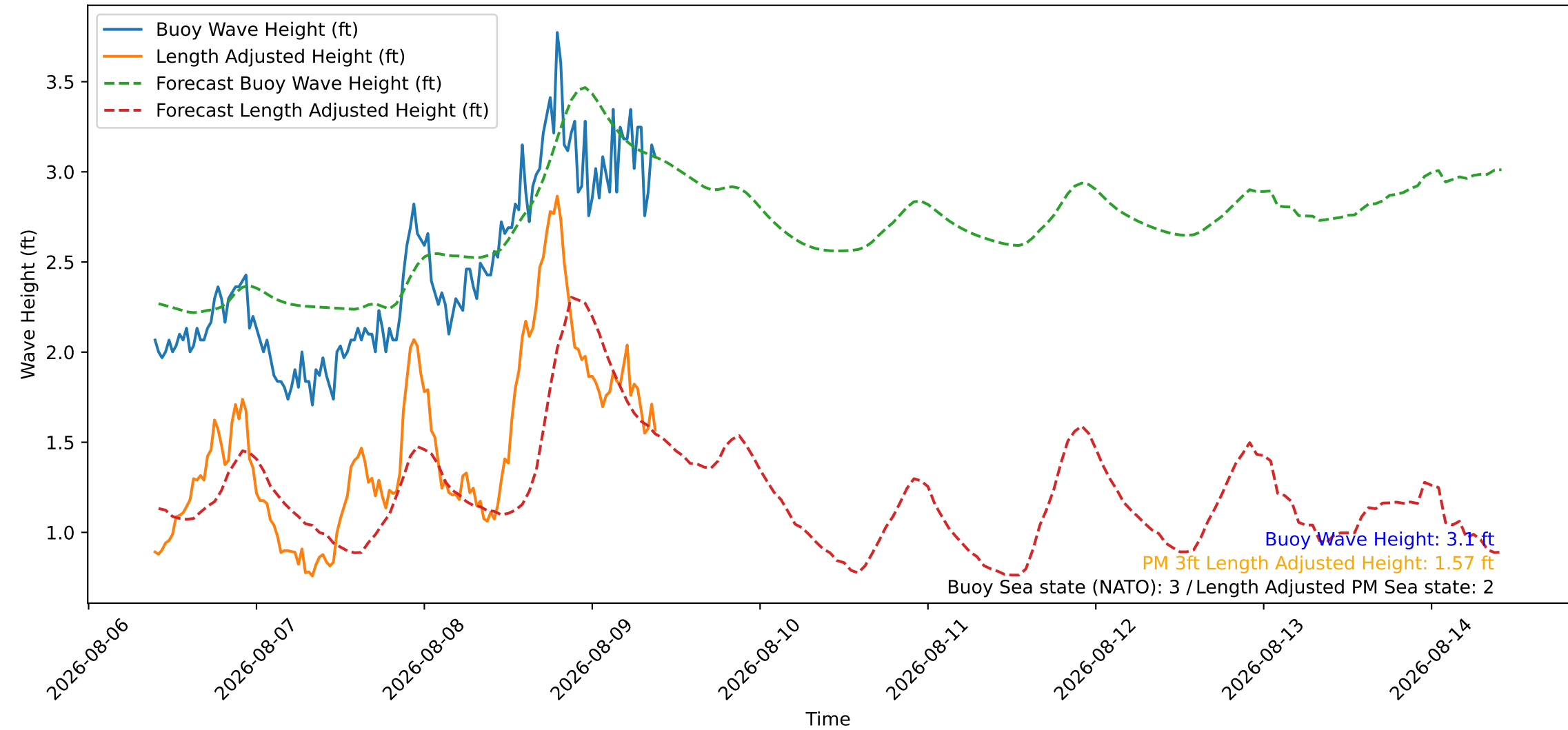
Wave Heights over Time for Green Beach at 2026-08-09 09:41:09
