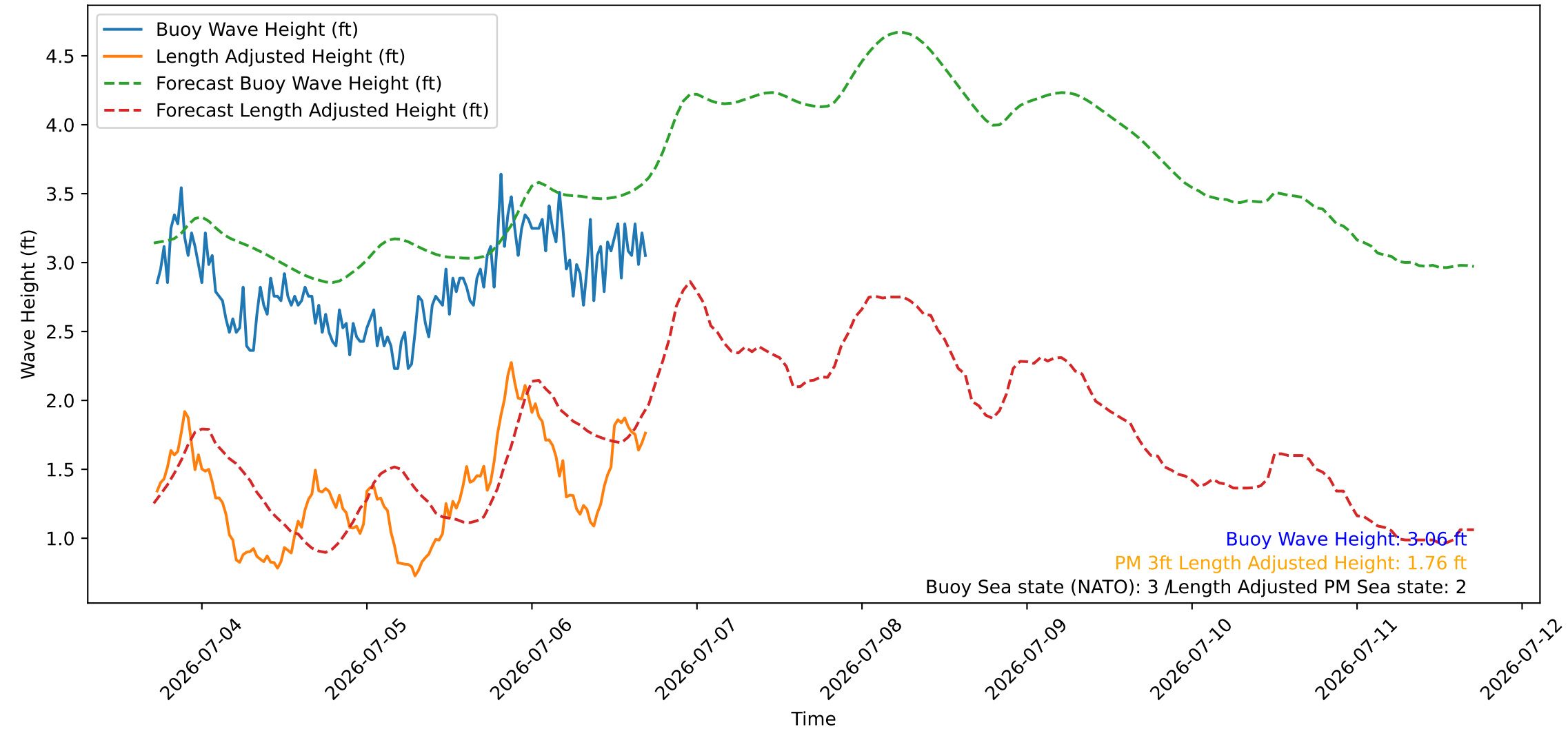
Wave Heights over Time for Red Beach at 2026-07-06 17:20:46
