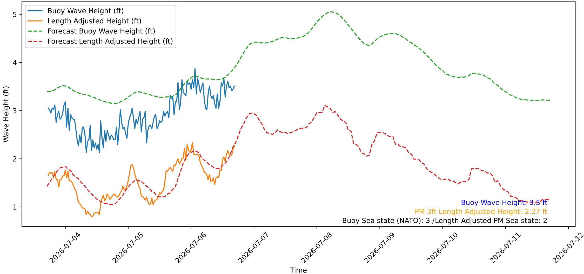
Wave Heights over Time for Oceanside Harbor at 2026-07-06 17:20:26
