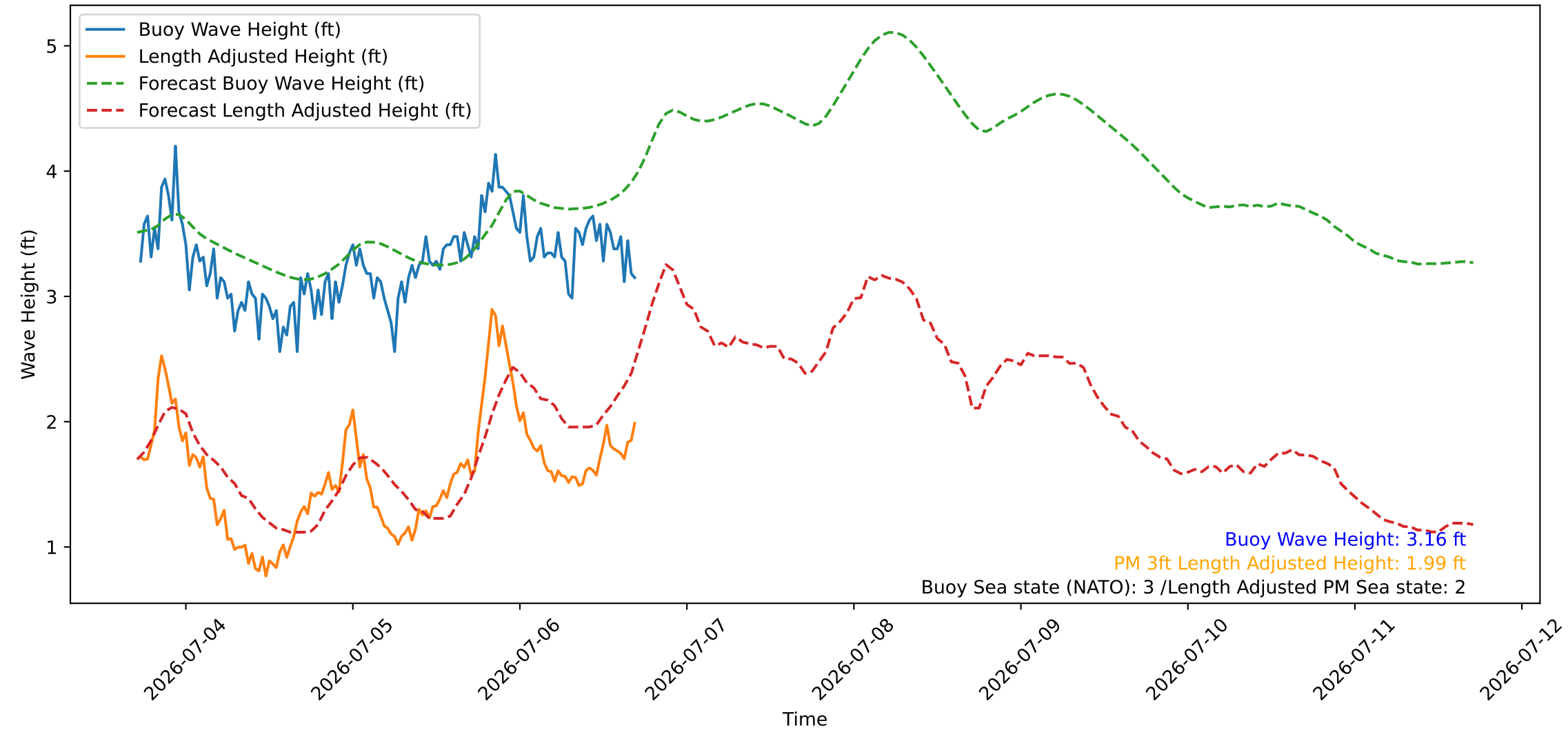
Wave Heights over Time for Green Beach at 2026-07-06 17:21:09
