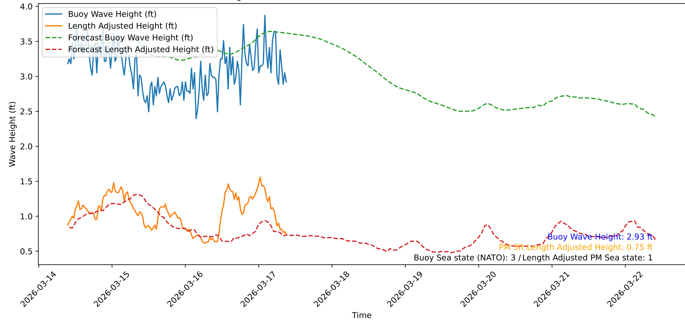
Wave Heights over Time for Oceanside Harbor at 2026-03-17 09:40:45
