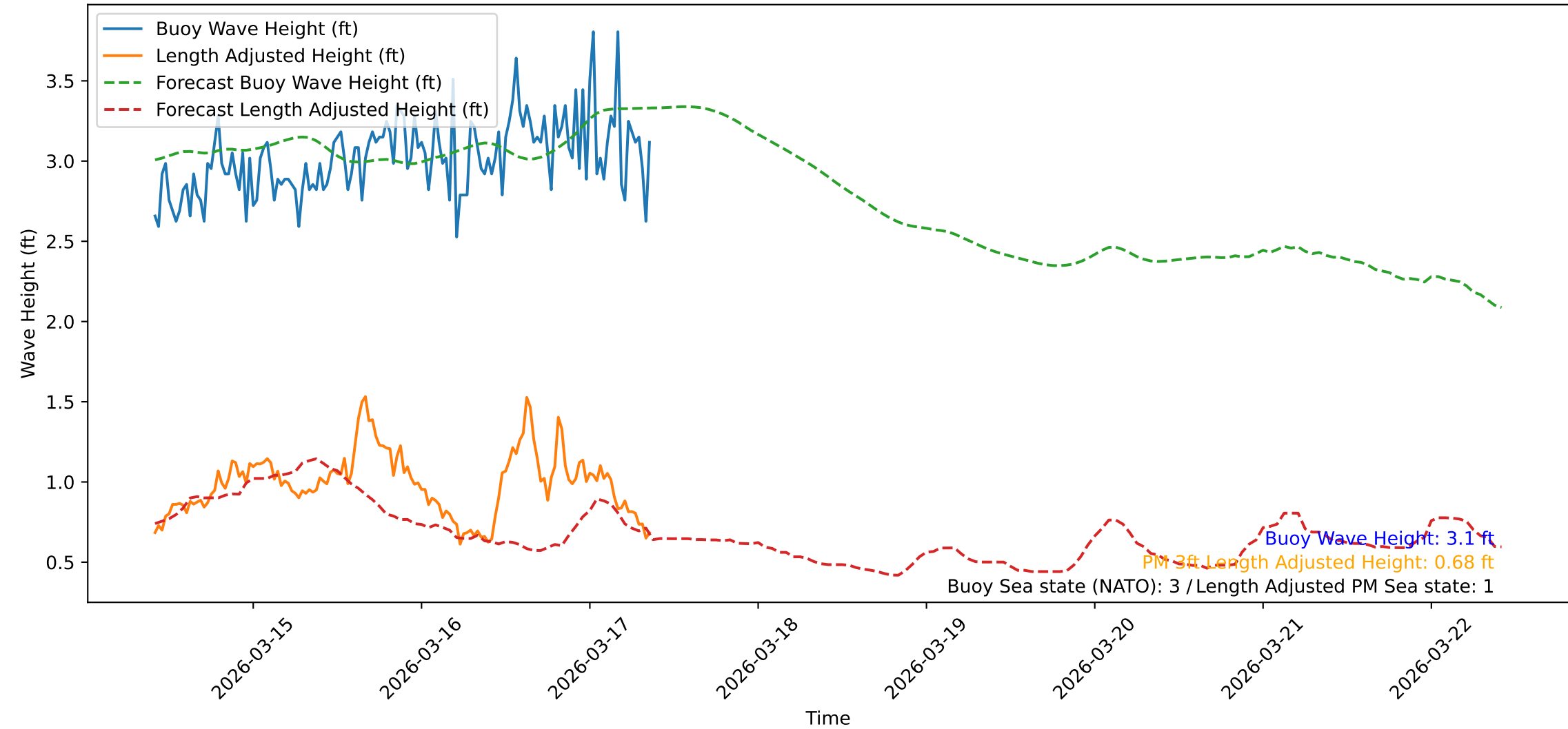
Wave Heights over Time for Red Beach at 2026-03-17 09:41:09
