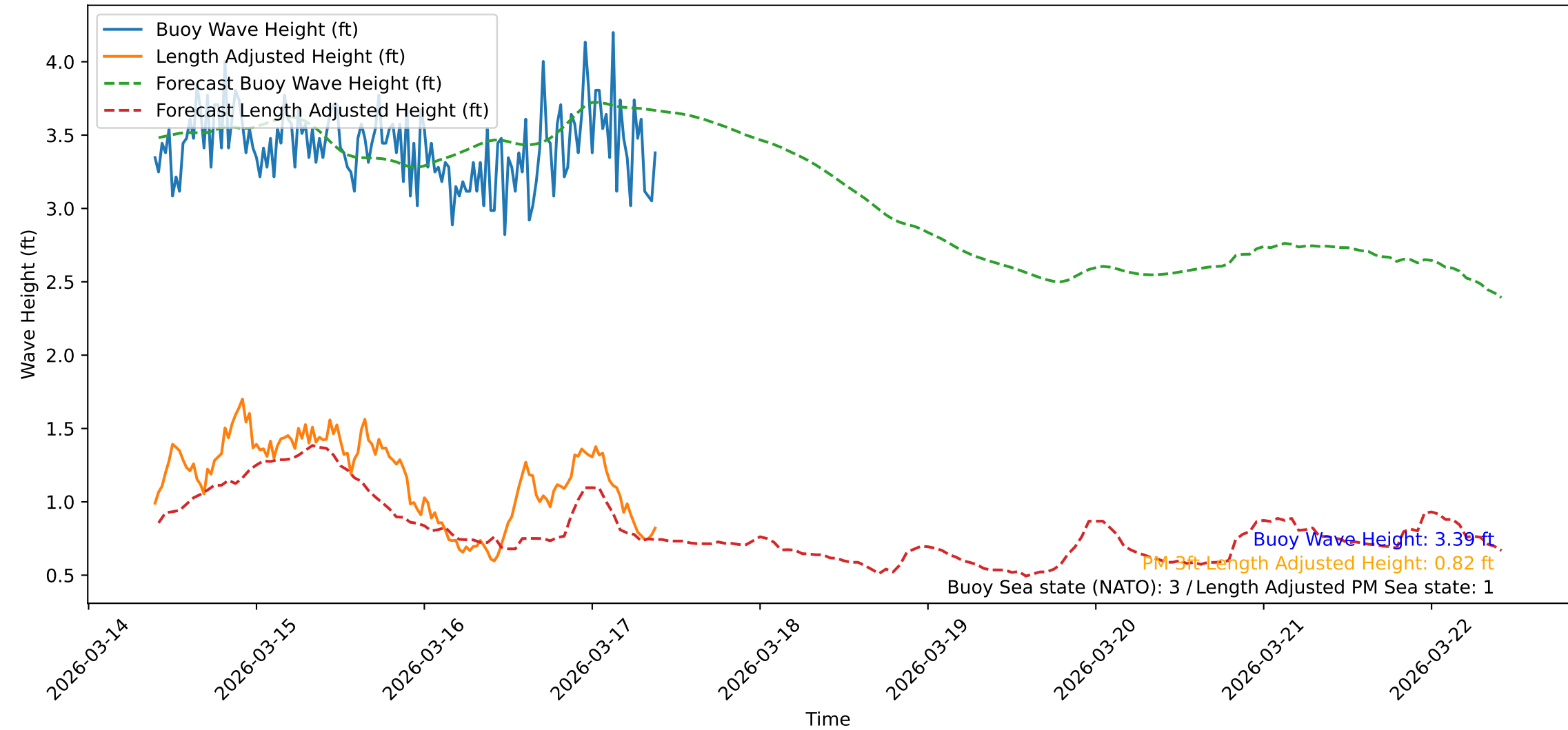
Wave Heights over Time for Green Beach at 2026-03-17 09:41:49
