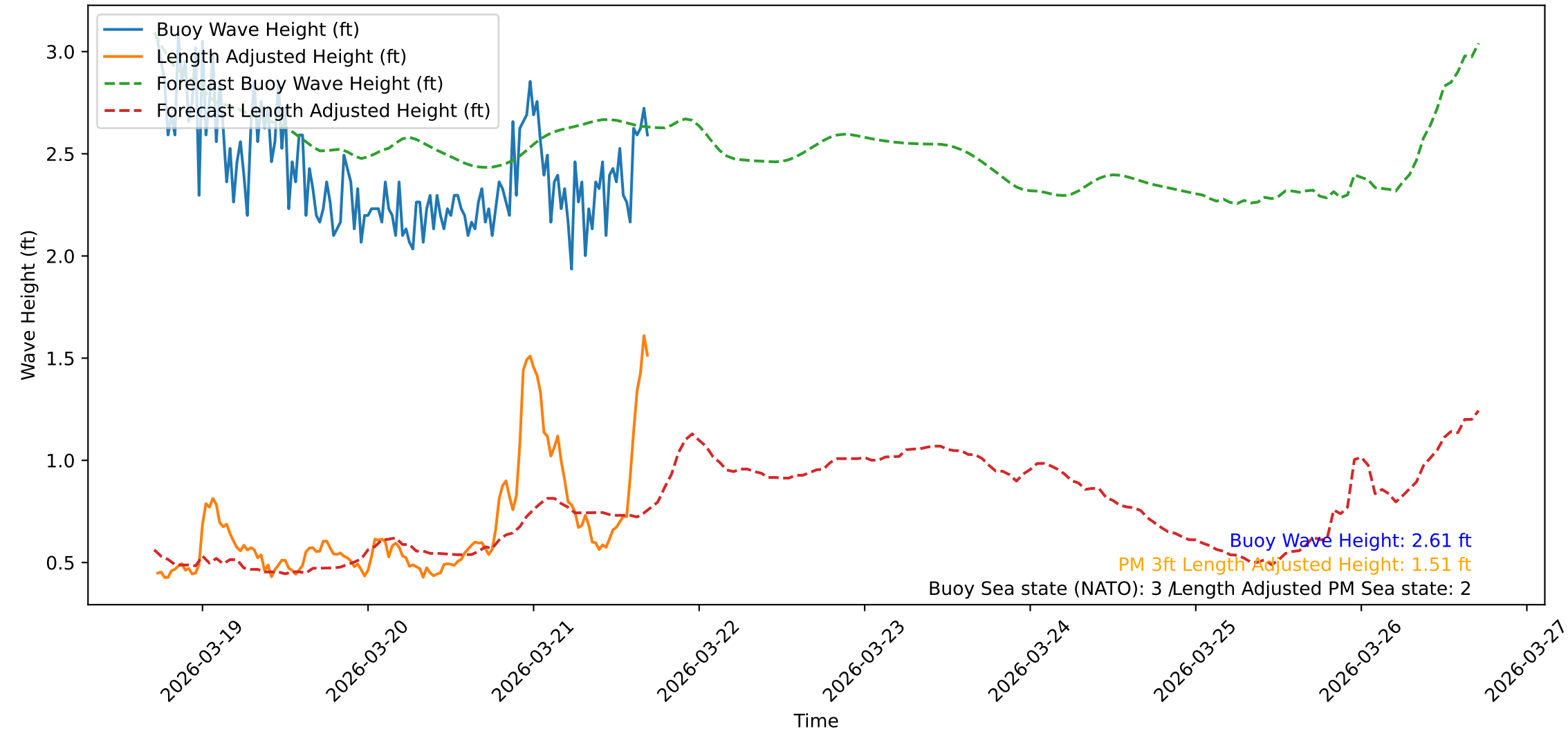
Wave Heights over Time for Green Beach at 2026-03-21 17:21:11
