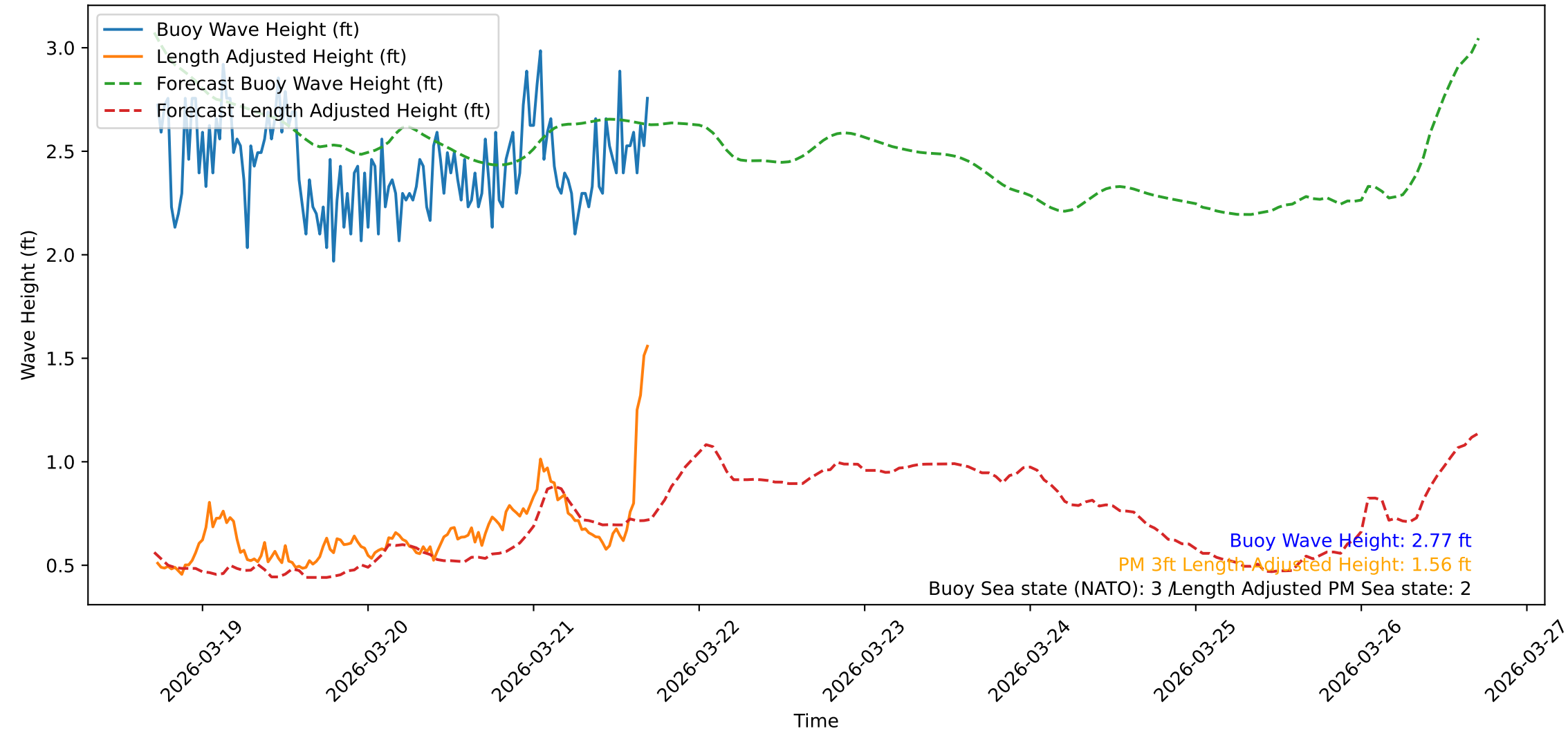
Wave Heights over Time for Oceanside Harbor at 2026-03-21 17:20:32
