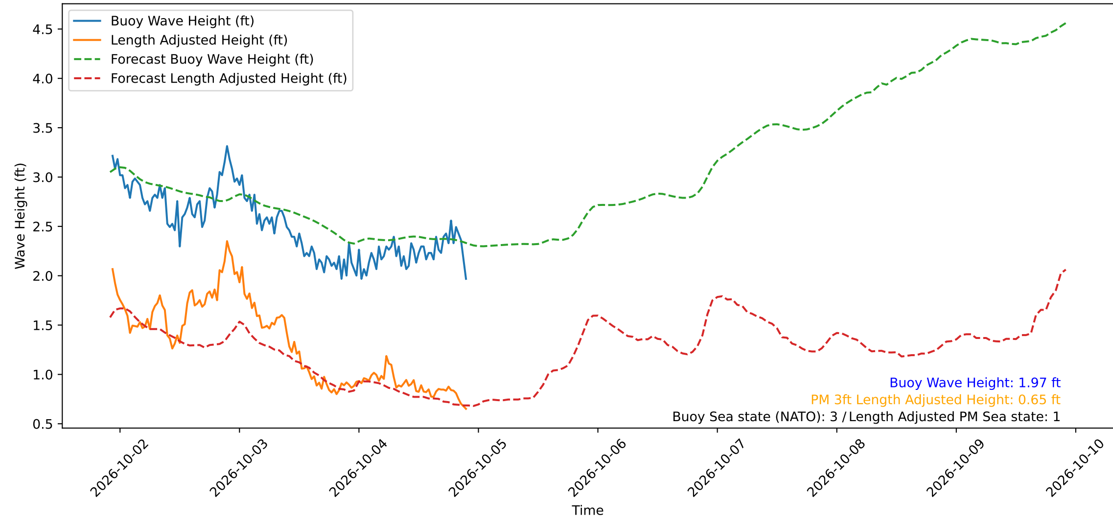
Wave Heights over Time for Oceanside Harbor at 2026-10-04 22:20:30
