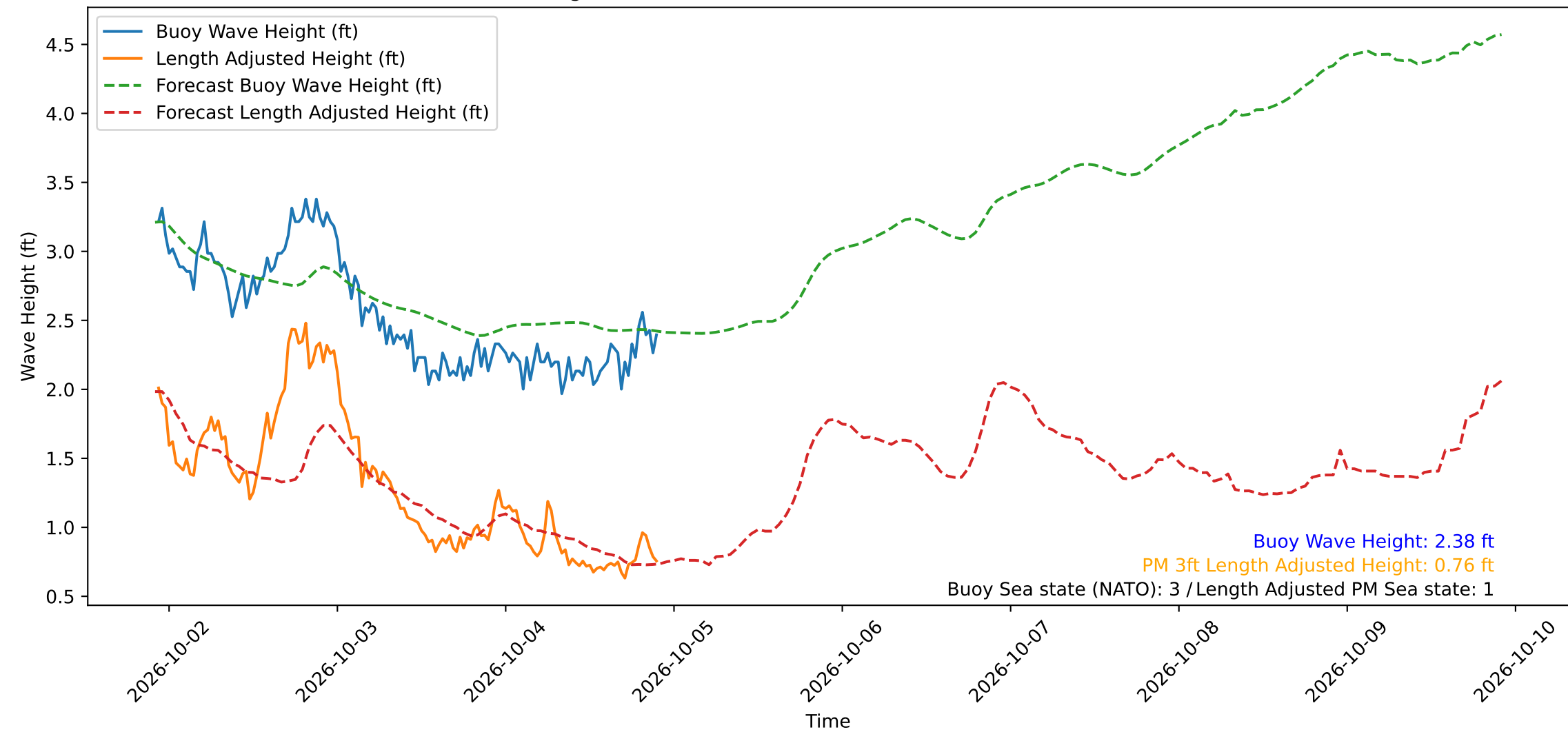
Wave Heights over Time for Green Beach at 2026-10-04 22:21:14
