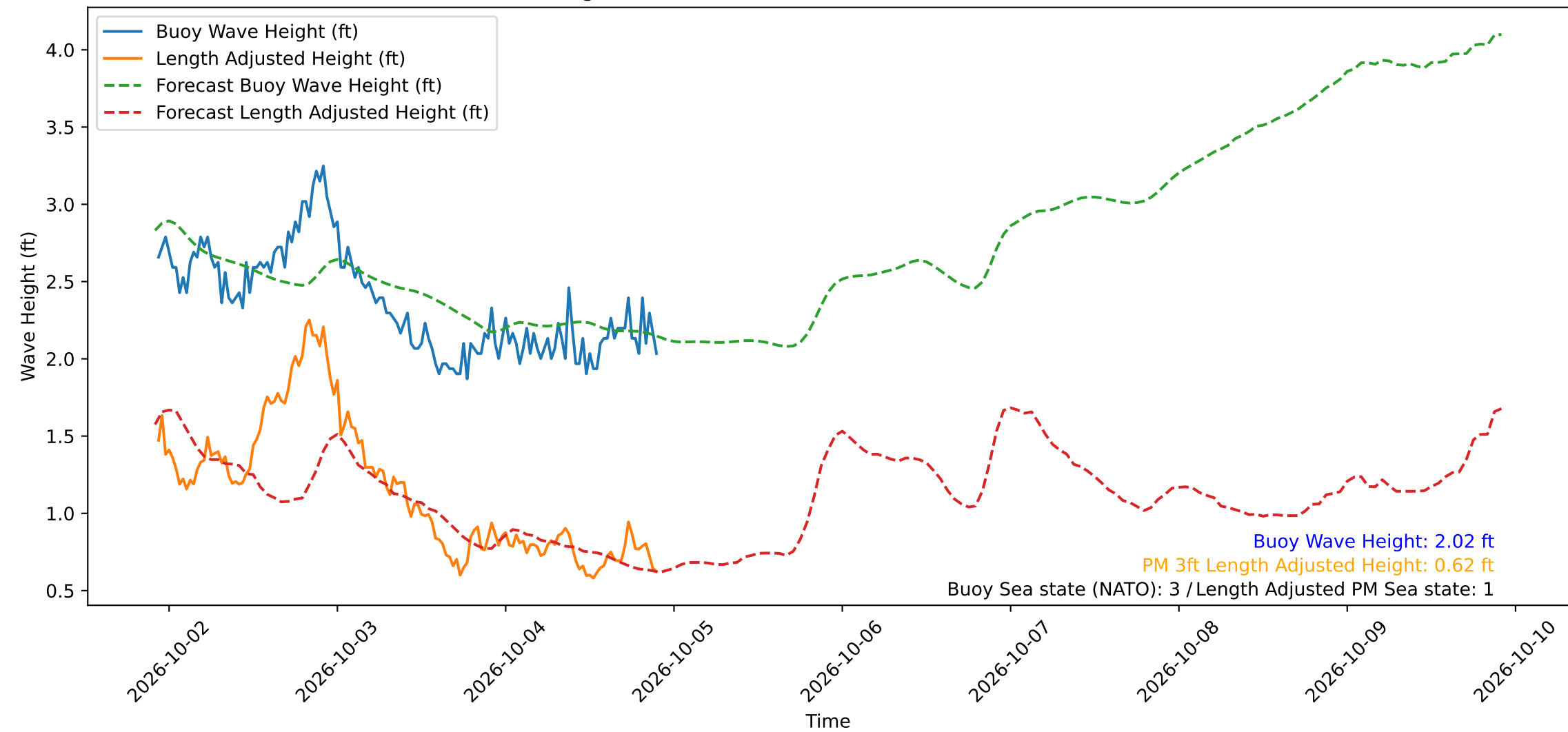
Wave Heights over Time for Red Beach at 2026-10-04 22:20:50
