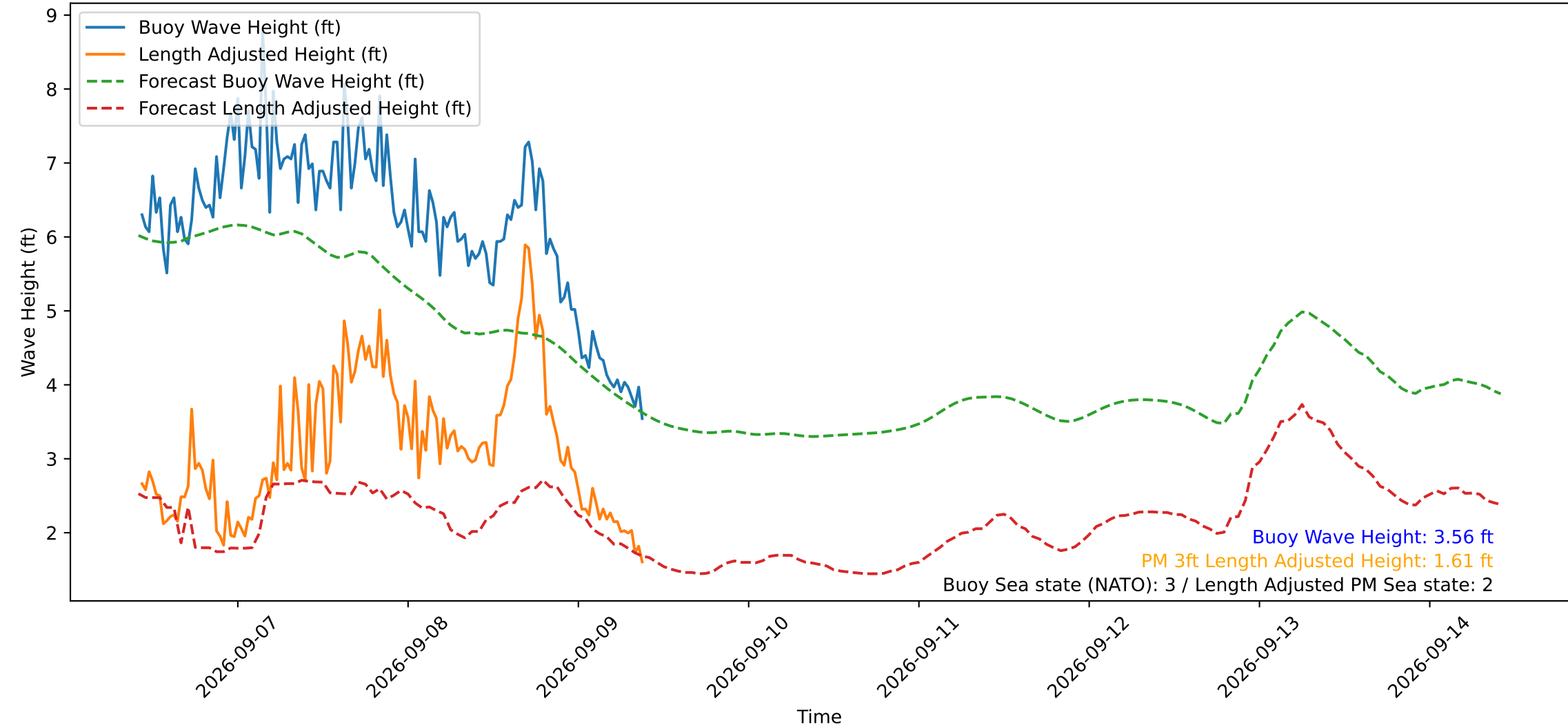
Wave Heights over Time for Green Beach at 2026-09-09 10:01:12
