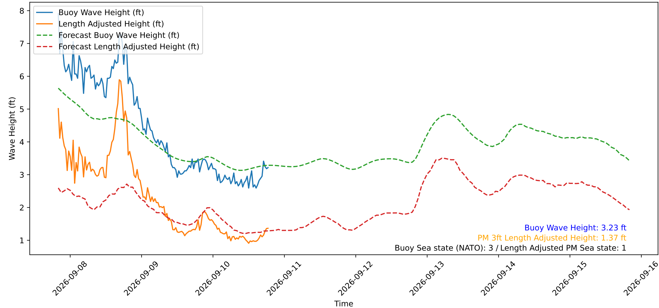
Wave Heights over Time for Green Beach at 2026-09-10 19:31:12
