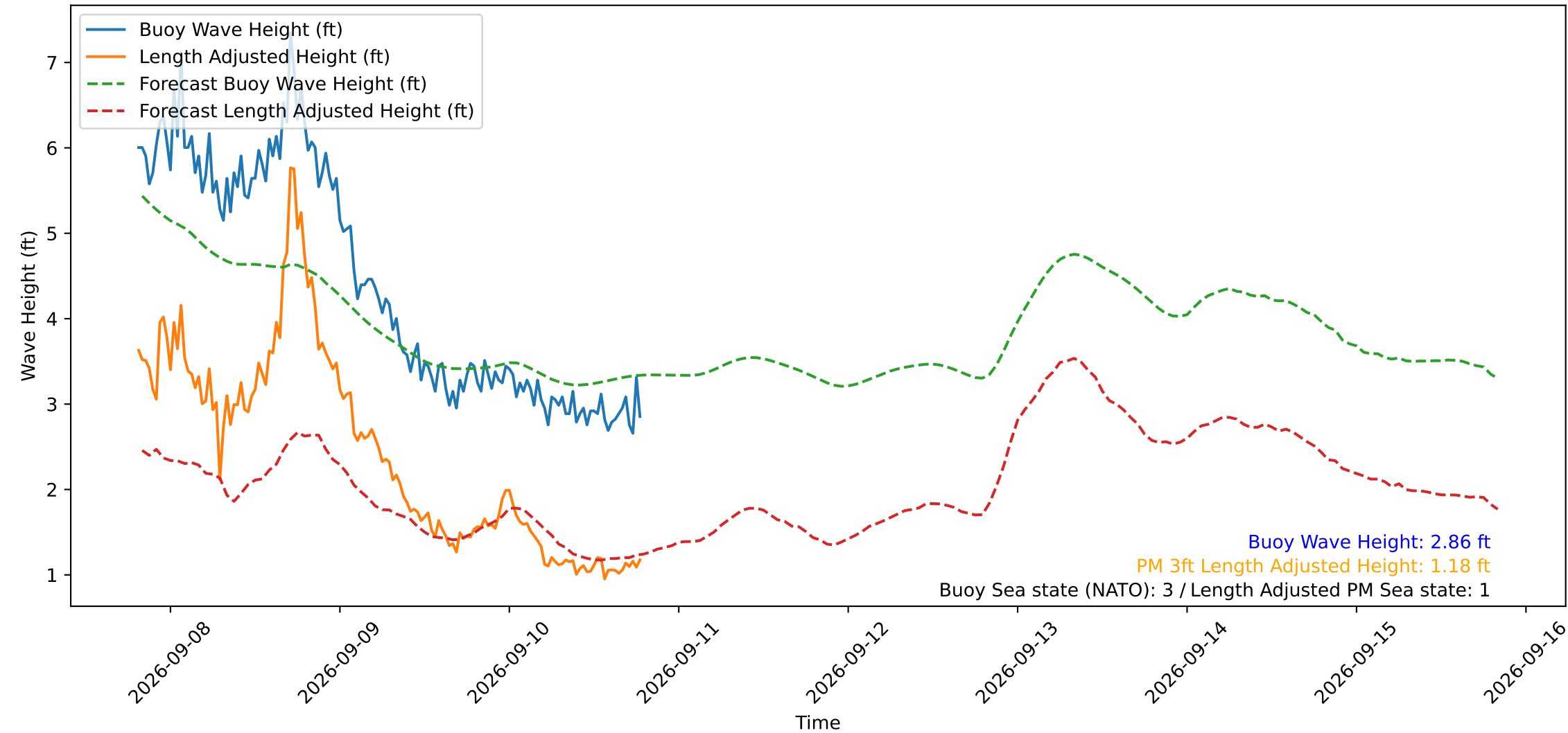
Wave Heights over Time for Oceanside Harbor at 2026-09-10 19:30:30
