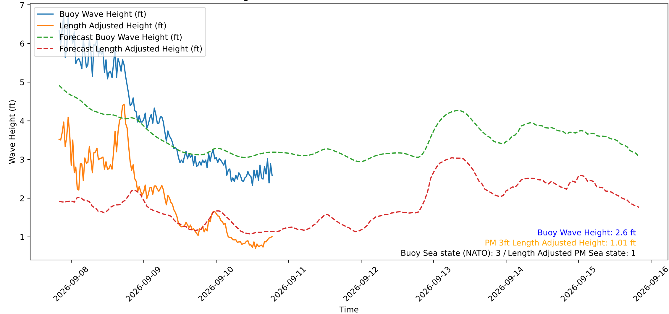
Wave Heights over Time for Red Beach at 2026-09-10 19:30:49
