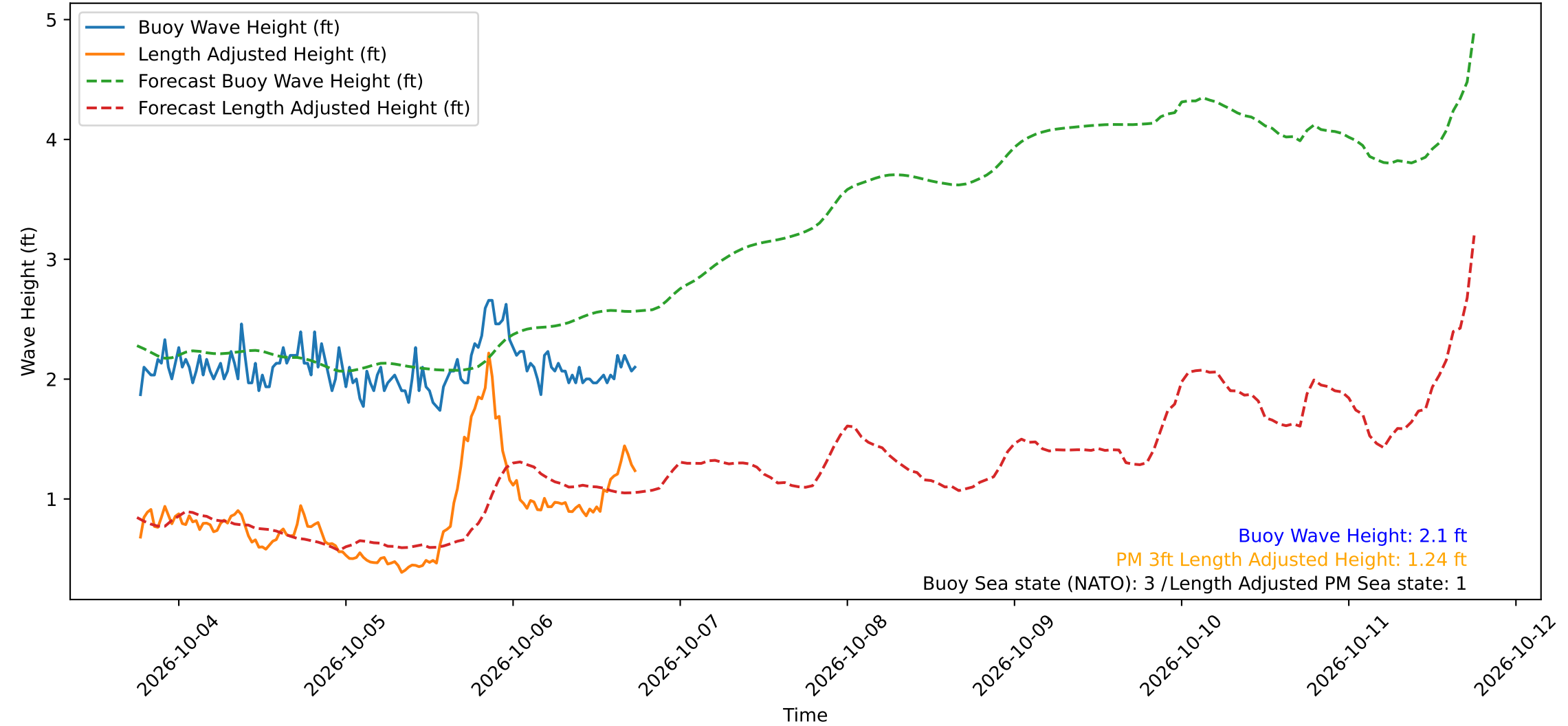
Wave Heights over Time for Red Beach at 2026-10-06 18:20:51
