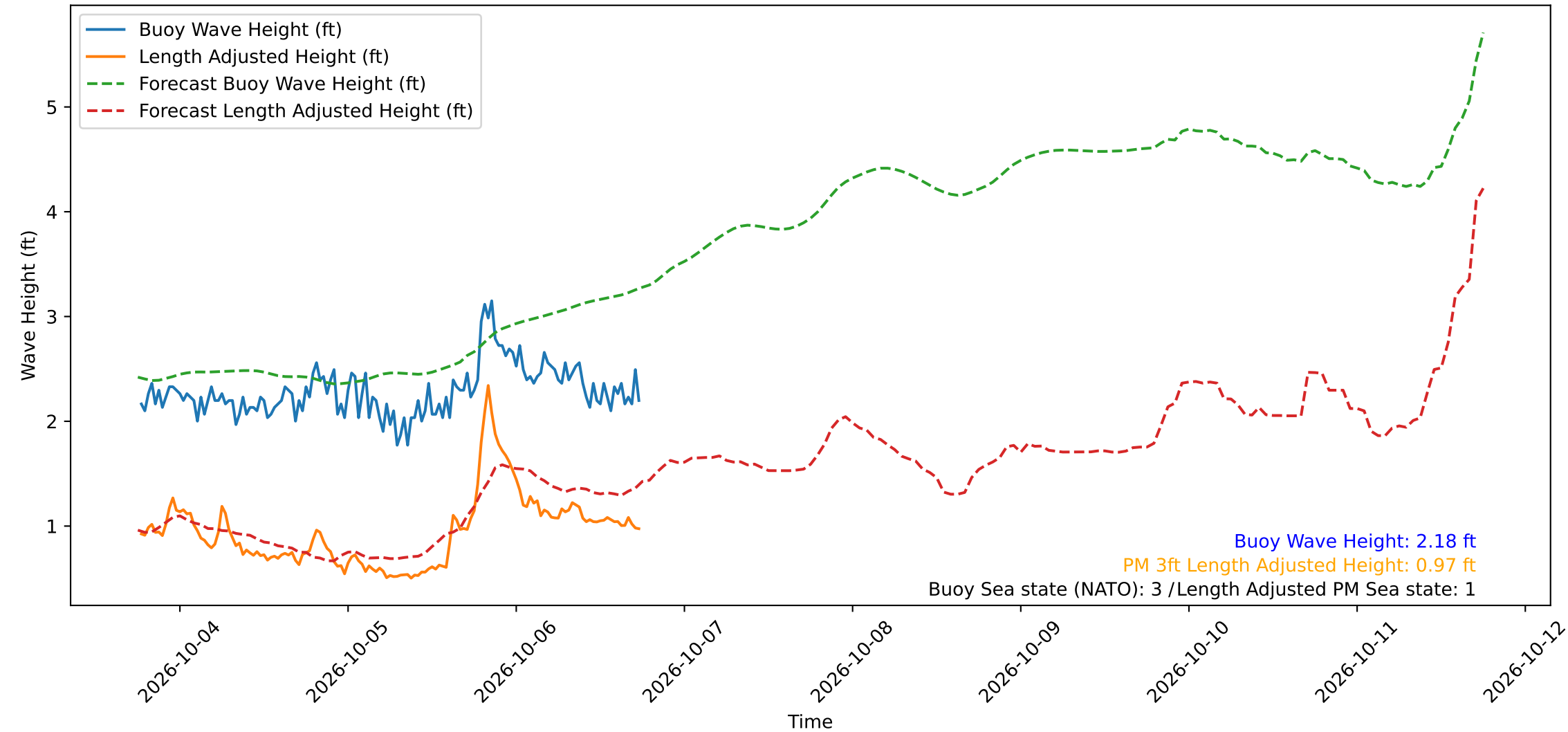
Wave Heights over Time for Green Beach at 2026-10-06 18:21:15
