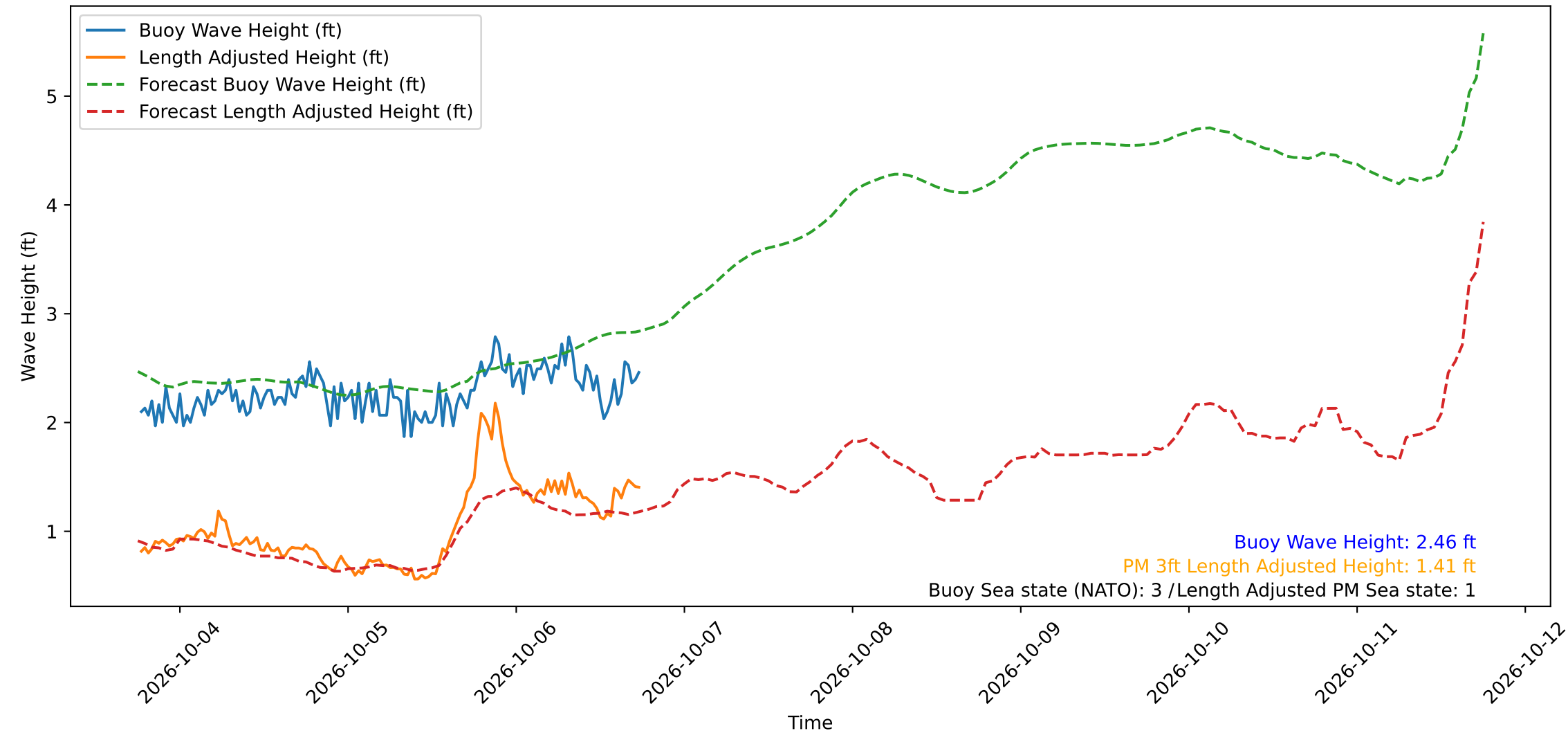
Wave Heights over Time for Oceanside Harbor at 2026-10-06 18:20:30
