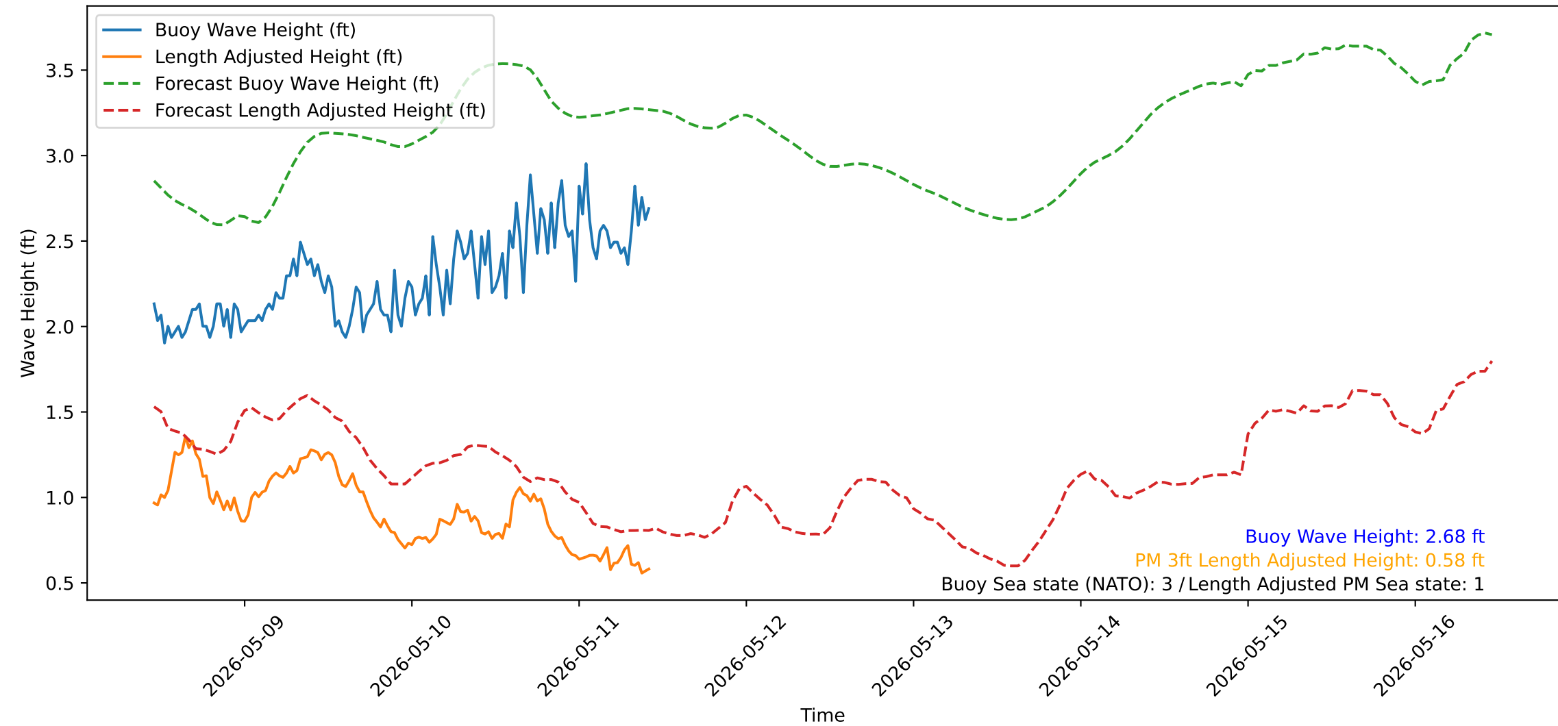
Wave Heights over Time for Red Beach at 2026-05-11 10:50:52
