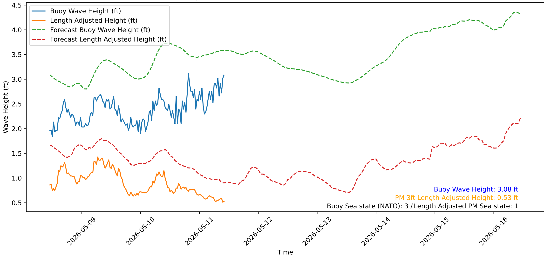
Wave Heights over Time for Green Beach at 2026-05-11 10:51:15
