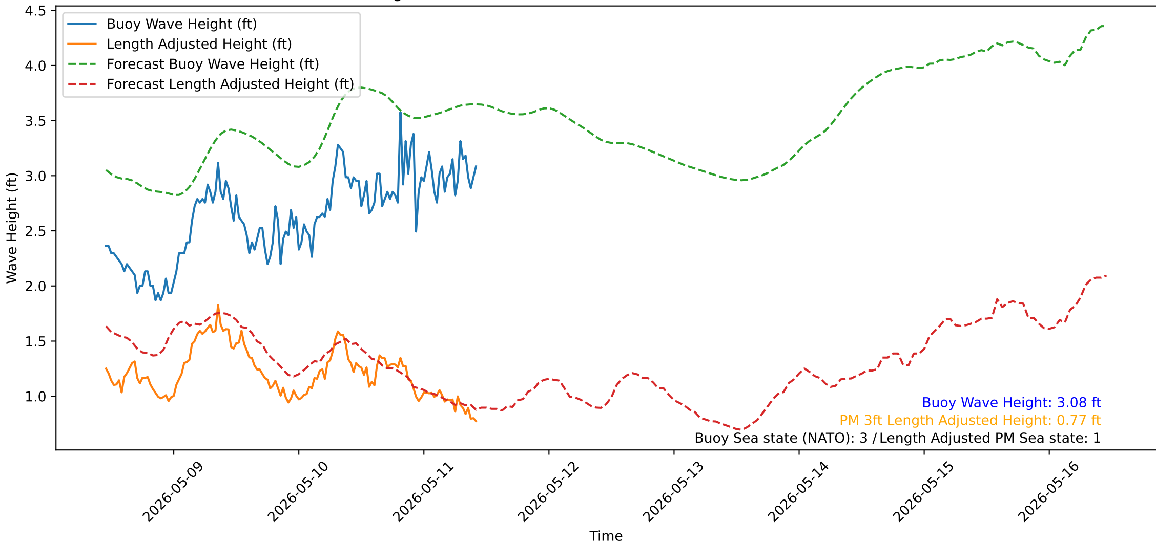
Wave Heights over Time for Oceanside Harbor at 2026-05-11 10:50:31
