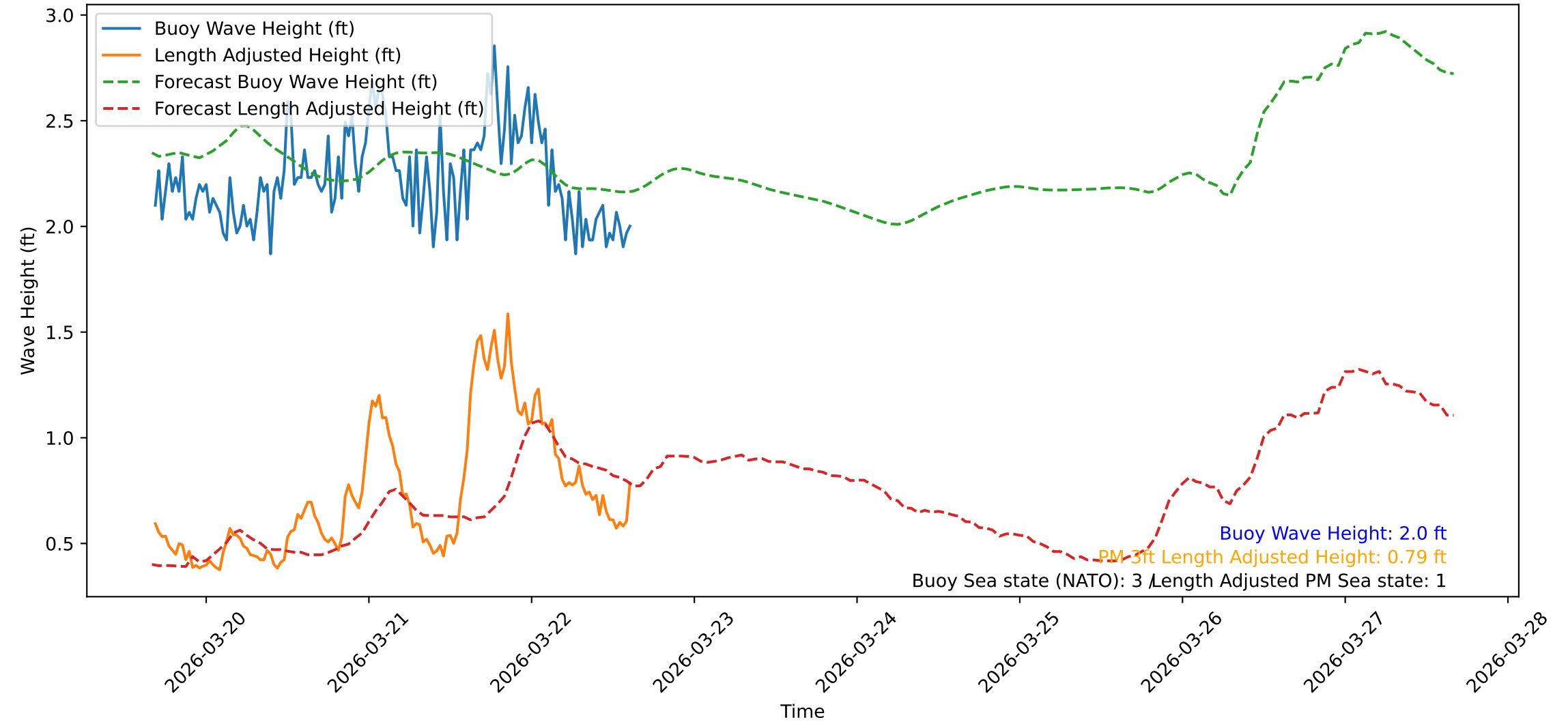
Wave Heights over Time for Red Beach at 2026-03-22 16:20:47
