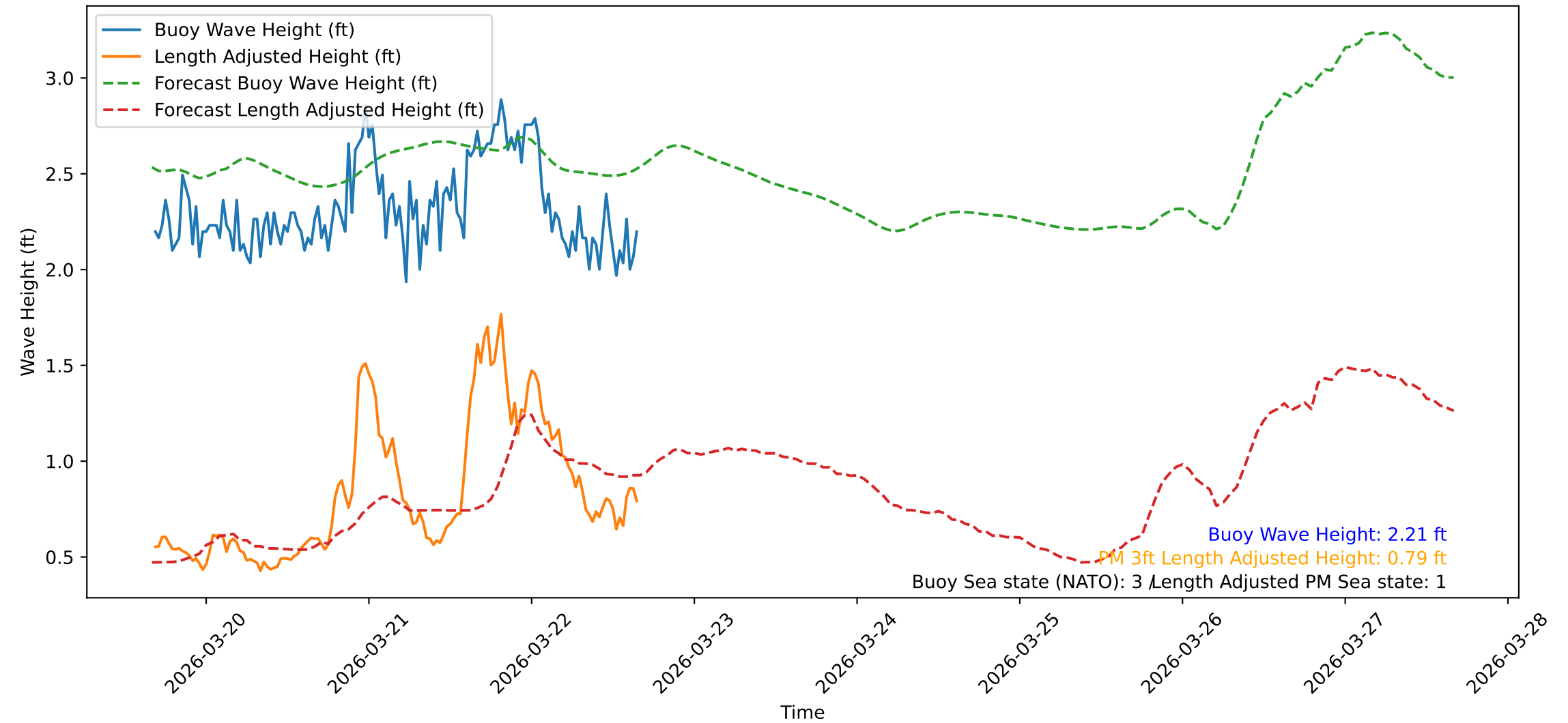
Wave Heights over Time for Green Beach at 2026-03-22 16:21:09
